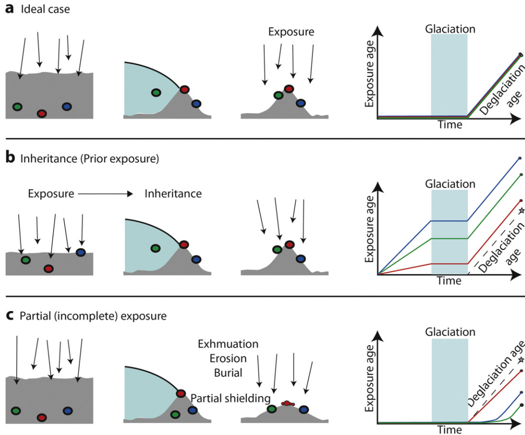
Fig. 3. Potential scenarios to be considered when using TCN dating from Heyman et al. (2011). a) The sample has been completely shielded from cosmic rays prior to glacialiation and continuously exposed since deglaciation. b) Sample is exposed to cosmic rays prior to glacialiation and experiences no post-glacial shielding (prior exposure) the apparent exposure age will exceed the deglaciation age. c) Sample is completely shielded from cosmic rays prior to glacialiation and partially shielded from cosmic rays following deglaciation (incomplete exposure) the apparent exposure age will be younger than the deglaciation age.
