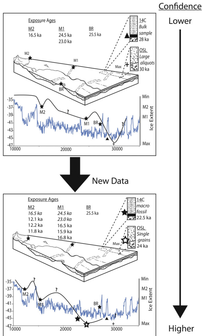
Fig. 2. A hypothetical deglaciation sequence initially populated with ages that are taken at face value to reconstruct changes in ice extent in a palaeoclimatic context using the NGRIP \delta^{18}\text{O} record (Rasmussen et al., 2006). Addition of new data fundamentally changes the interpretation of the relationship between changes in ice extent and climate. In this hypothetical example the large aliquot OSL age is several ka older than the age obtained using the single grain approach (e.g. Duller, 2006, 2008). The bulk radiocarbon age is older than the radiocarbon age obtained from a macrofossil in the same horizon (e.g. Grimm et al., 2009). The TCN ages in the original scenario reflect nuclide inheritance which is only identifiable if sufficient samples exist (e.g. Everest et al., 2013). While this example is deliberately extreme it is intended to highlight that the availability of data exerts a fundamental control on the subsequent reconstruction.
