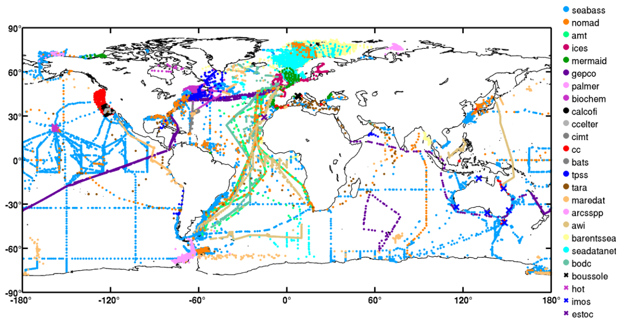
Figure 9. Global distribution of chlorophyll-a concentration per data set in the final table. All chlorophyll data were considered, but for a given station, HPLC data were selected if available. Crosses show sites from where data of chlorophyll are available in a specific geographic location.
