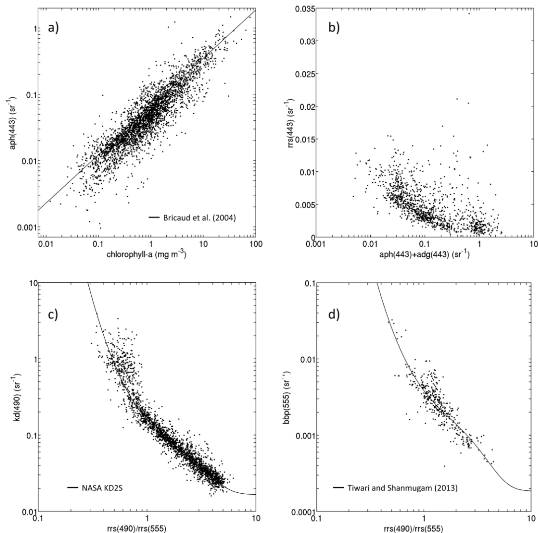
Figure 16. Examples of bio-optical relationships in the final merged table: (a) \text{aph}(443) versus chlorophyll-a. Total number of points (2,953) is divided between AWI (334), COASTCOLOUR (335), MERMAID (214), NOMAD (991), SeaBASS (124) and TPSS (955). For reference the solid line show the regression from Bricaud et al. (2004). (b) [\text{aph}(443) + \text{adg}(443)] versus \text{rrs}(443) . Total number of points (1,112) is divided between MERMAID (33) and NOMAD (1,079). (c) [\text{rrs}(490)/\text{rrs}(555)] versus \text{kd}(490) . The total number of points (2,280) is divided between MERMAID (62), NOMAD (2,117) and SeaBASS (101). For reference the solid line show the NASA KD2S standard algorithm ( http://oceancolor.gsfc.nasa.gov/cms/atbd/kd_490 ). (d) [\text{rrs}(490)/\text{rrs}(555)] versus \text{bbp}(555) . The total number of points (365) is divided between MERMAID (33), NOMAD (324), COASTCOLOUR+SeaBASS (4). For reference the solid line show the relation proposed by Tiwari and Shanmugam (2013). A search window of 2 nm was used for (a) and (b), and a search window of 5 nm was used for (c) and (d) to include data at 560 nm when not available at 555 nm.
