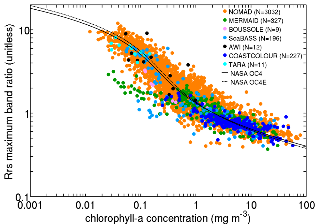
Figure 11. A remote-sensing reflectance maximum band ratio (as defined in text) ( [443,490,510]/555 or [443,490,510]/560 if 555 not available) as a function of chlorophyll-a concentration. All chlorophyll data were considered, but for a given station, HPLC data were selected if available. Data within 2 nm of the wavelengths were used. For reference, the solid and dotted lines show the NASA OC4 and OC4E v6 standard algorithms, respectively ( http://oceancolor.gsfc.nasa.gov/cms/atbd/chlor_a ). The total number of points was 3,814, of which 79% were from NOMAD.
