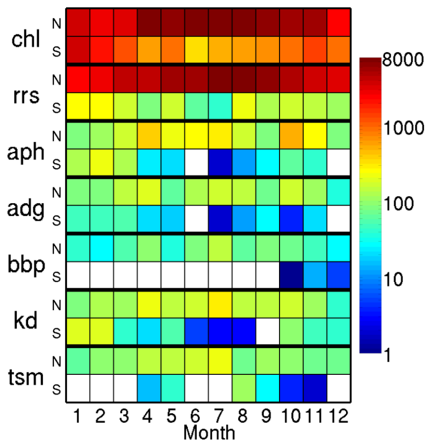
Figure 3. Temporal distribution of chlorophyll-a concentration (“chl”), remote-sensing reflectance (“rrs”), algal pigment absorption coefficient (“aph”), detrital plus CDOM absorption coefficient (“adg”), particle backscattering coefficient (“bbp”), the diffuse attenuation coefficient for downward irradiance (“kd”) and total suspended matter (“tsm”) in the final table. All chlorophyll data were considered, but for a given station, HPLC data were selected if available. Colours indicate the number of stations available for each variable, as a function of month and hemisphere of data acquisition (“N” - Northern Hemisphere; “S” - Southern Hemisphere).
