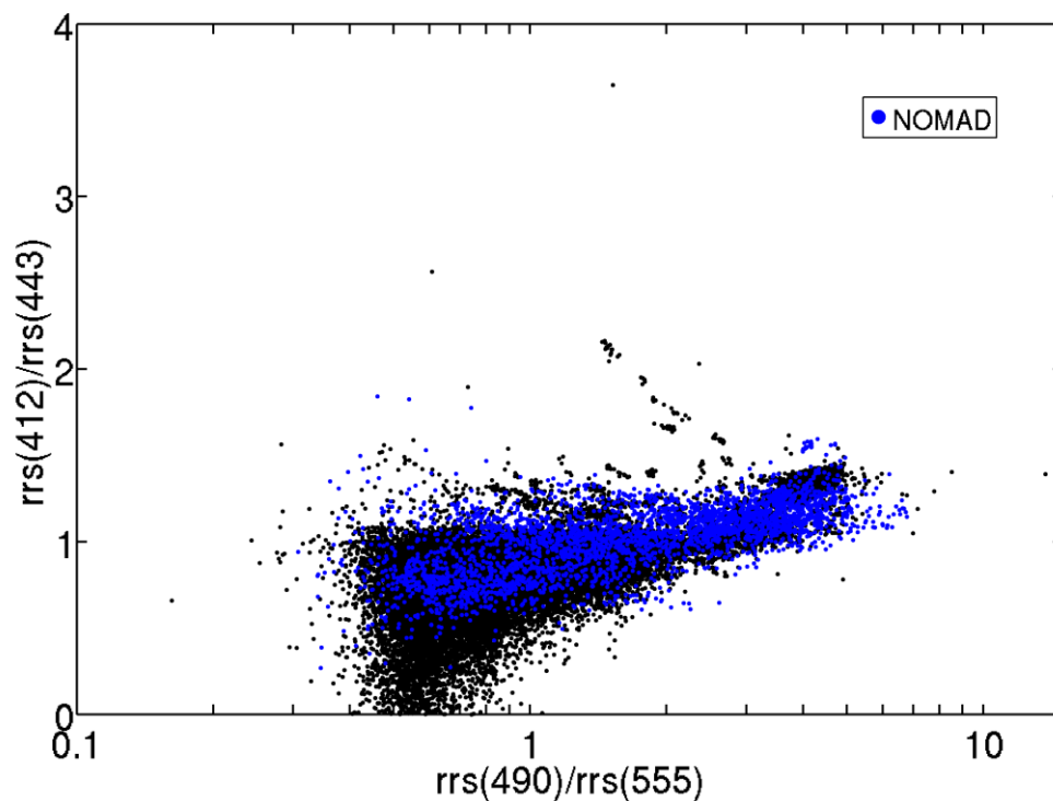
Figure 4. Ranges of remote-sensing reflectance band ratios (412:443 and 490:555) for all data. The points from the NOMAD data set are shown in blue for reference. To maximize the number of ratios per data set a search window up to 12 nm was used, when the four wavelengths (412, 443, 490, 555) were not simultaneously available. The effect of different search windows was negligible in the ratio distribution.
