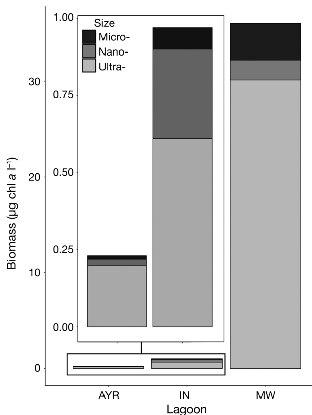
Fig. 2. Contribution of ultraphytoplankton (<5 \mu\text{m} , light grey), nanophytoplankton (5–20 \mu\text{m} , grey) and microphytoplankton (>20 \mu\text{m} , dark grey) to the total biomass, in the oligo- (AYR), meso- (IN) and hypertrophic (MW) lagoons (see Fig. 1) in summer 2014
