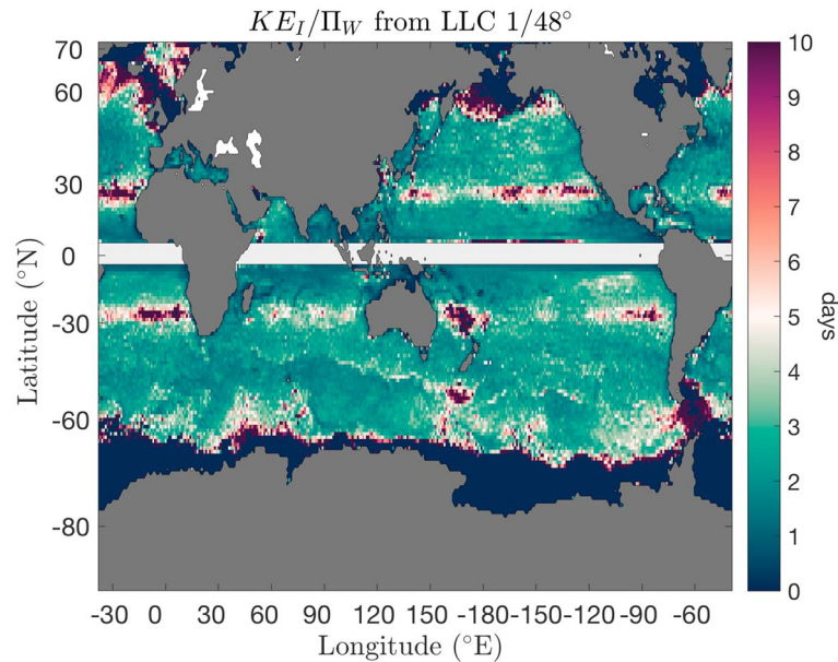
Figure 13. Decay rate, in days, calculated as the ratio between annual-mean estimates of KE_I and \Pi_W from LLC 1/48°. LLC = Latitude-Longitude-polar Cap.
