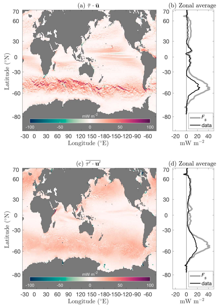
Figure 4. Spatial distributions of (a,b) time-mean fluxes, \bar{\tau} \cdot \bar{\mathbf{u}} , and (c,d) eddy fluxes, \overline{\tau' \cdot \mathbf{u}'} from LLC 1/48°. Surface kinetic energy fluxes ( F_s ) have been divided into a time-mean component ( \bar{\tau} ) and an eddy component using a Reynolds decomposition, where F_s = \bar{\tau} \cdot \bar{\mathbf{u}} = \bar{\tau} \cdot \bar{\mathbf{u}} + \tau' \cdot \mathbf{u}' . (b) and (d) are the respective zonal averages of (a) and (c), “data” presented in black. For comparative purposes, the zonal average of total wind energy input is also shown, F_s presented in gray.
