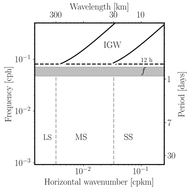
Figure 3. Schematic of the wavenumber/frequency regimes considered in this study. The large scale (LS) contains lengthscales, L > 300 km and periods T > 1.25f . The mesoscale (MS) is defined by 300 \text{ km} > L > 30 km and periods T > 1.25f . The submesoscale (SS) has L < 30 km and periods T > 1.25f . The semidiurnal band (12 hr) includes periods from 12.66 to 11.97 hr and all wavenumbers. The inertial band ( f ) spans over all the inertial periods included in the domain (which may lead to overestimation) and all wavenumbers. The internal gravity wave field (IGW) is the continuum between normal mode 1 and normal mode 10 (the highest normal mode allowed by the horizontal resolution of the numerical model), for periods T < 12.66 hr.
