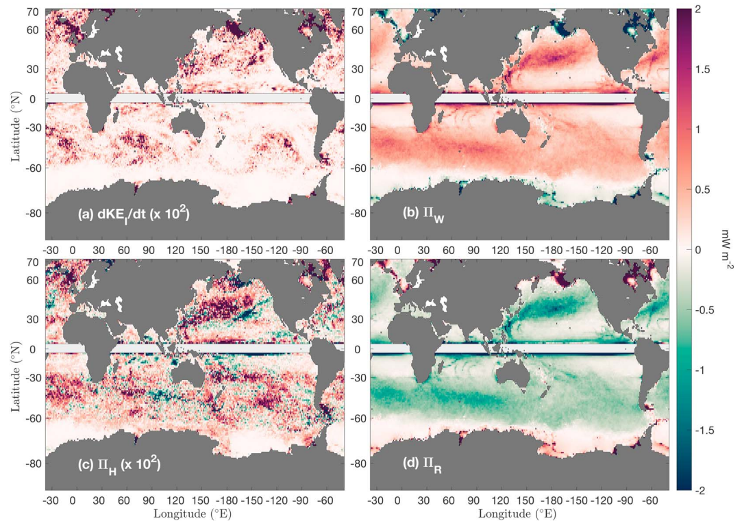
Figure 11. Annual-mean estimates of (a) rate of change in KE_I , (b) \Pi_W , (c) \Pi_H , and (d) \Pi_R (in mW/m^2 ) calculated from LLC 1/48° hourly wind stress and ocean currents. Note the change in scale: (a) and (c) are two orders of magnitude smaller than (b) and (d).
