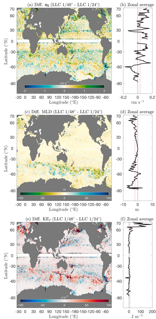
Figure 9. Maps and zonal averages of annual-mean differences (LLC 1/48°-LLC 1/24°) from (a, b) surface near-inertial currents, (c, d) MLD, and (e, f) KE_I . LLC = Latitude-Longitude-polar Cap; MLD = mixed layer depth.
