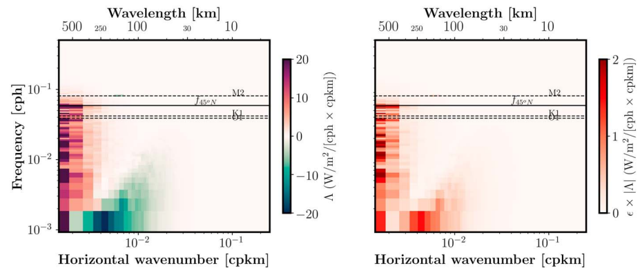
Figure B2. Frequency-wavenumber cospectrum of wind stress and ocean surface currents (left) and Root-Mean-Square error for the cospectrum (right).
