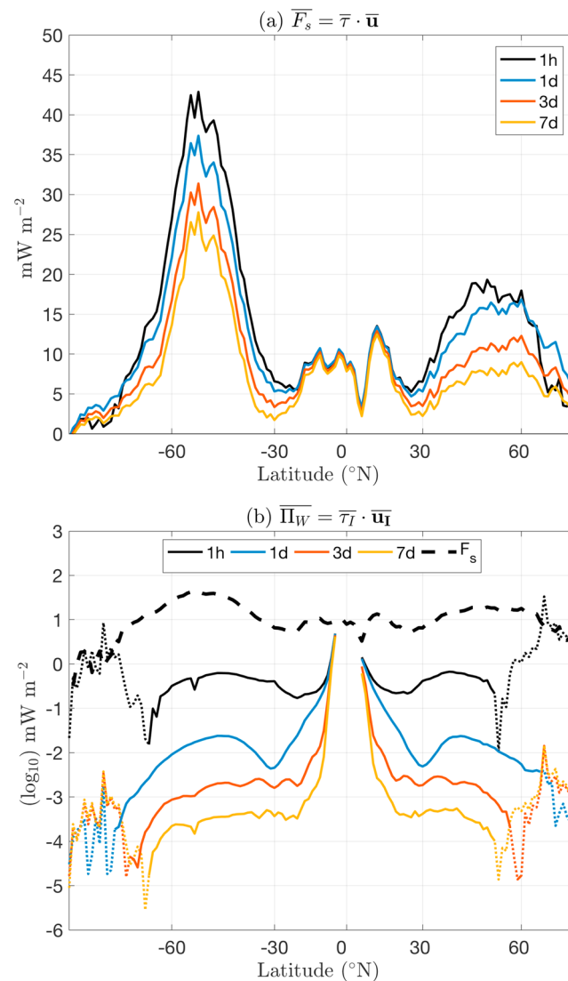
Figure 5. Impact of temporally averaging wind stress and surface currents (denoted with overline bars) on surface kinetic energy fluxes. Colors denote the averaging windows applied to each variable. (a) Zonal averages of surface kinetic energy fluxes from hourly mean (black), daily-mean (blue), 3-day mean (orange), and 7-day mean (yellow) variables. (b) Same as (a), for the near-inertial band. For reference, hourly mean total surface kinetic energy fluxes are shown (thick broken black line). Note the logarithmic scale in (b). Dotted lines indicate negative logarithmic values of \Pi_W (under ice).
