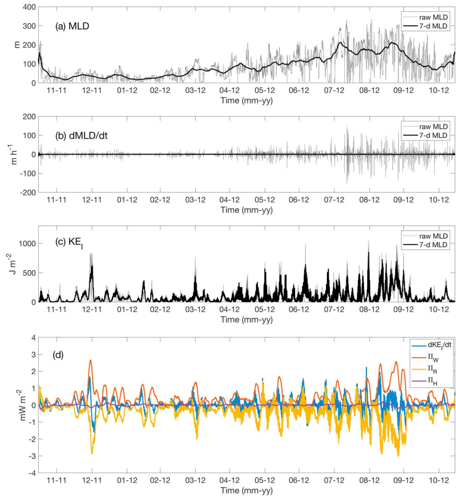
Figure 10. Time series of (a) MLD, (b) rate of change of MLD, and (c) near-inertial energy in the mixed layer ( KE_I ) East of Kerguelen ( 43^\circ S, 93^\circ E). Quantities obtained directly from Latitude-Longitude-polar Cap MLD output are shown in light gray (raw), while those obtained from MLD filtered using a 7-day moving average window are shown in black. (d) Near-inertial kinetic energy budget terms: dKE_I/dt (blue), \Pi_W (red), \Pi_R (yellow), and \Pi_H (magenta). MLD = mixed layer depth.
