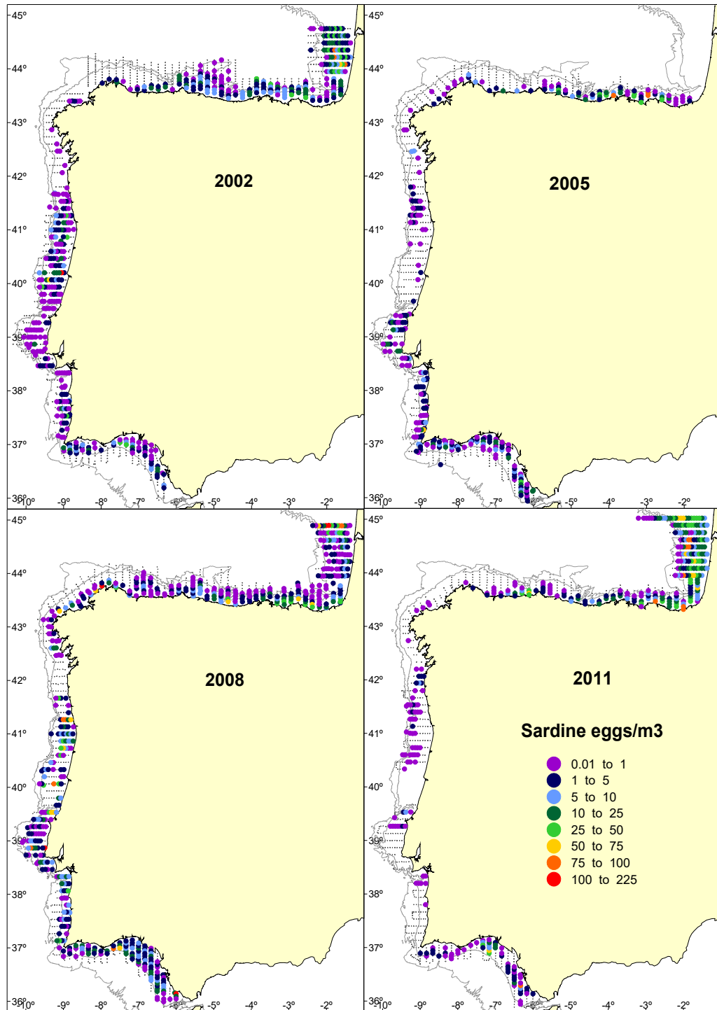
Figure 2.1.2b. Egg distribution ( \text{eggs m}^{-3} ) during the DEPM surveys for the Atlanto-Iberian sardine stock derived from CUFES sampling.
