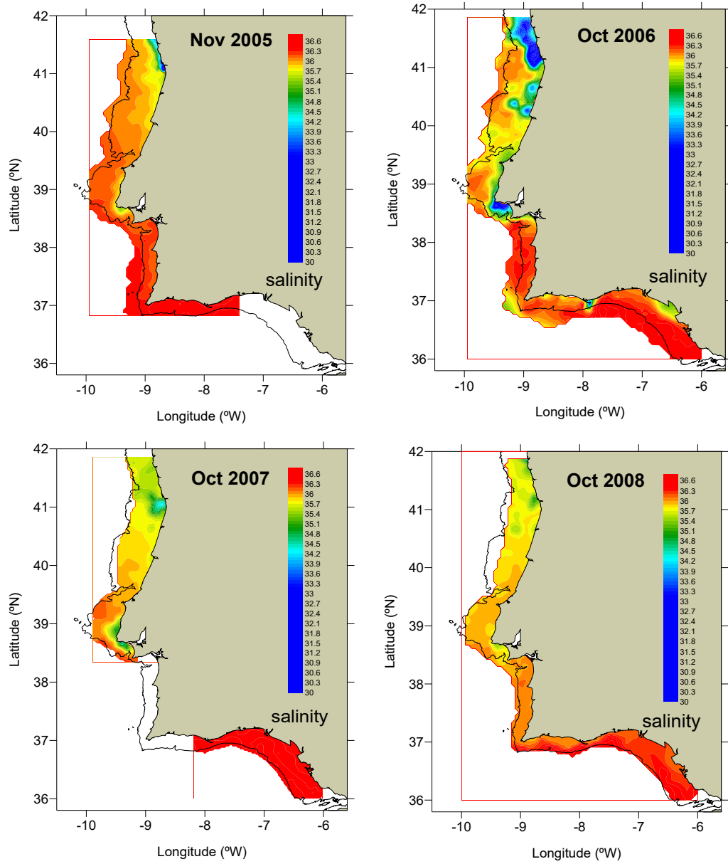
Figure 2.7.7. Sea surface salinity distribution contour derived from the CUFES CT sensor.
