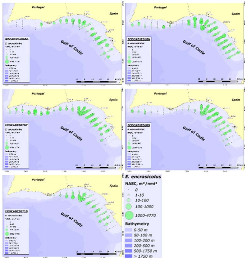
Figure 2.4.4. ECOCADIZ survey series. Distribution of the backscattering energy (nautical area scattering coefficient, NASC, in \text{m}^2 nautical mile -2 ) attributed to anchovy ( Engraulis encrasicolus ). BOCADIVA 0604 (2004), ECOCADIZ 0606 (2006), ECOCADIZ 0707 (2007), and ECOCADIZ 0609 (2009) and 0710 (2010) surveys.
