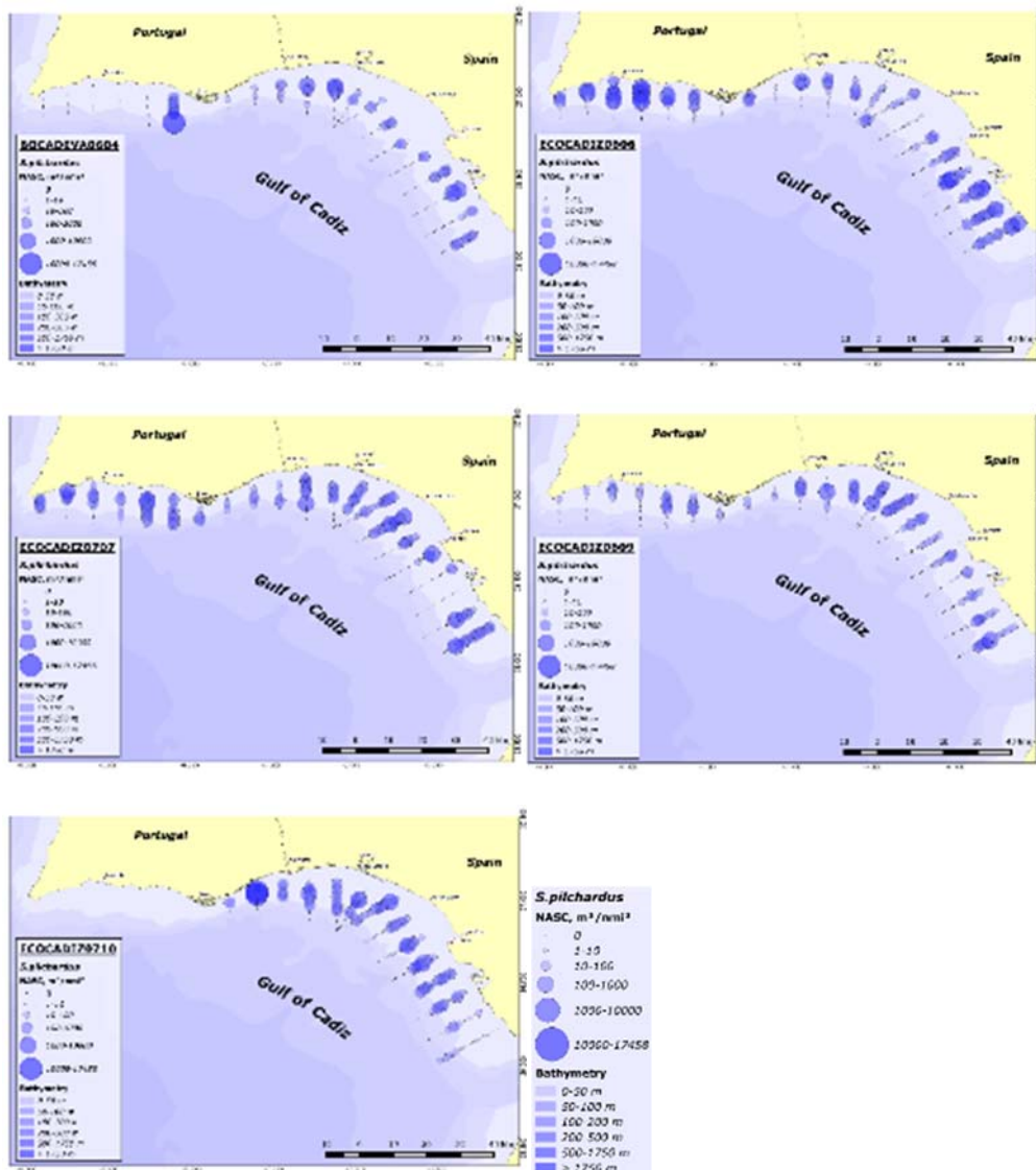
Figure 2.4.5. ECOCADIZ survey series. Distribution of the backscattering energy (nautical area scattering coefficient, NASC, in m^2 nautical mile ^{-2} ) attributed to sardine ( Sardina pilchardus ). BOCADEVA 0604 (2004), ECOCADIZ 0606 (2006), ECOCADIZ 0707 (2007), and ECOCADIZ 0609 (2009) and 0710 (2010) surveys.
