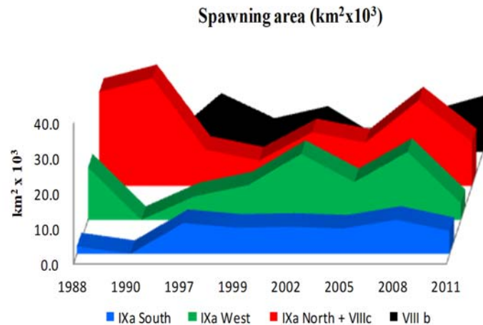
Figure 2.1.4. Spawning area ( \text{km}^2 \times 10^3 ) estimate in the DEPM surveys for the Atlanto-Iberian sardine stock. In 1990, only the northern Spanish coast was sampled.
