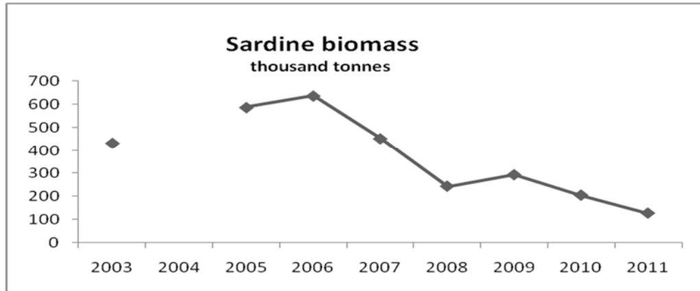
Figure 2.2.28. Sardine biomass (thousand tonnes) in the surveyed area during the spring survey series. Cádiz area was not covered in the 2004 survey.
