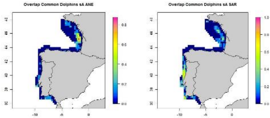
Figure 4.10.2. Occurrence frequency in the yearly overlap between common dolphins and anchovy (left) and sardine (right).
