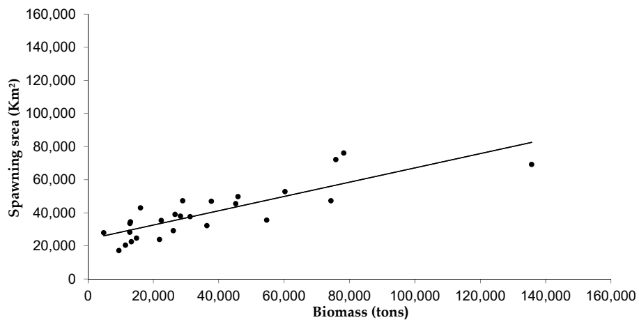
Figure 2.3.9. Relationship between spawning area (km 2 ) and anchovy biomass estimates (tonnes) by the DEPM. Data from the whole historical series (1987–2013).
