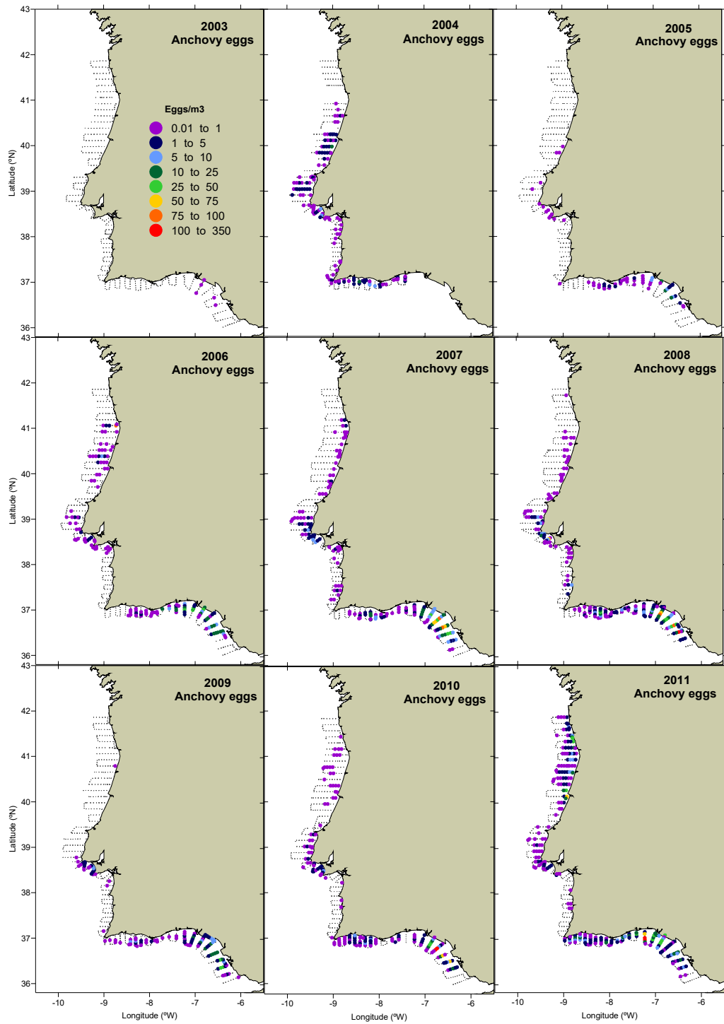
Figure 2.2.33. Anchovy egg density (eggs m^{-3} ) distribution during the acoustic surveys (2003–2011) derived from the CUFES sampler (equipped with a 500- \mu m mesh net in 2003–2004 and a 335- \mu m mesh net in 2005–present).
