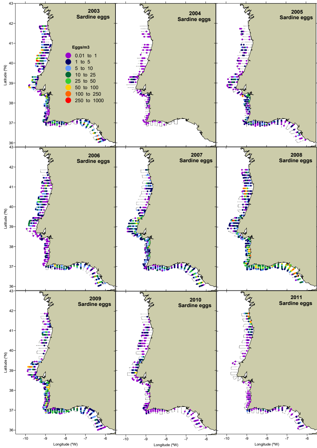
Figure 2.2.32. Sardine egg density (eggs m -3 ) distribution during the acoustic surveys (2003–2011) derived from the CUFES sampler (equipped with a 500- \mu m mesh net in 2003–2004 and a 335- \mu m mesh net in 2005–present).
