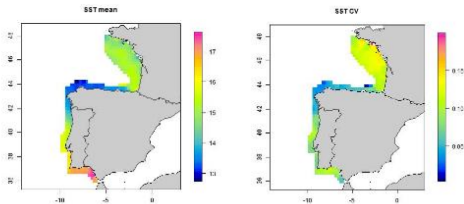
Figure 4.2.1. Spring sea surface temperature: time average (left) and CV (right).
