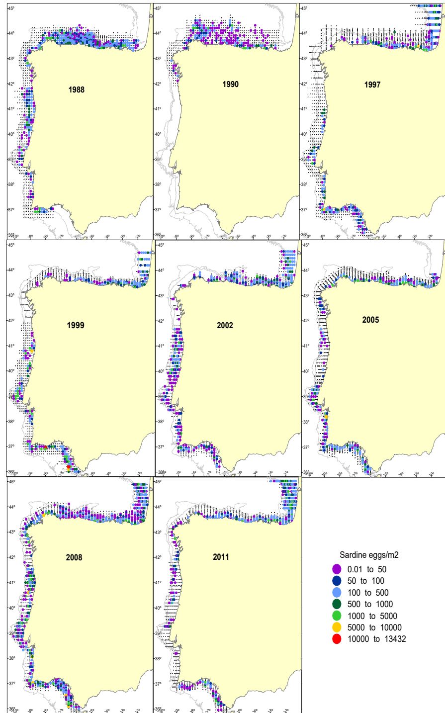
Figure 2.1.2a. Egg distribution during the DEPM surveys for the Atlanto-Iberian sardine stock derived from PairoVET (eggs m -2 ). In 1990, only the northern Spanish coast was sampled.
