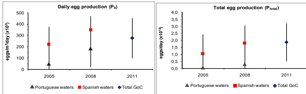
Figure 2.5.5. Daily egg production per surface unit (left) and total egg production (right) for anchovy in the Gulf of Cádiz, estimated by the DEPM (BOCADEVA surveys) (CV in bars).
