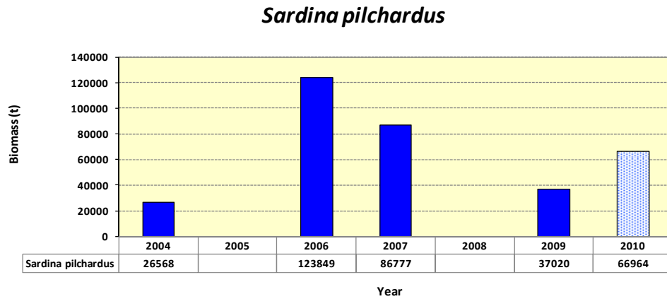
Figure 2.4.6. ECOCADIZ survey series. Recent trends in biomass estimates (in tonnes) for anchovy (top) and sardine (bottom). Gaps for the 2005 and 2008 anchovy acoustic estimates are filled with the BOCADEVA DEPM survey estimates (see Section 2.5.1). Note that the 2010 survey only partially covered the study area.
