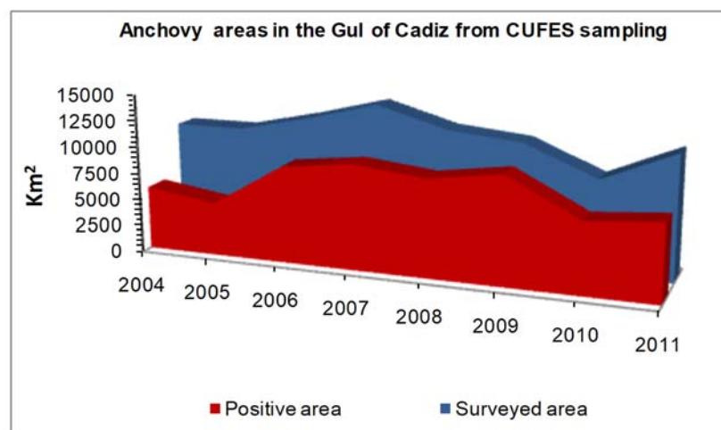
Figure 2.5.4. Surveyed and positive areas by CUFES: acoustic (2004, 2006, 2007, 2009, and 2010) and DEPM (2005, 2008, and 2011) surveys. In 2010, the survey was only from Strait of Gibraltar to Cape Santa Maria.
