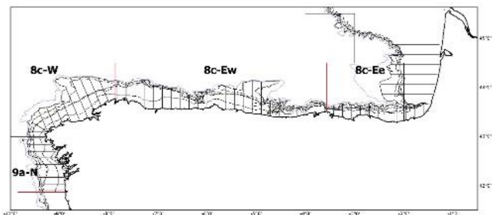
Figure 2.2.10. Spanish acoustic transects (in black) and ICES divisions (9.a N; 8.c W; 8.c EW [western part]; 8.c EE [eastern part]) considered for abundance estimation (in red).
