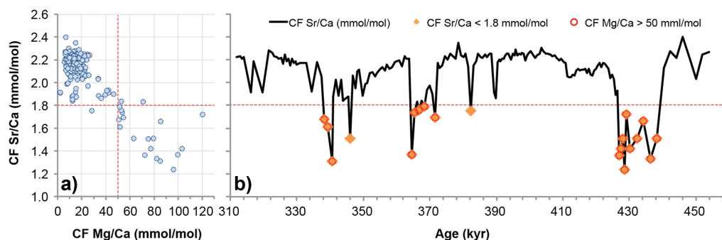
265 Figure 5 Detrital carbonate analysis: a) coccolith fraction (CF) Sr/Ca results and CF Mg/Ca cross-plot. Vertical and horizontal red lines delimit thresholds at 1.8 mol/mol of Sr/Ca and 50 mmol/mol of Mg/Ca, respectively; b) CF Sr/Ca samples possibly subjected to detrital carbonate contamination (red makers), notably associated with cold and abrupt events.
