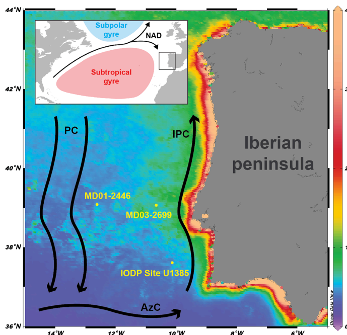
90 Figure 1 Core location and major currents in the area: NAD = North Atlantic Drift; PC = Portugal Current; IPC = Iberian Poleward Current; AzC = Azores Current. Background: chlorophyll a concentration ( \text{mg}\cdot\text{m}^{-3} ; March, April and May average, 2003-2018) derived from MODISA satellite data available at http://disc.sci.gsfc.nasa.gov/giovanni .
