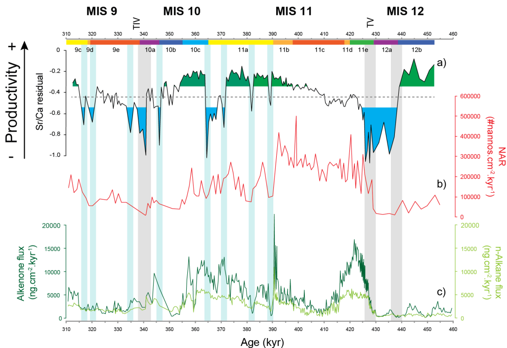
930 Figure 8: Cocolithophore paleoproductivity reconstruction with “high” and “low” coccolithophore productivity levels highlighted in green and blue shading, respectively (a) compared to: b) NAR (Amore et al., 2012) and c) total alkenone flux and n-alkane flux (Rodrigues et al., 2011). Chronology as in Fig. 3. Vertical bars: grey bars correspond to Heinrich-type events and blue bars to short-lived events of decreased coccolithophore productivity.
