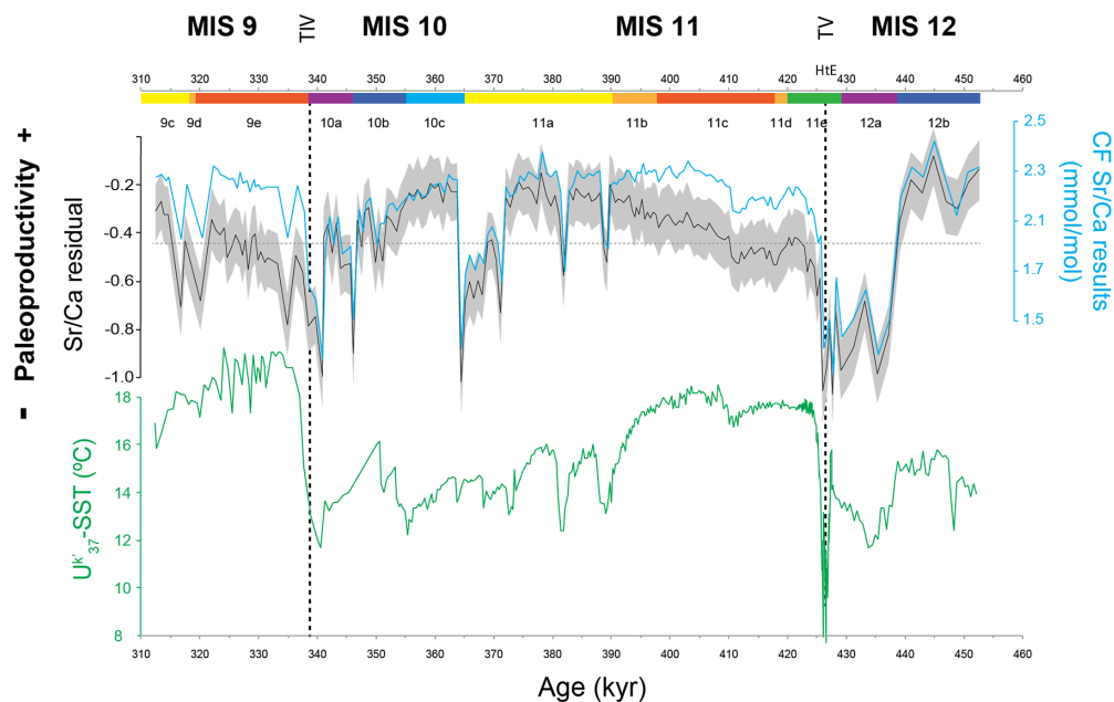
895 Figure 3: Coccolithophore paleoproductivity results from core MD03-2699: coccolith fraction (CF) Sr/Ca ratio and the resulting CF Sr/Ca residual with confidence interval (grey shading represents Monte Carlo 20-80% interval), U^k_{37} -based reconstruction of sea surface temperature (Rodrigues et al., 2011) The horizontal dashed line marks the average value for CF Sr/Ca and CF Sr/Ca residual. The chronology is based on the age model of Voelker et al. (2010), Marine isotope stages (MIS) and substages marked according to Railsback et al. (2015), vertical dashed lines highlight Terminations V and IV.
