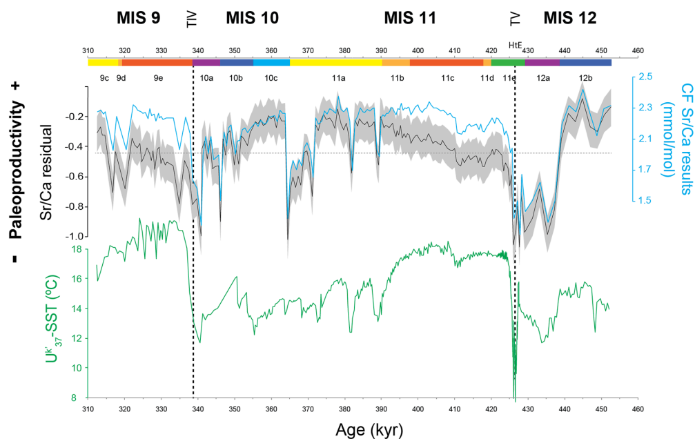
210 Figure 3 Coccolithophore paleoproductivity results from core MD03-2699: coccolith fraction (CF) Sr/Ca ratio and the resulting CF Sr/Ca residual with confidence interval (grey shading represents Monte Carlo 20-80% interval), U^k_{37} -based reconstruction of sea surface temperature (Rodrigues et al., 2011) The horizontal dashed line marks the average value for CF Sr/Ca and CF Sr/Ca residual. The chronology is based on the age model of Voelker et al. (2010), Marine isotope stages 215 (MIS) and substages marked according to Railsback et al. (2015), vertical dashed lines highlight Terminations V and IV.
