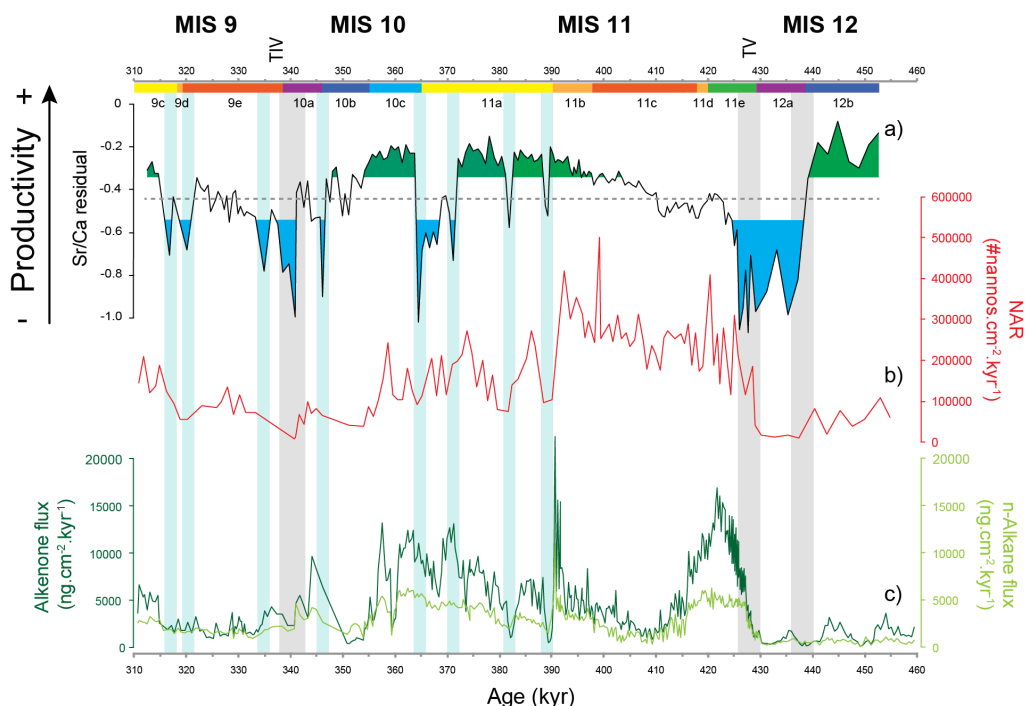
Figure 8 Coccolithophore paleoproductivity reconstruction with “high” and “low” coccolithophore productivity levels highlighted in green and blue shading, respectively (a) compared to: b) NAR (Amore et al., 2012) and c) total alkenone flux and n-alkane flux (Rodrigues et al., 2011). Chronology as in Fig. 3. Vertical bars: grey bars correspond to Heinrich-type events and blue bars to short-lived events of decreased coccolithophore productivity.
