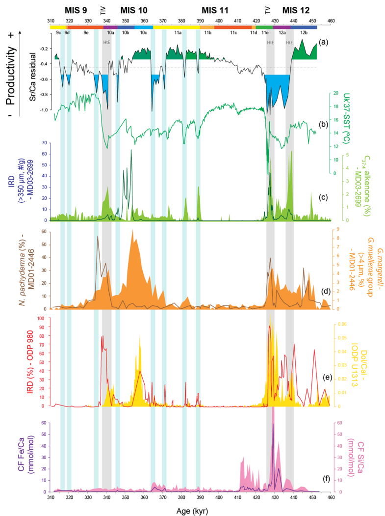
240 Figure 4 Coccolithophore paleoproductivity reconstruction with “high” and “low” coccolithophore productivity levels highlighted in green and blue shading, respectively (a) compared to: b) U^{k^1}_{37} -based reconstruction of sea surface temperature from core MD03-2699 (Rodrigues et al., 2011); c) ice-rafted debris (IRD) abundance (Voelker et al., 2010) and heptatriatetraenone ( C_{37:4} alkenone) abundance (Rodrigues et al., 2011), both from core MD03-2699; d) Neogloboquadrina pachyderma relative abundance and Gephyrocapsa margereli and G. muelleriae group relative abundance, both from core
