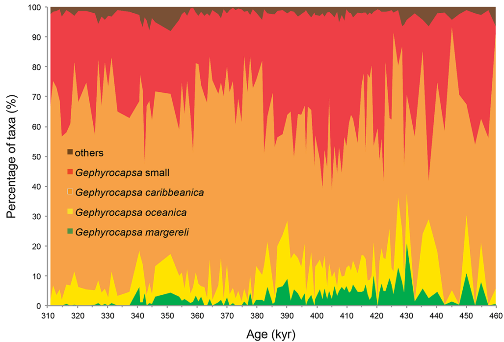
890 Figure 2: Composition of coccolith assemblages in core MD03-2699 based on Amore et al. (2012). Note that only a minor percentage of coccoliths belong to groups other than the dominant Gephyrocapsids. The chronology is based on the age model of Voelker et al. (2010).
