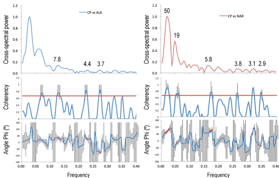
935 Figure 9: Cross-spectral analysis results for Coccolithophore paleoproductivity (CP) and alkenone flux (ALK – blue line; Rodrigues et al., 2011) and nannofossil accumulation rate (NAR – red line; Amore et al., 2012). The quasi-periodicities are given on top each significant peak on the cross-spectral results. The red line in coherency results defines the significance level of 80% (bandwidth is 0.02). All estimation errors are shown as vertical lines. Red dots highlight the angles for which significant quasi-periodicities exist.
