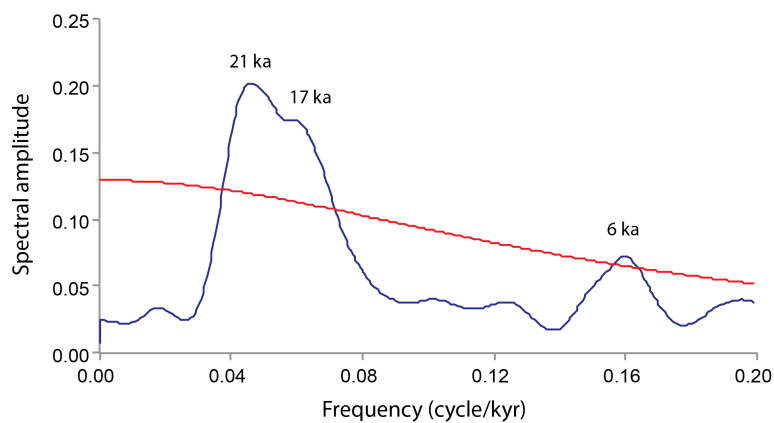
920 Figure 6: Coccolithophore paleoproductivity time-series analysis showing significant peaks at 21, 17 and 6 ka. The red line defines the significance level of 80% (bandwidth is 0.02), indicating that the peaks at 21 and 17 ka are not independent (may represent the same frequency given the uncertainty of dating and resolution).
