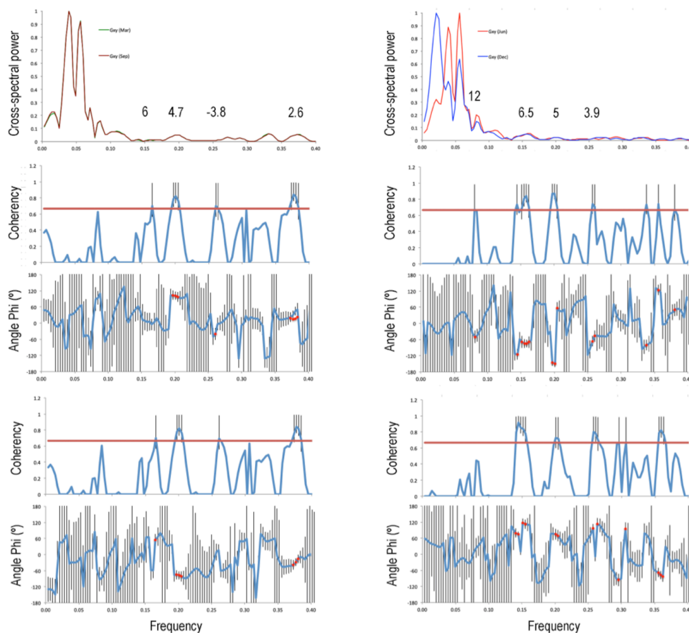
940 Figure 10: Cross-spectral analysis results for Coccolithophore paleoproductivity (PC) and insolation curves: March and September cross spectral analysis results (left panel), June and December cross spectral analysis results (right panel; insolation data from Laskar et al., 2011). The quasi-periodicities are given on top the first four significant peaks on the cross-spectral results. The red line in coherency results defines the significance level of 80% (bandwidth is 0.02). All estimation errors are shown as vertical lines. Red dots highlight the angles for which significant quasi-periodicities exist.
