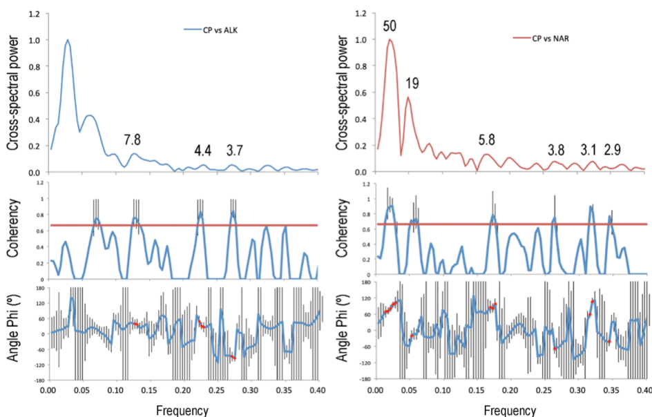
Figure 9 Cross-spectral analysis results for Coccolithophore paleoproductivity (CP) and alkenone flux (ALK – blue line; Rodrigues et al., 2011) and nannofossil accumulation rate (NAR – red line; Amore et al., 2012). The quasi-periodicities are
