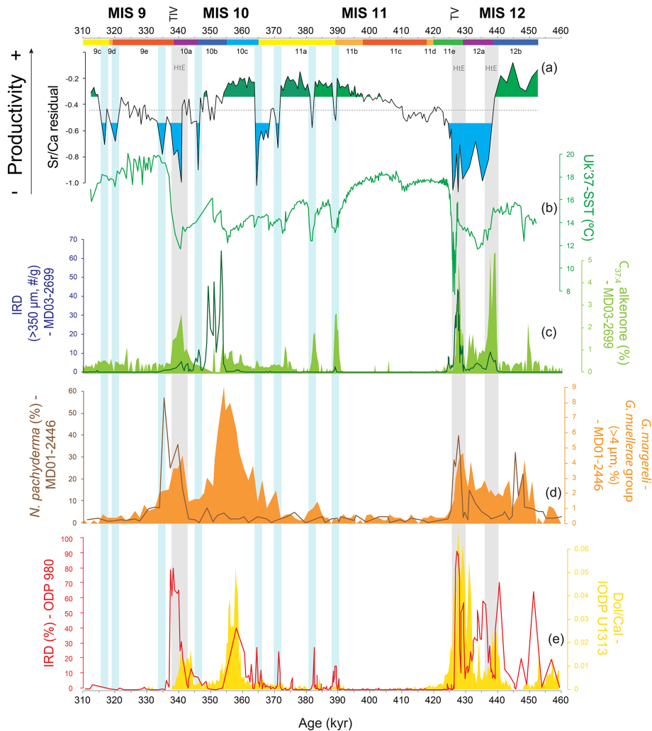
Figure 4. Coccolithophore paleoproductivity reconstruction with “high” and “low” coccolithophore productivity levels highlighted in green and blue shading, respectively ( a ), compared to ( b ) U_{37}^{K'} -based reconstruction of sea surface temperature from core MD03-2699 (Rodrigues et al., 2011); ( c ) ice-rafted debris (IRD) abundance (Voelker et al., 2010) and heptatriatetraenone ( C_{37:4} alkenone) abundance (Rodrigues et al., 2011), both from core MD03-2699; ( d ) Neogloboquadrina pachyderma relative abundance and Gephyrocapsa margaritella and G. muelleriae group relative abundance, both from core MD01-2446 (Marino et al., 2014); ( e ) percentage IRD from ODP Site 980 (McManus et al., 1999) and dolomite/calcite ratio from IODP Site U1313 (Stein et al., 2009). Note that the MD03-2699 lithic fragments were counted in a coarser size fraction ( > 315 \mu\text{m} ) than the standard size fraction ( > 150 \mu\text{m} ; Hemming, 2004) and thus most likely only record major ice-rafting events at the IbM, as suggested by Marino et al. (2014). Chronology as in Fig. 3. Vertical bars: grey bars correspond to Heinrich-type events (HtEs) and blue bars to short-lived events of decreased coccolithophore productivity.
