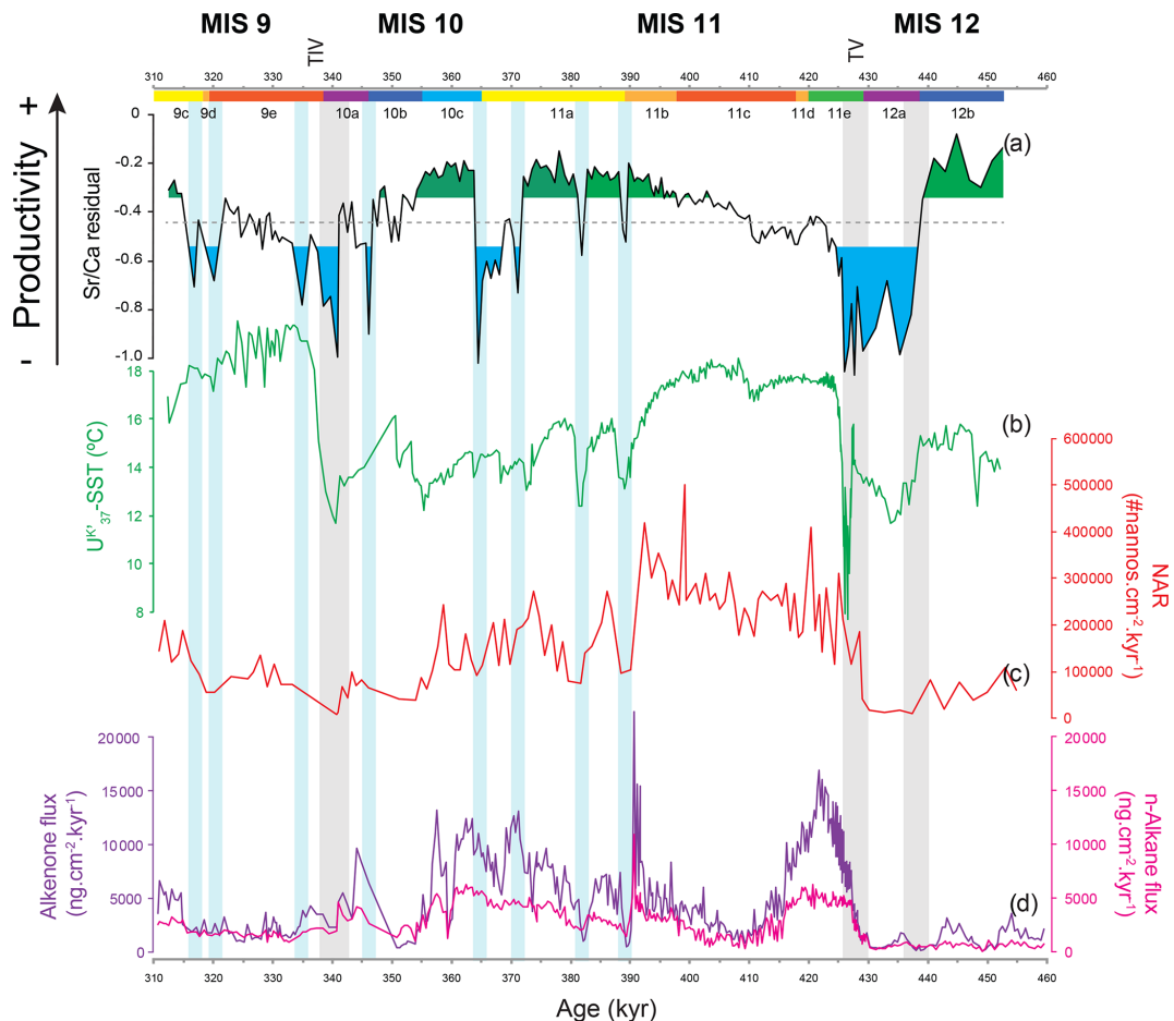
Figure 6. Coccolithophore paleoproductivity reconstruction with “high” and “low” CP levels highlighted in green and blue shading, respectively (a), compared to (b) U^{K'}_{37} -based reconstruction of sea surface temperature (Rodrigues et al., 2011), (c) nanofossil accumulation rate (NAR) (Amore et al., 2012), and (d) total alkenone (AlkAR) and n -alkane accumulation rates (Rodrigues et al., 2011). Chronology as in Fig. 3. Vertical bars: grey bars correspond to Heinrich-type events (HtEs) and blue bars to short-lived events of decreased CP.
