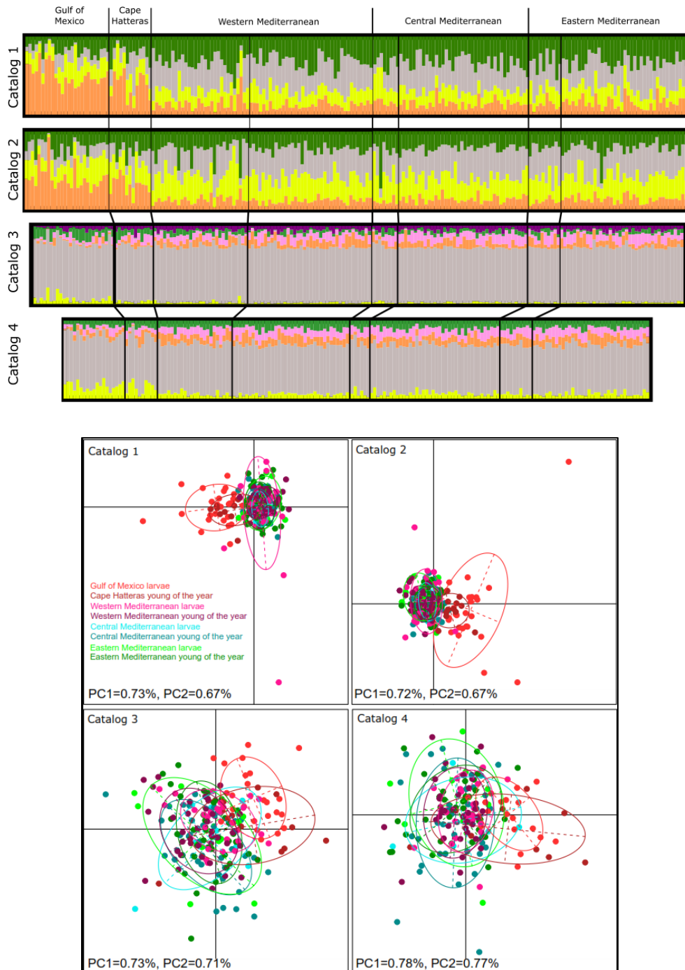
WebFigure 1. Graphical representation of the Bayesian clustering approach for (top panel) the best-supported K value and (bottom panel) principal component analyses (PCAs) for catalogs 1–4.
