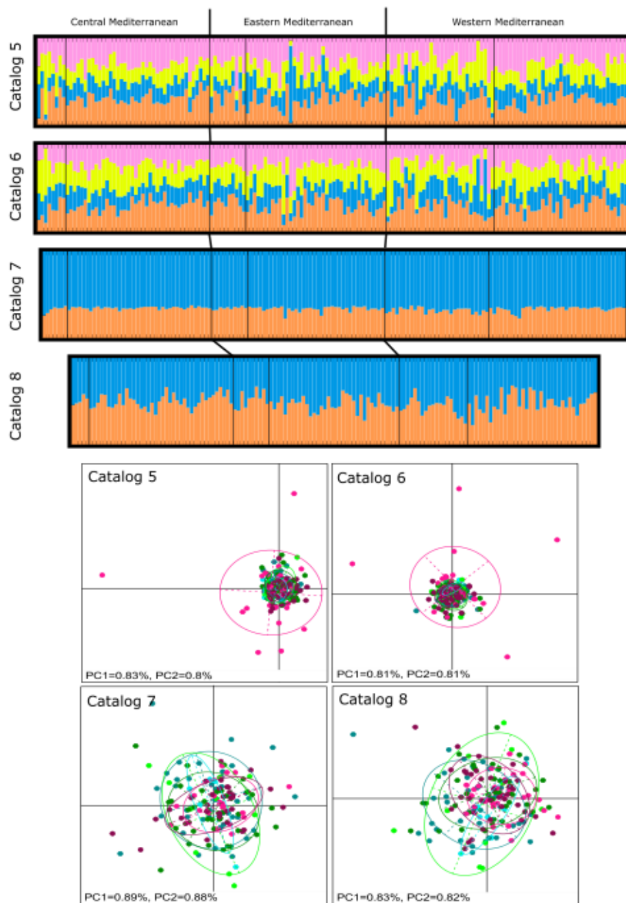
WebFigure 2. Graphical representation of the Bayesian clustering approach for (top panel) the best-supported K value and (bottom panel) PCAs for catalogs 5–8.
