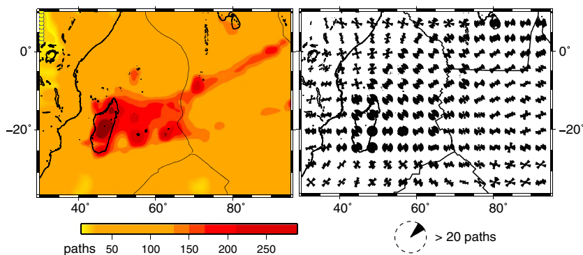
Figure 7. Data set used in the group velocity calculation. (left) Density path map. (right) Azimuthal coverage of the area, where the number of paths per unit area ( 2^\circ \times 2^\circ cell) are binned in the azimuth range of 30^\circ , and the vectors are saturated at 20 paths. There is higher density of paths beneath Réunion and the central/eastern part of the map than beneath Africa; the path coverage is redundant everywhere.
