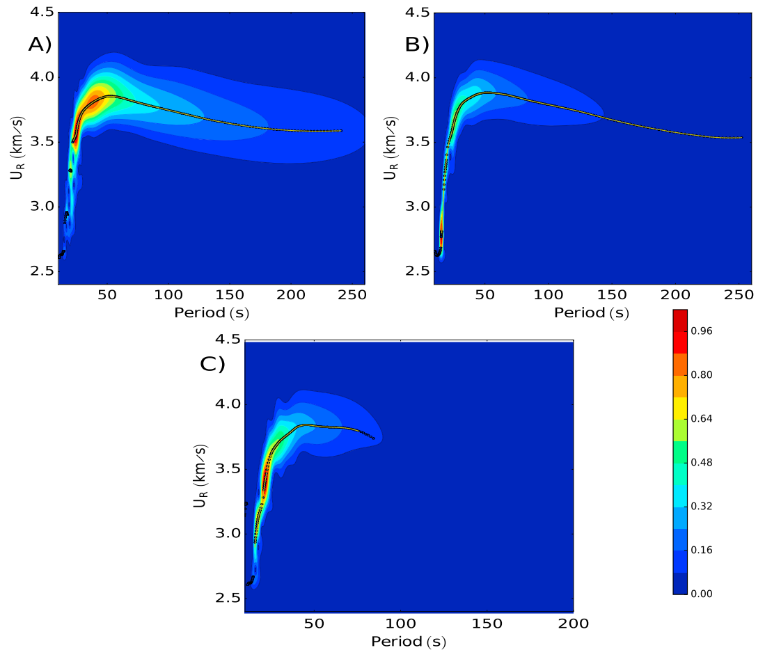
Figure 6. Dispersion curves for an earthquake in Thailand M = 6.8 11 November 2012, as recorded by (a) RER, (b) RR40, and (c) RR01. The colored backgrounds indicate the time frequency signal amplitudes, with red-based colors as the largest amplitudes. The yellow lines show the manually picked dispersion curves. The measured period range is broader for RER and RR40 than for RR01 due to the different sensors in the stations.
