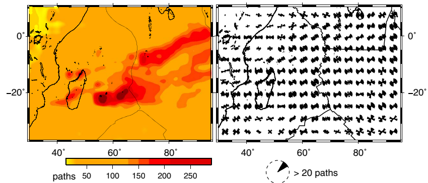
Figure 4. Data set used in the phase velocity calculation. (left) Density path map. (right) Azimuthal coverage of the area, where the number of paths per unit area ( 2^\circ \times 2^\circ cell) is binned in the azimuth range of 30^\circ , and the vectors are saturated at 20 paths. However, the density path beneath Réunion and the central/eastern part of the map is higher than beneath Africa. The path coverage is redundant everywhere.
