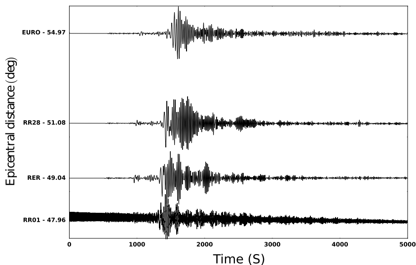
Figure 3. Seismograms corresponding to the event that occurred in Pakistan M = 7.7 (24 September 2013) that were recorded by the French INSU OBS RR28 station, the German DEPAS OBS RR01 station, the Geoscope RER land station (La Réunion Island), and the temporary EURO land station deployed on Europa island in Mozambique Channel.
