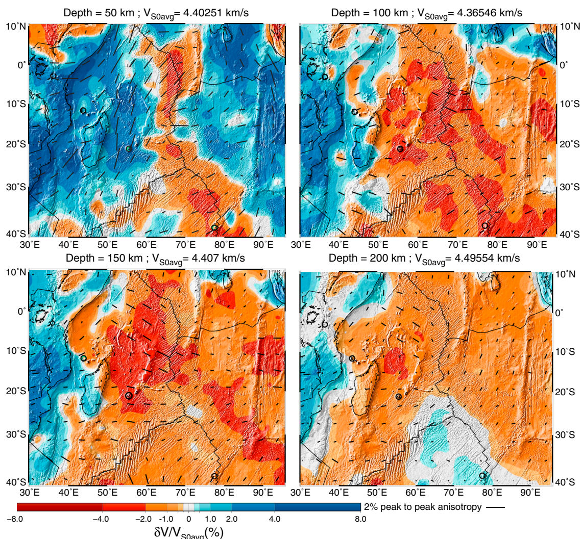
Figure 8. S_V wave velocity perturbation with respect to the mean velocity at the different depths of 50, 100, 150, and 200 km. Fast anisotropy directions are plotted with bars, where the strength is normalized with respect to the maximum value at each depth. Black circles indicate the hot spot locations in the area.
