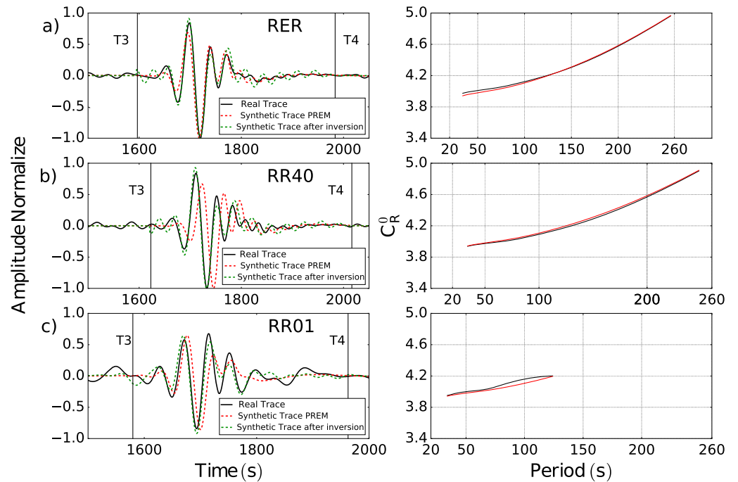
Figure 5. Quality of the fundamental mode measurements is assessed in windows delimited by T3 ( \Delta/U_{\max_0} , where \Delta is the epicentral distance, U_{\max_0} = 4.0 km/s maximum velocity of the fundamental mode) and T4 ( \Delta/U_{\min_0} , where U_{\min_0} = 2.8 km/s minimum velocity of the fundamental mode). (left column) Recorded traces for an earthquake in Thailand M = 6.8 for stations (a) RER, (b) RR40, and (c) RR01. The data are in black (filtered in the 33–333 s period band), the synthetic before and after the inversions are in red and green, respectively. (right column) Measured fundamental mode phase velocity (black), compared to the predicted ones for the Prem model (red).
