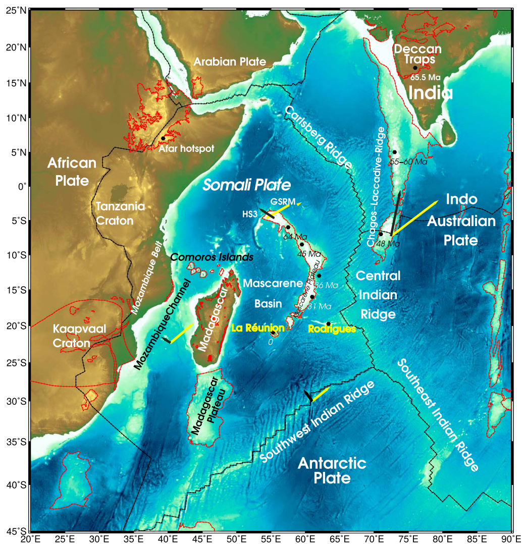
Figure 1. Bathymetry and topography map of the study area (ETOPO1) (Amante & Eakins, 2009). Absolute plate motion vectors (1 cm/yr) calculated from the no net rotation global strain rate model (Kreemer, 2009) are shown in yellow and from the HS3-Nuvel1A model (hot spot frame) (Gripp & Gordon, 2002) in black. The domains inside the red lines represent the volcanic provinces. Crustal ages (Duncan et al., 1990; Duncan & Hargraves, 1990) are indicated with black or white circles.
