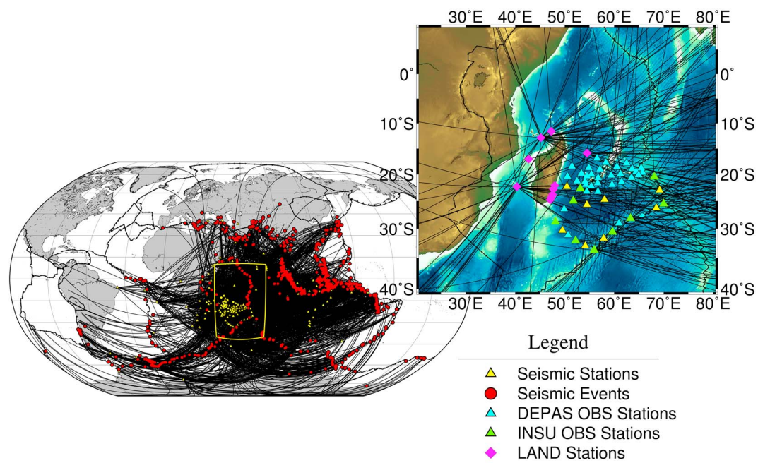
Figure 2. Global distribution of the ~300 earthquakes sources (red) and 130 stations (yellow) used in this study. Black lines show the great circle paths. The magnified panel (right) shows the distribution of the RHUM-RUM stations and the final raypath coverage used in the procedure.
