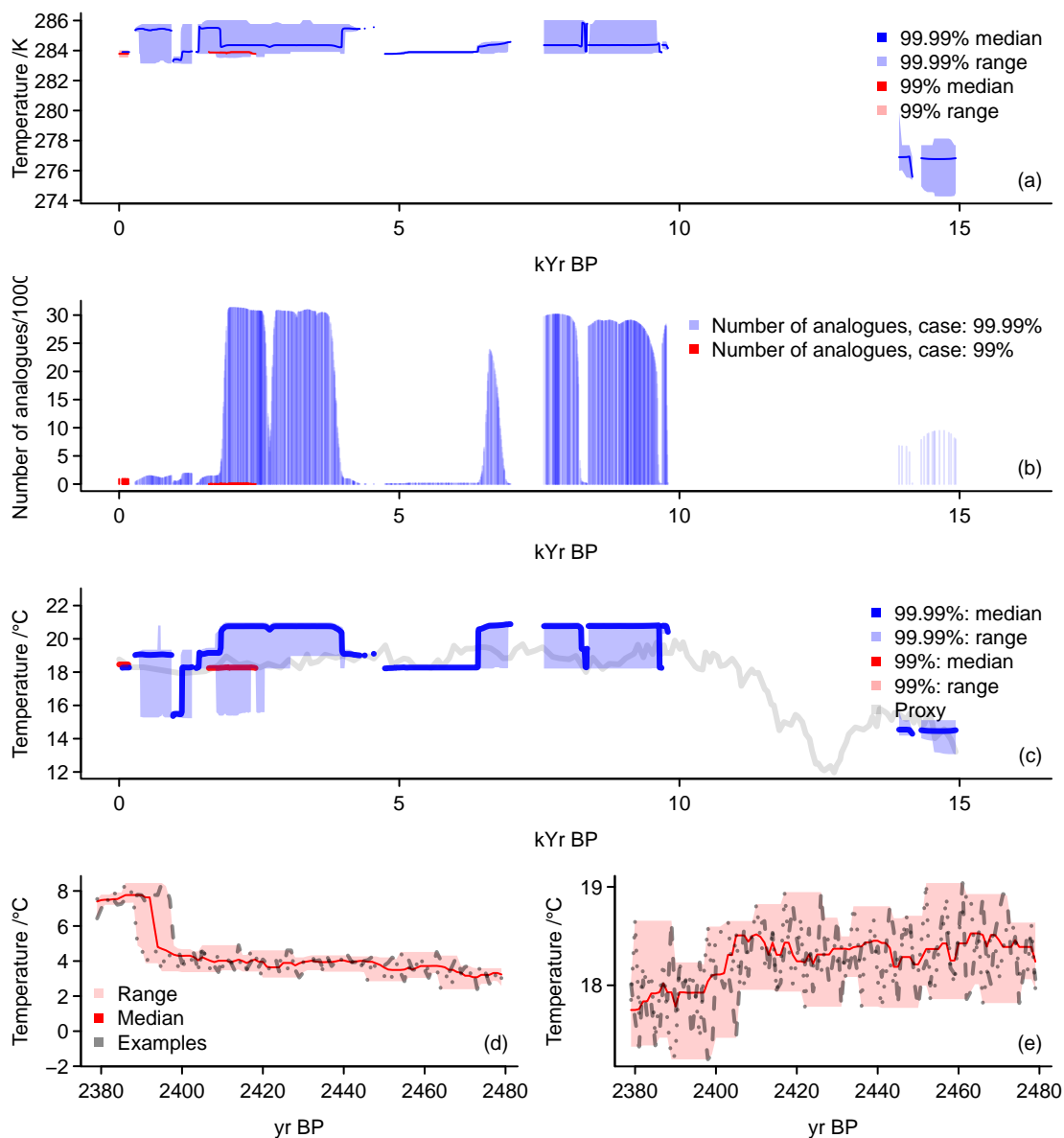
Figure 8. Visualising reconstruction results for the analogue method under two assumed uncertainty envelopes: (a) regional averages for 101-year moving averages, (b) number of analogues, (c) local results for 101-year moving averages, (d,e) expansion of regional (d) and local (e) 101-year moving averages in 101 year series ranges. (a) shows median and range of all analogues for an assumed 99% uncertainty envelope (red) and a 99.99% envelope (blue) for the proxy data. (b) shows the number of analogues found for each of the dates considered; red: 99% envelope, blue: 99.99% envelope. (c) adds for the location of the record MD95-2043 the proxy data (grey), and the range and median of all local analogue values for a 99% envelope (red) and a 99.99% envelope (blue). (d,e) show the median (red), the range (light red), and two examples of the extension of 101-year mean analogues into 101 year long time-series for (d) the regional averages and (e) the location of MD95-2043. (d) and (e) only show results for the 99% uncertainty envelope.
