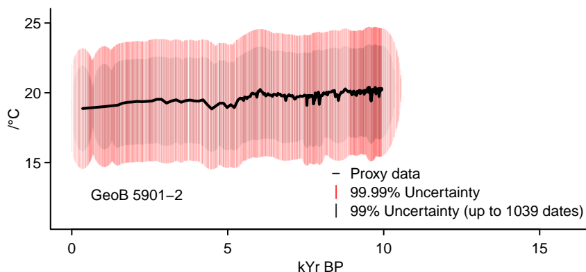
Figure A4. Proxy data and assumed uncertainties for GeoB 5901-2.
