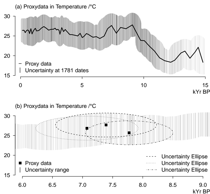
Figure 2. Visualisation of our approach to uncertainty: (a) Example proxy data (line) and assumed data uncertainty at all dates when we reconstruct values. Number of dates are all dates when any of the proxies included has a dated data point. (b) Proxy data at three example dates and uncertainty ellipses for these dates using data uncertainty and age/date uncertainty.
