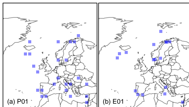
Figure 1. Map of the reconstruction domain and the proxy predictors: (a) for the pseudoproxy setup, (b) for the main proxy setup.
