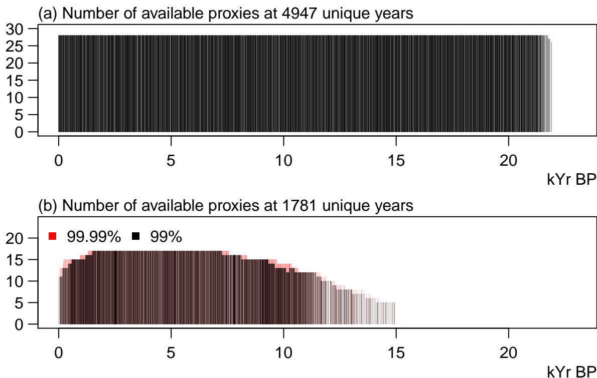
Figure 3. Information about the number of available proxies for the dates to be reconstructed: (a) the pseudoproxy setup, (b) the proxy setup. In (b) we show results for two different assumptions on the uncertainties, a 99% envelope and a 99.99% envelope (compare section 2.2.3).
