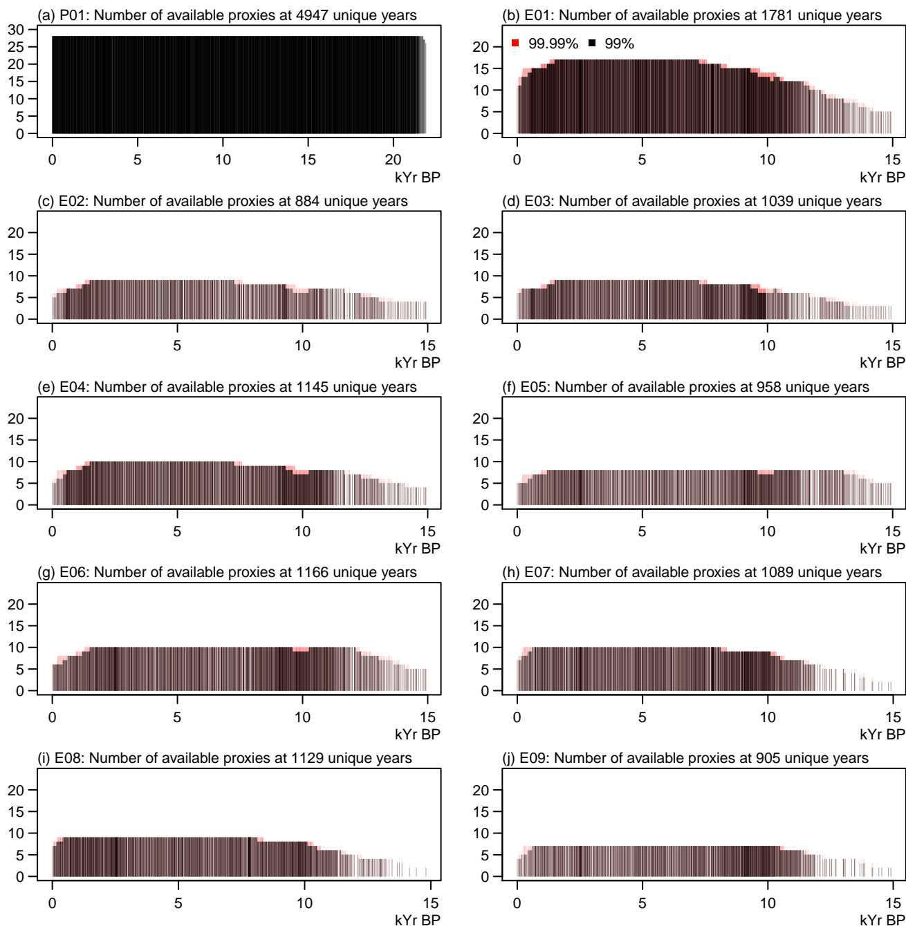
Figure A3. Information about the number of available proxies for the dates to be reconstructed: (a) the pseudoproxy setup, (b) to (j) the various proxy setups according to Figure A2 and Table 1. In (b) to (j) we show results for two different assumptions on the uncertainties, a 99% envelope and a 99.99% envelope (compare section 2.2.3).
