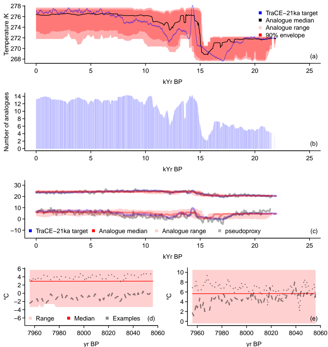
Figure 5. Visualising reconstruction results for the pseudoproxy application of the analogue method: (a) regional averages for 101-year moving averages, (b) number of analogues, (c) local results for 101-year moving averages, (d,e) expansion of regional (d) and local (e) 101-year moving averages in regional and local 101 year series ranges. (a) shows the 101-year moving average regional target in the TraCE-21ka simulation (blue), the median of all analogues (black), the range of all analogues (light red), and the 90% range of the analogues (red). (b) shows the number of analogues found for each of the dates considered. (c) adds for two locations the local pseudoproxy data (grey), the local target (blue), the range of all local analogue values (light red), and the local median of the analogues (red). (d,e) show the median (red), the range (light red), and two examples of the extension of 101-year mean analogues into 101 year long time-series for the (d) regional averages and (e) one location.
