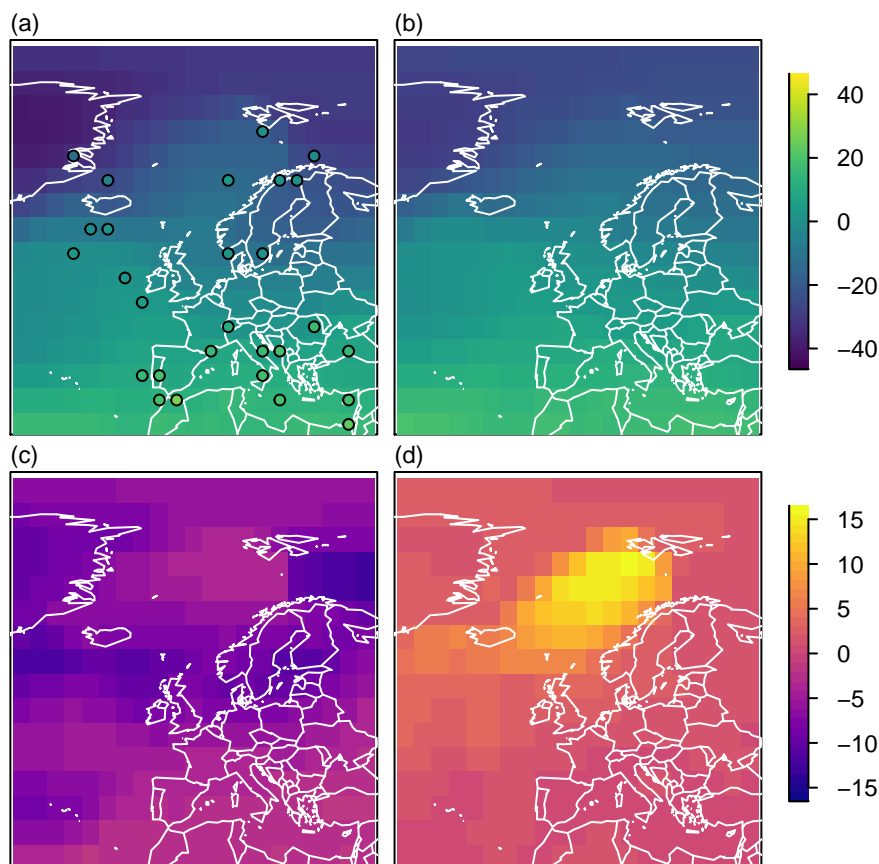
Figure 6. Visualising field information for the pseudoproxy approach: Example of 101-year mean annual temperature analogue reconstruction for the European-North-Atlantic sector in °C. (a) One example analogue, (b) local median of all analogues, (c) local minimum of all analogues, and (d) local maximum of all analogues. Panels (c) and (d) show differences to the median in °C.
