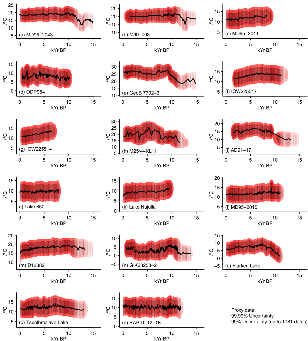
Figure 7. Proxy data and assumed uncertainties for the 17 main proxy record locations in our analogue search under two different uncertainty envelopes.
