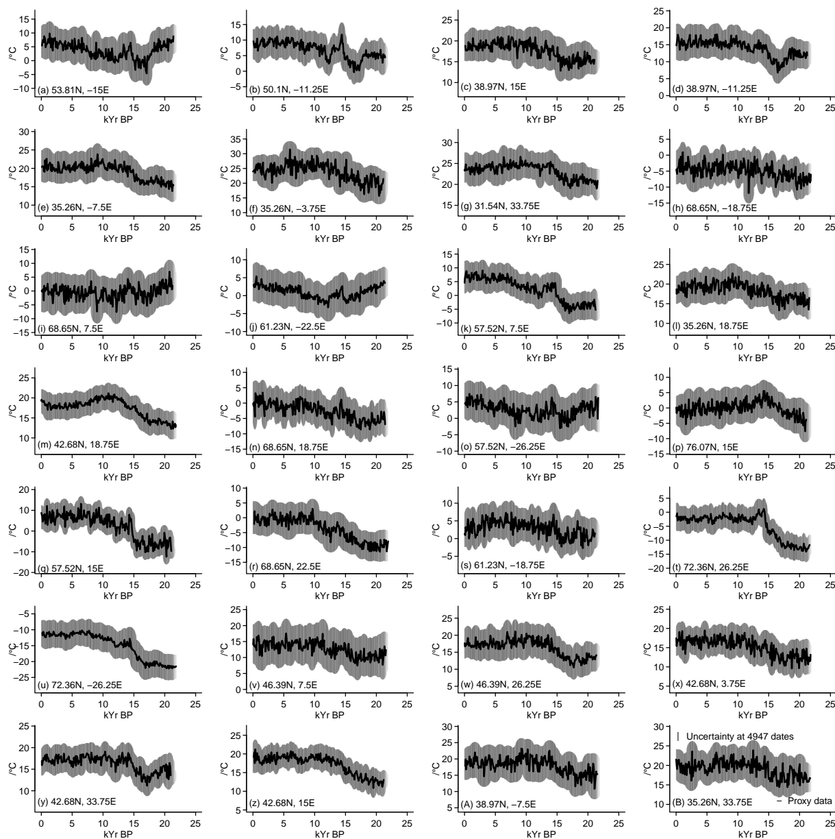
Figure 4. Pseudoproxy data and assumed uncertainties for the 28 locations in our pseudoproxy application.
