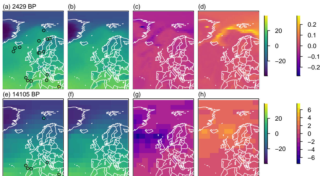
Figure 9. Visualising field information for the analogue search: Two examples of 101-year mean annual temperature analogue reconstruction for the European-North-Atlantic sector in °C. (a,e) One example analogue, (b,f) local median of all analogues, (c,g) difference of local minimum to local median of all analogues, and (d,h) difference of local maximum to local median of all analogues. (a) to (d) are for the 99% uncertainty envelope, (e) to (h) for the 99.99% uncertainty envelope.
