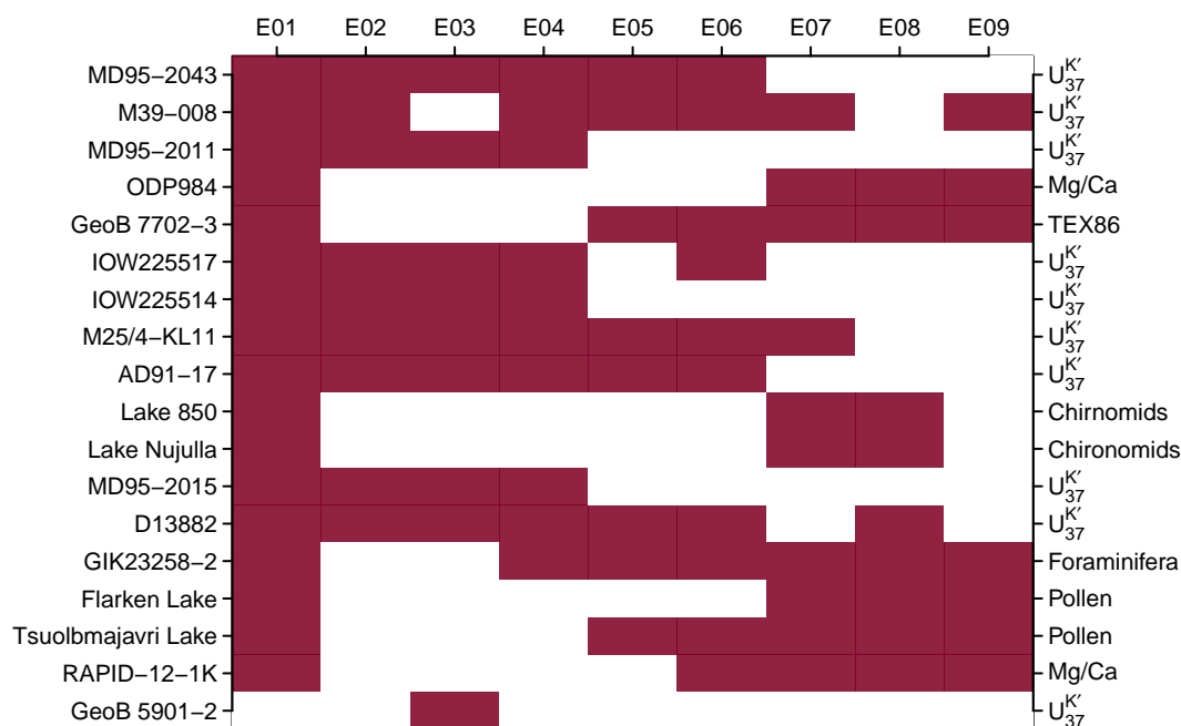
Figure A2. Information about the different proxy setups: Matrix of proxy records against proxy setup (E01-E09). For more information see Table 1. White-out means that the relevant proxy is not included in the respective proxy setup.
