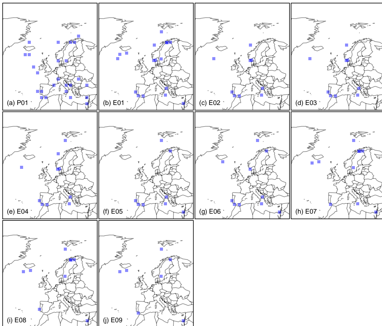
Figure A1. Map of the reconstruction domain and the proxy predictors: (a) for the pseudoproxy setup; (b) to (j) for the different proxy setups. For more details see Table 1 and Figure A2.
