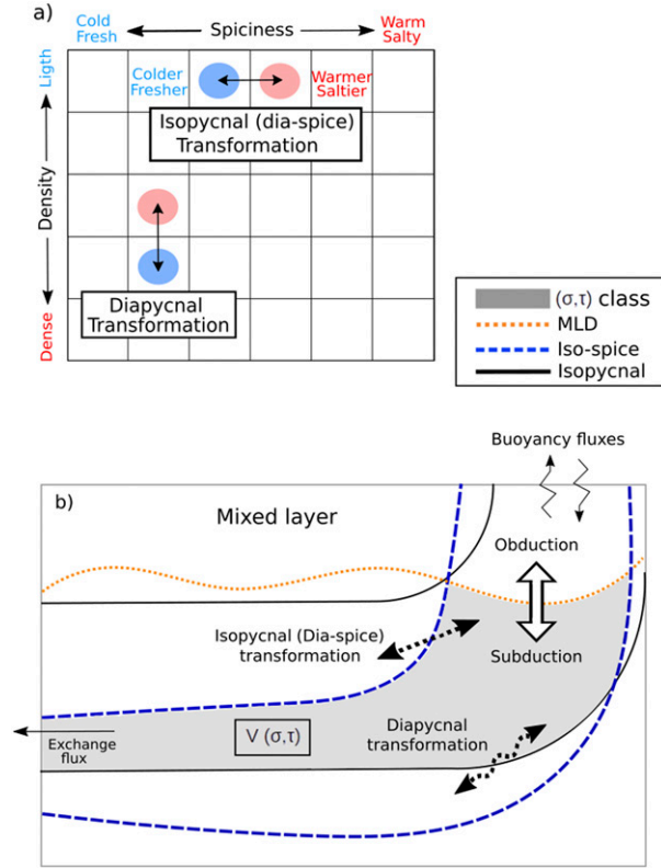
FIG. 1. (a) Diagram showing the effect of the transformation of a given water class in \sigma - \tau space, and (b) processes involved in the volume change of a given \sigma - \tau class in geographical coordinates.
