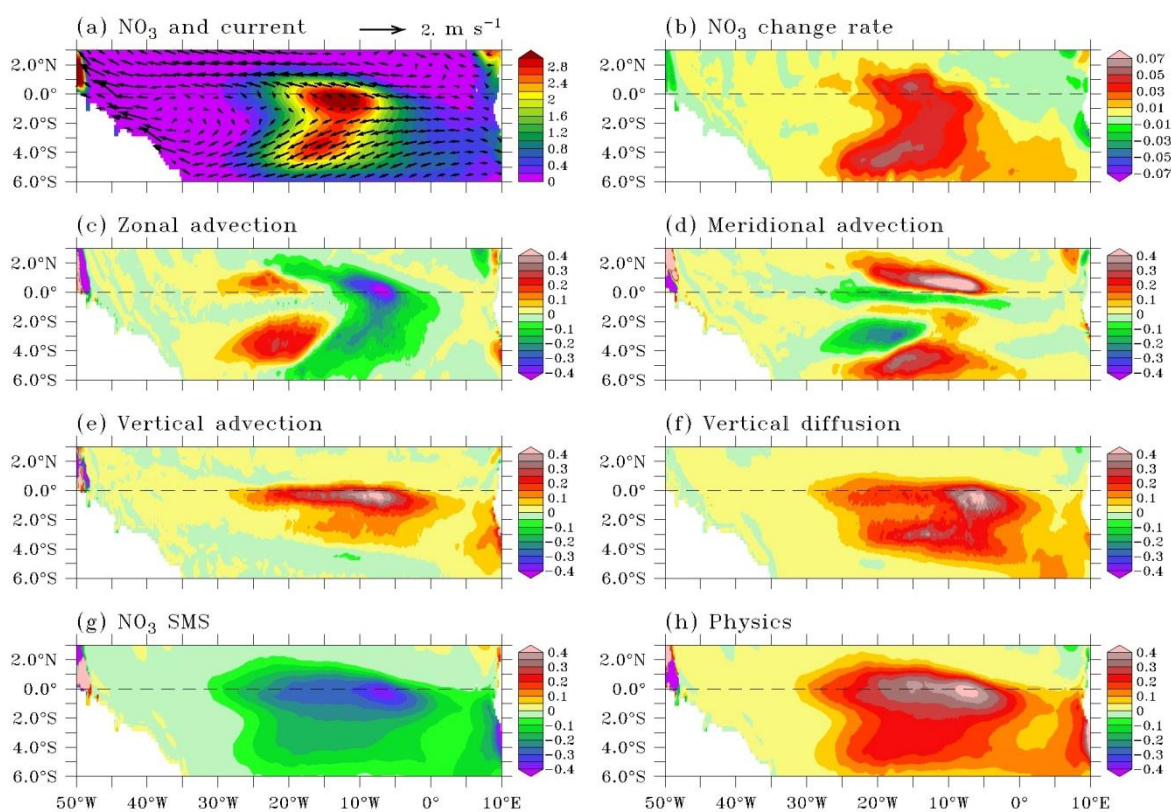
285 Figure 6: Maps of (a) nitrate, (b) nitrate change rate, (c) zonal advection, (d) meridional advection, (e) vertical advection, (f) vertical diffusion, (g) nitrate source minus sink, and (h) physical processes averaged in the mixed layer in July. The mean current in the mixed layer is superimposed in (a). Note that color scale in (b) is different from color scale in (c-h). Nitrate units are \mu\text{mol l}^{-1} and tendency units are \mu\text{mol l}^{-1} \text{day}^{-1} .
