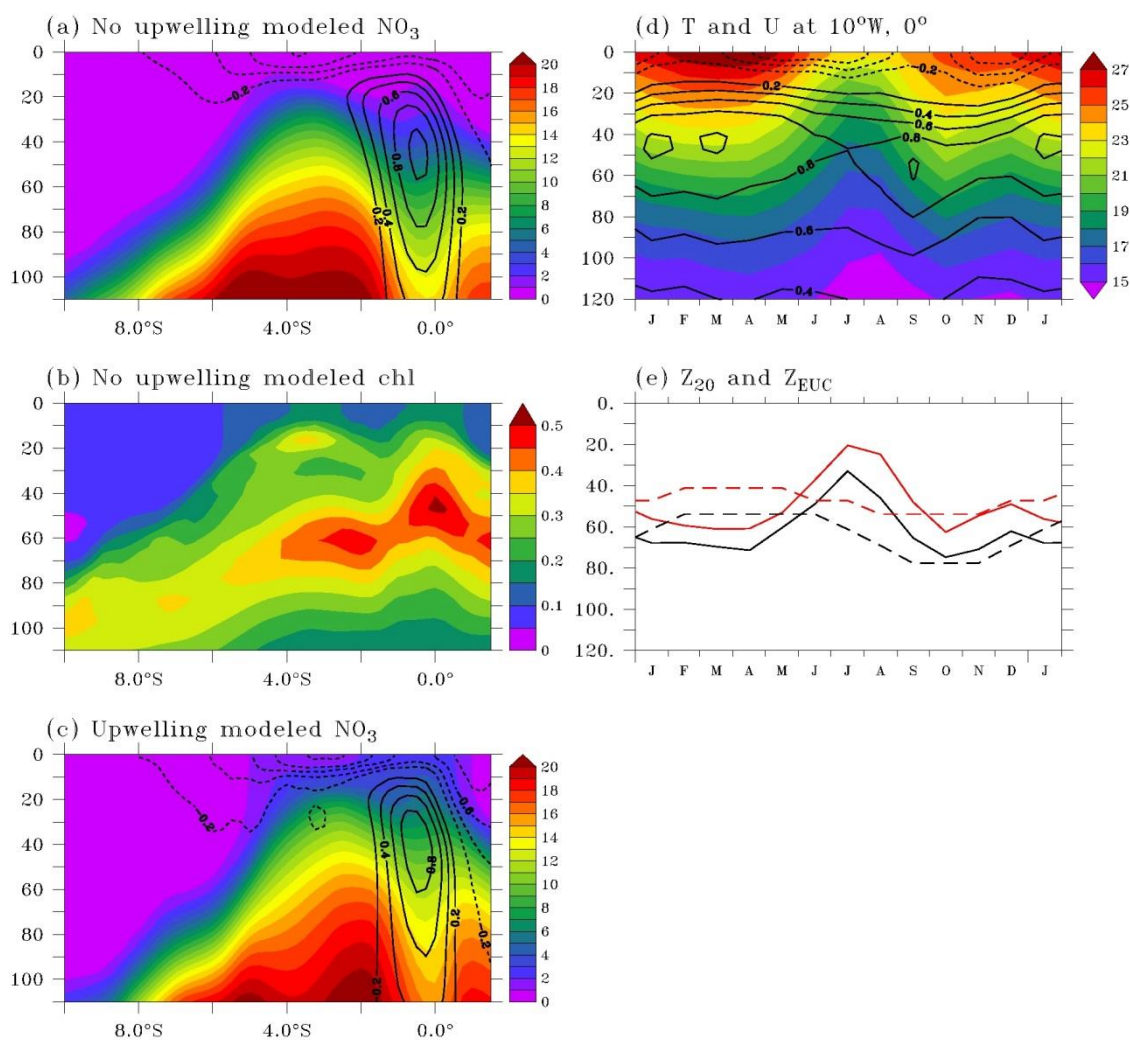
230 Figure 4: (a, c) Simulated nitrate ( \mu\text{mol l}^{-1} ; a, c) and chlorophyll ( \text{mg m}^{-3} ; b) distributions along 10^\circ \text{W} during low productive (a, b) and productive (c) conditions. Zonal velocity is overlaid on nitrate distribution. (d) Seasonal cycles of temperature (colors; ^\circ \text{C} ) and zonal current (contours; \text{m s}^{-1} ) at the 10^\circ \text{W} , 0^\circ \text{N} mooring. Velocity contour interval is 0.2 \text{ m s}^{-1} ; the 0 \text{ m s}^{-1} contour has been removed. (e) Observed (black) and simulated (red) depths of the 20^\circ \text{C} isotherm (full line) and of the EUC core (dashed line) at 10^\circ \text{W} , 0^\circ \text{N} .
