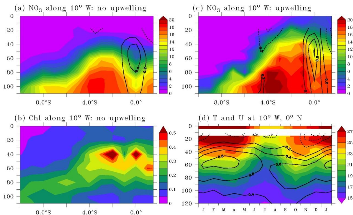
145 Figure 2: (a, c) Observed nitrate ( \mu\text{mol l}^{-1} ; a, c) and chlorophyll ( \text{mg m}^{-3} ; b) distributions along 10^\circ\text{W} during low productive (a, b) and productive (c) conditions. Zonal velocity is overlaid on nitrate distribution. (d) Seasonal cycles of temperature (colors; ^\circ\text{C} ) and zonal current (contours; \text{m s}^{-1} ) at the 10^\circ\text{W} , 0^\circ\text{N} mooring. Velocity contour interval is 0.2\text{ m s}^{-1} ; the 0\text{ m s}^{-1} contour has been removed.
