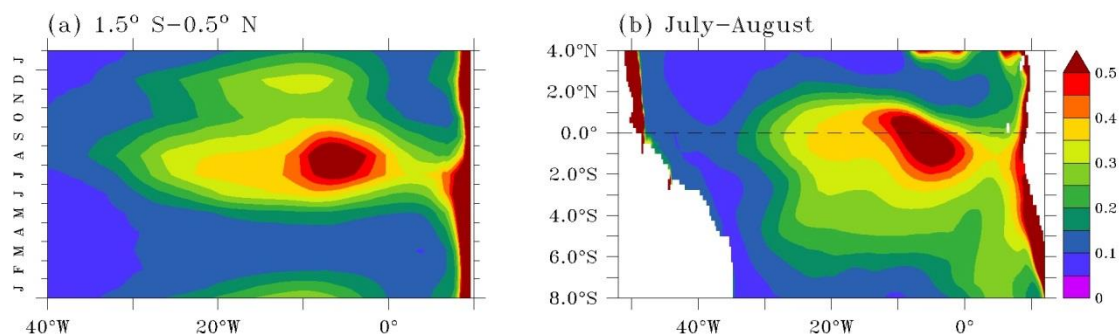
215 Figure 3: Seasonal cycles averaged in 1.5^\circ \text{ S}-0.5^\circ \text{ N} (a) and mean surface distributions in July-August (b) of the simulated chlorophyll ( \text{mg m}^{-3} ; colors). The climatology is calculated over 1998-2015.
