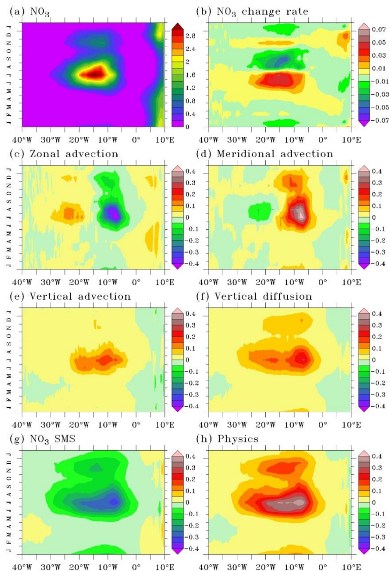
265 Figure 5: Seasonal cycle of modeled (a) surface nitrate ( \mu\text{mol l}^{-1} ), (b) nitrate change rate, (c) zonal advection, (d) meridional advection, (e) vertical advection, (f) vertical diffusion, (g) nitrate source minus sink, and (h) physical processes averaged in 1.5^\circ\text{S} - 0.5^\circ\text{N} in the mixed layer. Tendency units are \mu\text{mol l}^{-1}\text{day}^{-1} . Note that the color scale of nitrate change rate is different from the color scale of other tendencies. Climatology has been calculated between 1995 and 2015.
