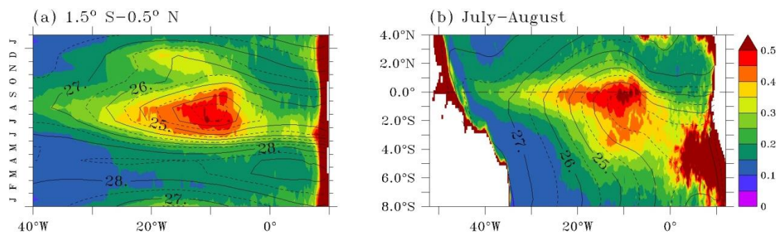
45 Figure 1: Seasonal cycles averaged in 1.5^\circ \text{ S} - 0.5^\circ \text{ N} (a) and mean surface distributions in July-August (b) of satellite chlorophyll ( \text{mg m}^{-3} ; colors) and observed SST ( ^\circ \text{ C} ; contours). The SST contour interval is 0.5^\circ \text{ C} . Chlorophyll and SST climatologies are calculated over 1998-2015. See the data section for origin of data.
