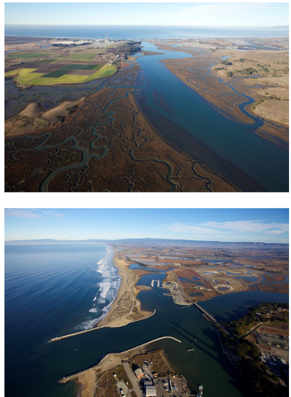
Fig. 1. Elkhorn Slough estuary. Top: View to West, of lower main channel and surrounding marshes. Bottom: View to Northeast, showing Moss Landing Harbor and the artificial mouth to the estuary constructed and maintained to support it. (Photos by K. Ellenbogen.)
