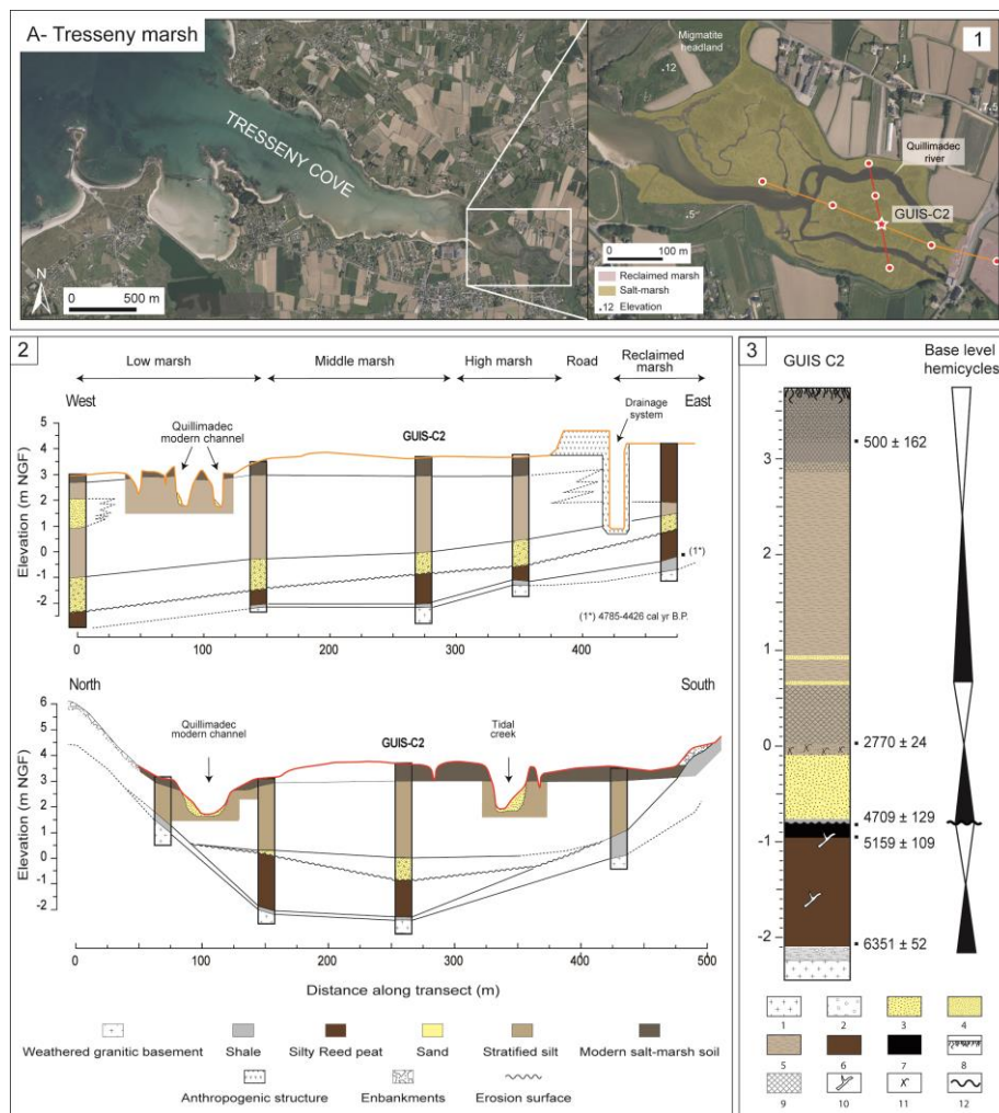
361 362 Figure 2 - 1) Map of the Tressény marsh (noted A on Fig.1) showing the location of the coring transects. The red 363 star locates the GUI-C2 sampled core. 2) Detailed stratigraphy from coring transects taken through the marsh 364 (adapted from Stéphan et al. , 2014), (1*) is an informative dating taken from Stéphan et al. (2014) and unused in 365 this study. 3) Complete stratigraphic log of the GUI-C2 core. 1- Weathered granite basement, 2- Angular gravels 366 and pebbles, 3- Coarse sand, 4- Fine sand, 5- Laminated silt dominated minerogenic deposit, 6- Silty Reed peat, 367 7- Black peat, 8- Humic soil horizon, 10- wood fragments, 11- fragmented shells, 12- Erosion surface.
