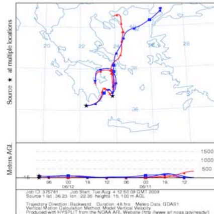
T18 NOAA HYSPLIT MODEL Backward trajectories ending at 0900 UTC 12 Jun 06 GDAS Meteorological Data
