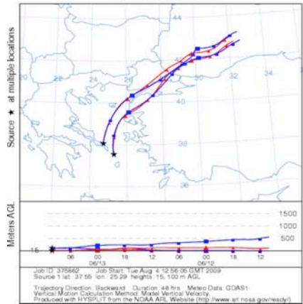
T20 NOAA HYSPLIT MODEL Backward trajectories ending at 1000 UTC 13 Jun 06 GDAS Meteorological Data
