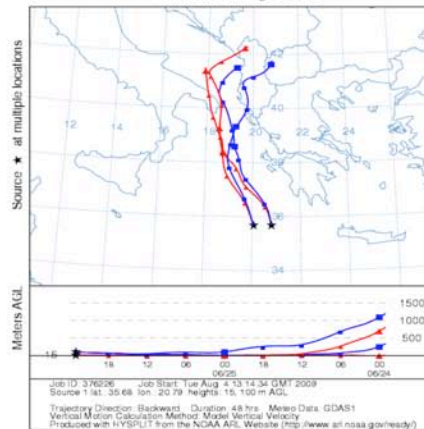
STIIib NOAA HYSPLIT MODEL Backward trajectories ending at 2300 UTC 25 Jun 06 GDAS Meteorological Data
