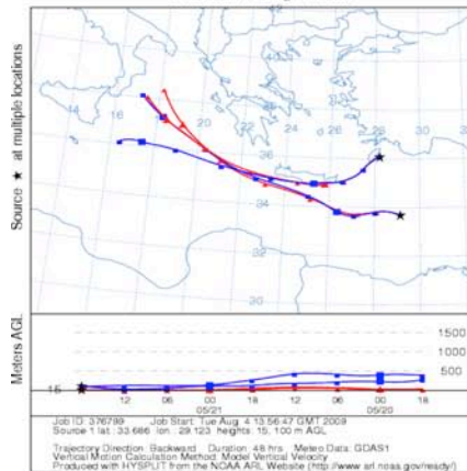
T17 NOAA HYSPLIT MODEL Backward trajectories ending at 1800 UTC 21 May 07 GDAS Meteorological Data
