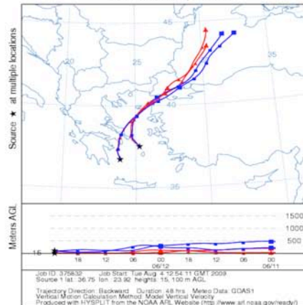
T19 NOAA HYSPLIT MODEL Backward trajectories ending at 2300 UTC 12 Jun 06 GDAS Meteorological Data
