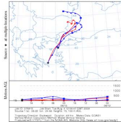
T21 NOAA HYSPLIT MODEL Backward trajectories ending at 2300 UTC 13 Jun 06 GDAS Meteorological Data
