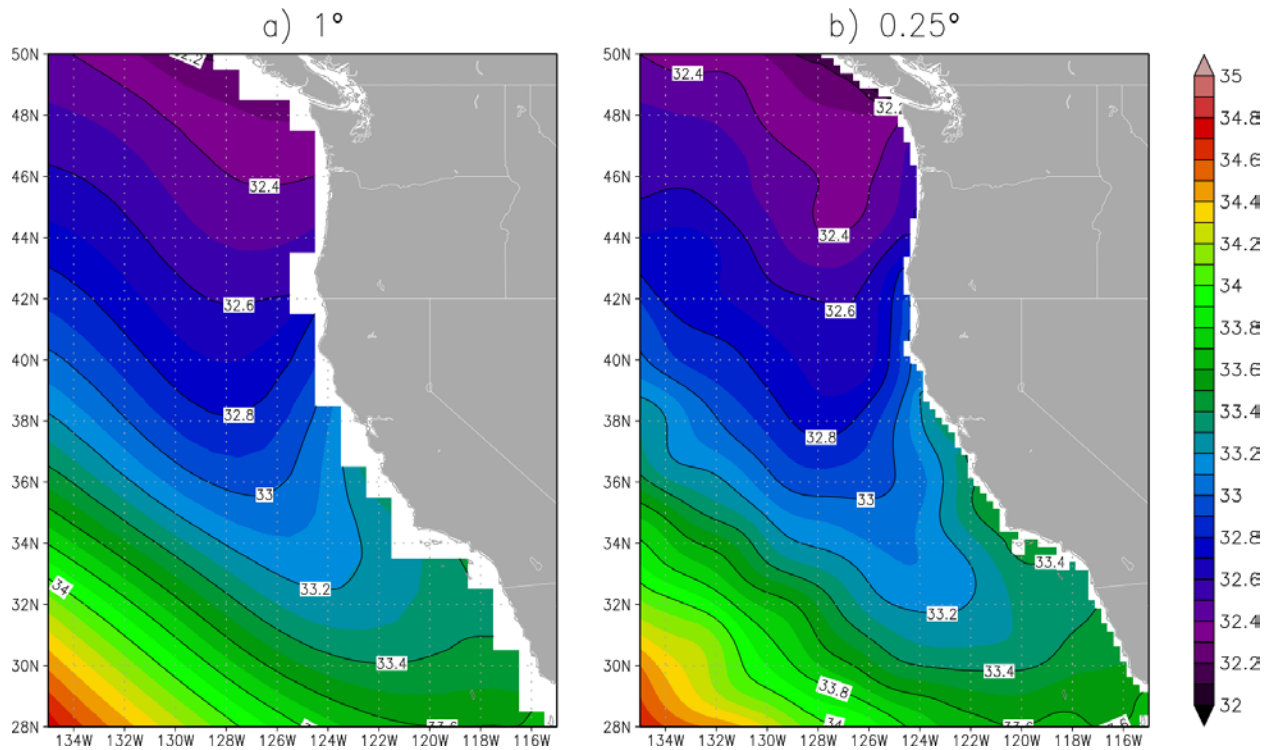
Figure 1. The annual salinity of the California Current at 30m depth for the 1955 - 1964 decade as represented by one-degree resolution and quarter-degree resolution.
