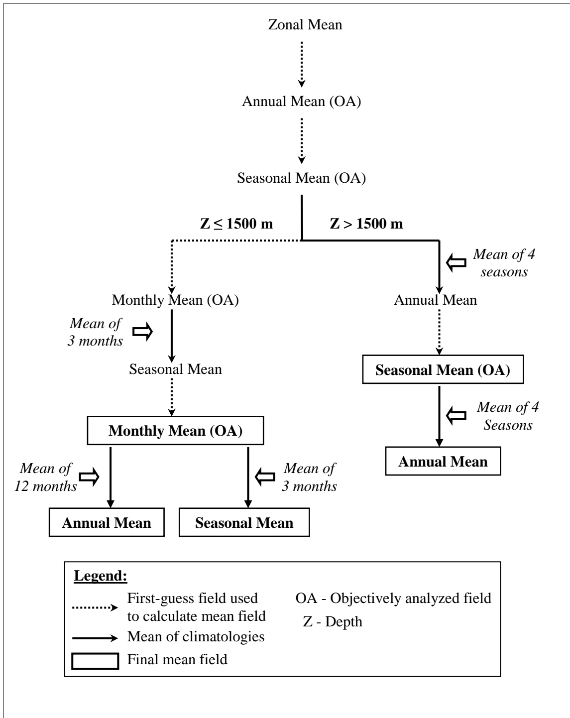
Figure 3. Scheme used in computing “all-data” annual, seasonal, and monthly objectively analyzed means for salinity.
