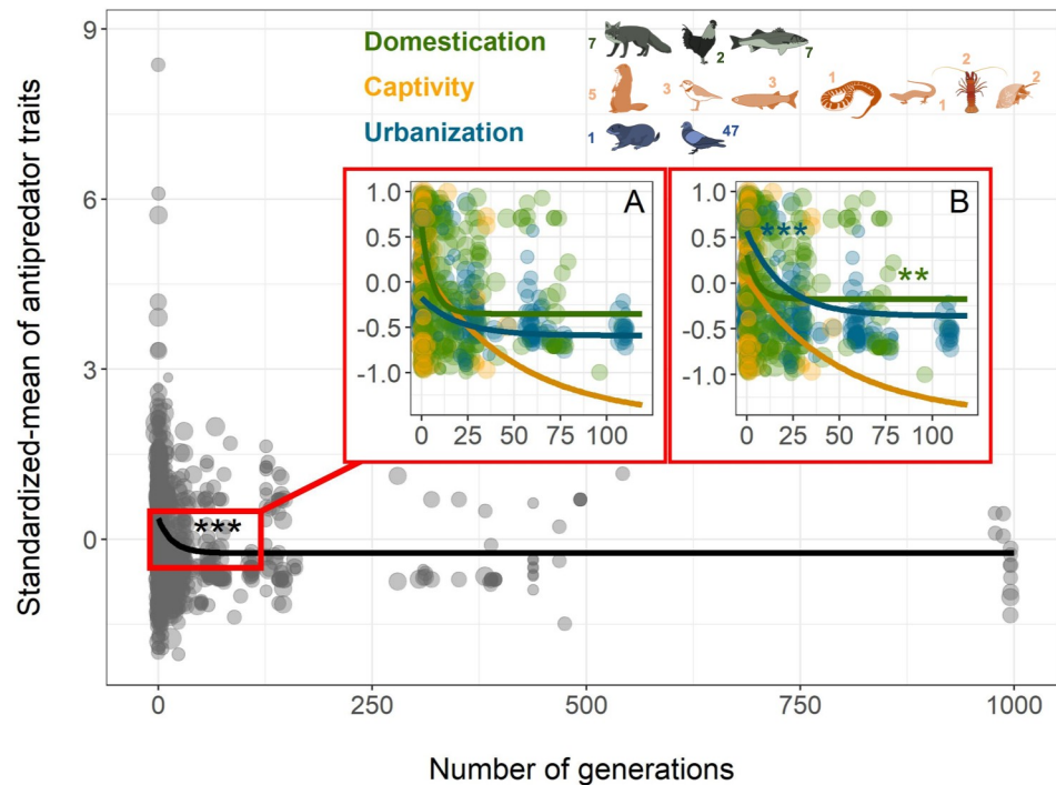
Fig 1. In multiple species, interactions with humans reduce the overall mean of antipredator traits over time, black line (all contexts). (A) Lines correspond to the best inverse model fitting the data using the cma-es function. (B) Lines correspond to the best inverse model with the outputs (slopes and intercepts) of the MCMCglmm model for the mean. Dot size is proportional to the log-transformed number of replicates used in each study. “***” indicates significant p -value < 0.001 and “**” significant p -value < 0.01 of the inverse slopes with the MCMCglmm model (S1 Table). The number associated with each animal indicates the number of species in each of the following taxa: Mammals, Birds, Reptiles, Fish, Amphibians, Arthropods, and Mollusks. All data and R code supporting the figure are available in S1C Data . Species design: Pierre Lopez (MARBEC). cma-es , covariance matrix adapting evolutionary strategy; MARBEC, Marine Biodiversity, Exploitation and Conservation; MCMCglmm, Markov chain Monte Carlo generalized linear mixed model.
