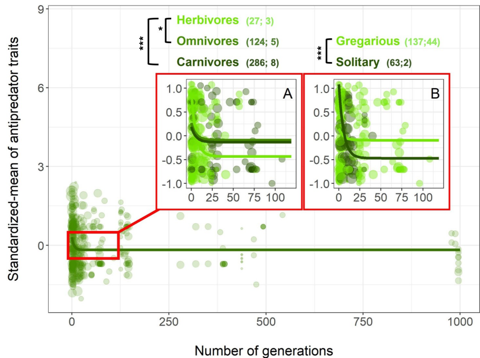
Fig 3. The decrease in average antipredator traits over generations of domestication differs as a function of animal's foraging type (A) and social status (B). The lines represent the best inverse model with the outputs (slopes and intercepts) of the MCMCglmm. In (A), model was fitted with foraging type \times generation interaction. In (B), model was fitted with social status \times generation interaction. Dot size is proportional to the log-transformed number of replicates used in each study. The number in brackets represents the number of estimates followed by the number of species. "***" indicates significant p -value < 0.05 and "****" significant p -value < 0.001 between slopes within each life-history trait using the MCMCglmm model (S3 Table). All data and R code supporting the figure are available in S1C Data . MCMCglmm, Markov chain Monte Carlo generalized linear mixed model.
