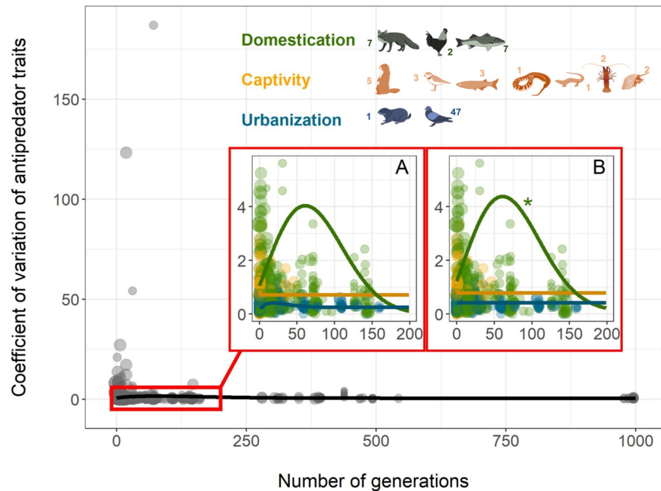
Fig 2. Effects of human presence over time on the CV in antipredator traits, black line (all contexts). (A) Lines correspond to the best loess fitting the data using the cma-es function. (B) Lines correspond to the best Weibull model with the outputs (slopes and intercepts) of the MCMCglmm for the CV. Dot size is proportional to the log-transformed number of replicates used in each study. “*” indicates significant p -value < 0.05 of the Weibull slopes with the MCMCglmm model (S1 Table). The number associated with each animal indicates the number of species in each of the following taxa: Mammals, Birds, Reptiles, Fish, Amphibians, Arthropods, and Mollusks. All data and R code supporting the figure are available in S1C Data. Species design: Pierre Lopez (MARBEC). cma-es , covariance matrix adapting evolutionary strategy; CV, coefficient of variation; MARBEC, Marine Biodiversity, Exploitation and Conservation; MCMCglmm, Markov chain Monte Carlo generalized linear mixed model.
