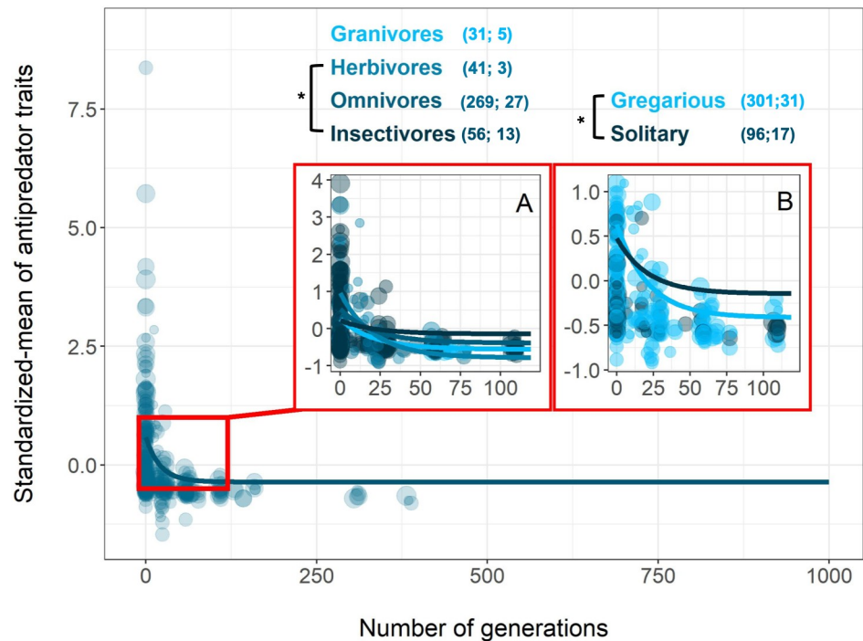
Fig 4. The decrease in average antipredator traits over generations of urbanization differs according to an animal's foraging type (A) and its social status (B). The lines represent to the best inverse model with the outputs (slopes and intercepts) of the MCMCglmm. In (A), model was fitted with foraging type \times generation interaction. In (B), model was fitted with social status \times generation interaction. Dot size is proportional to the log-transformed number of replicates used in each study. The number in brackets represents the number of estimates followed by the number of species. “*” indicates significant p -value < 0.05 between slopes within each life-history trait using the MCMCglmm model (S3 Table). All data and R code supporting the figure are available in S1C Data . MCMCglmm, Markov chain Monte Carlo generalized linear mixed model.
