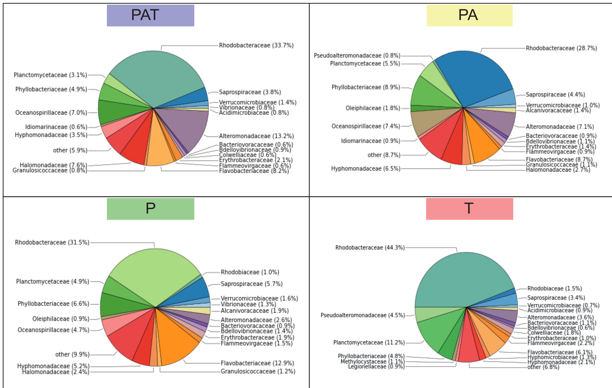
Figure S7 Pie Chart of bacteria families in each assemblage. PAT: P. damicornis , A. cytherea , T. maxima ; PA: P. damicornis , A. cytherea ; P: P. damicornis ; T: T. maxima .
