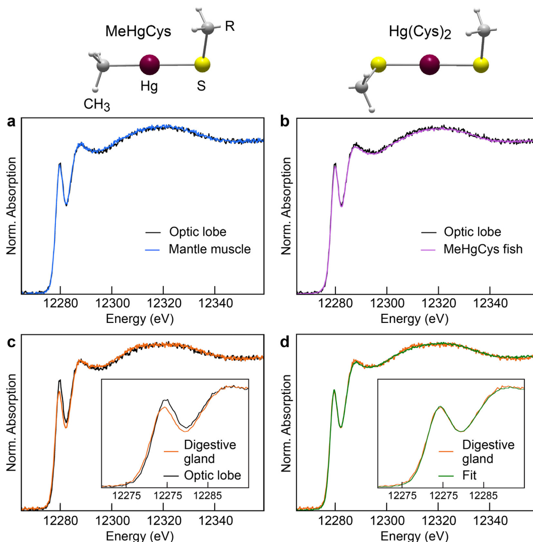
Fig. 3. Chemical forms of Hg determined by Hg L_3 -edge HR-XANES spectroscopy and ball-and-stick representation of the MeHgCys and Hg(Cys) 2 complexes. a-c) Comparison of the spectrum for the optic lobes with the spectra (a) for the mantle muscle, (b) for MeHgCys in fish muscle, and (c) for the digestive gland. d) Linear combination fit of the spectrum for the digestive gland with 68 \pm 11\% of the optic lobes spectrum and 33 \pm 11\% of the dicysteinate complex Hg(Cys) 2 . NSS = 1.50 \times 10^{-4} .
