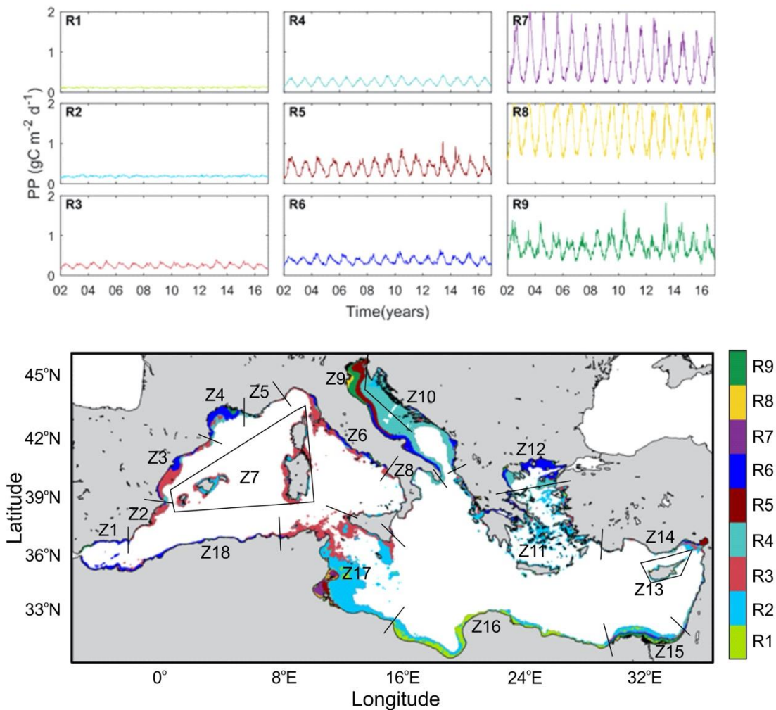
340 Figure 7: Regionalization of the coastal waters in the Mediterranean Sea based on their temporal patterns of pelagic primary production. a) Characteristic temporal patterns of PP obtained from SOM classification (R1 to R9) and b) coastal regions 345 defined from alongshore variations of the SOM – regions (Z1 to Z18).
