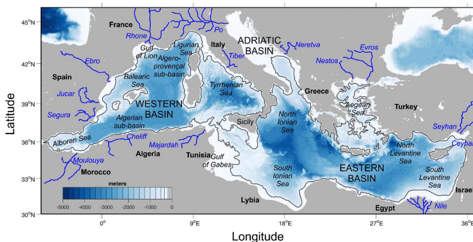
110 Figure 1: Map of the Mediterranean Sea showing the main basins, sea regions, surrounding countries and major rivers. 115 Bathymetric data were obtained from ETOPO1 (Amante and Eakins, 2009). The black contour indicates the 200m isobath, the limit of coastal waters as defined in the present study.
