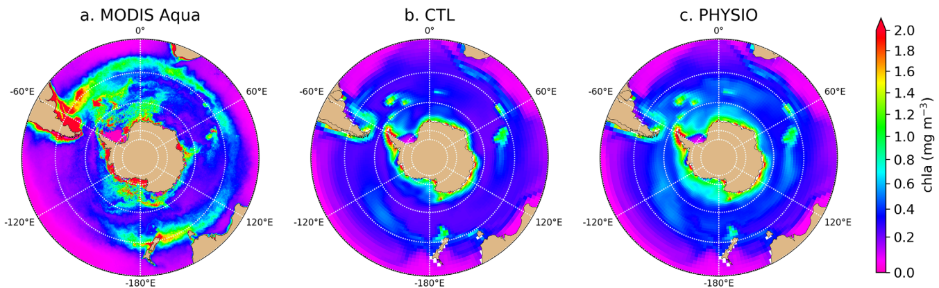
Figure 4. Spatial distribution of the mean surface chlorophyll concentrations in summer (December, January, and February) in the Southern Ocean, south of 30°S, from (a) observations (MODIS-Aqua), (b) the CTL experiment, and (c) the PHYSIO experiment. Annual mean positions of the fronts in the model are shown in both experiments by the black lines: from north to south, the STF, the SAF, and the PF.
