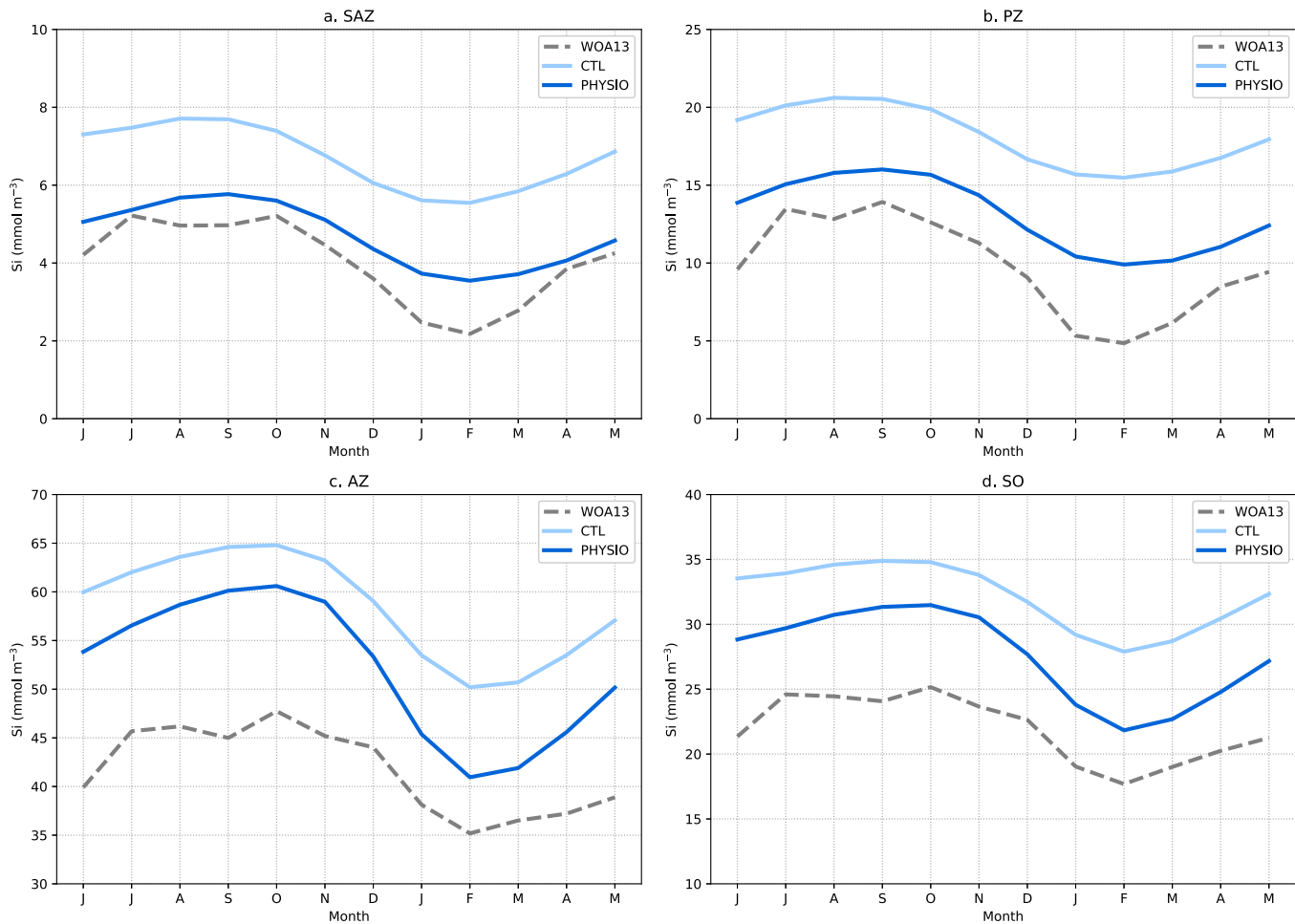
Figure 11. Seasonal cycles from June to May of the surface silicate concentration ( Si , \text{mmol m}^{-3} ) from the World Ocean Atlas 2013 observations climatology (dashed line, gray), the CTL experiment (light blue), and the PHYSIO experiment (dark blue) averaged over (a) the Sub-Antarctic Zone (SAZ), (b) the Polar Zone (PZ), (c) the Antarctic Zone, and (d) the Southern Ocean (SO), south of the subtropical front.
