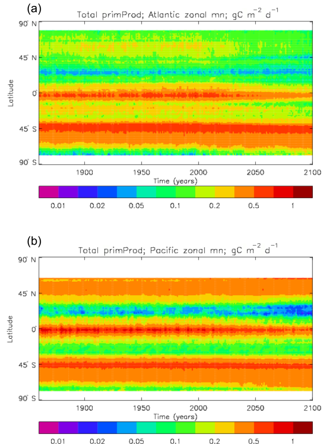
Figure 38. Change in annual mean depth-integrated total primary production ( \text{gC m}^{-2} \text{d}^{-1} ) during the model years 1860 to 2099 in the CMIP5 historical and RCP8.5 simulations. (a) Atlantic Ocean basin zonal mean; (b) Pacific Ocean basin zonal mean.
