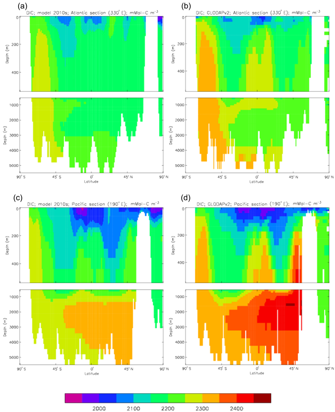
Figure 10. Meridional sections of DIC: panels (a) and (b) show sections in the Atlantic Ocean along 330°; (c, d) Pacific Ocean sections along 190°. Panels (a) and (c) show model concentrations averaged over 2010–2019, and panels (b) and (d) show concentrations from the GLODAPv2 gridded product.
