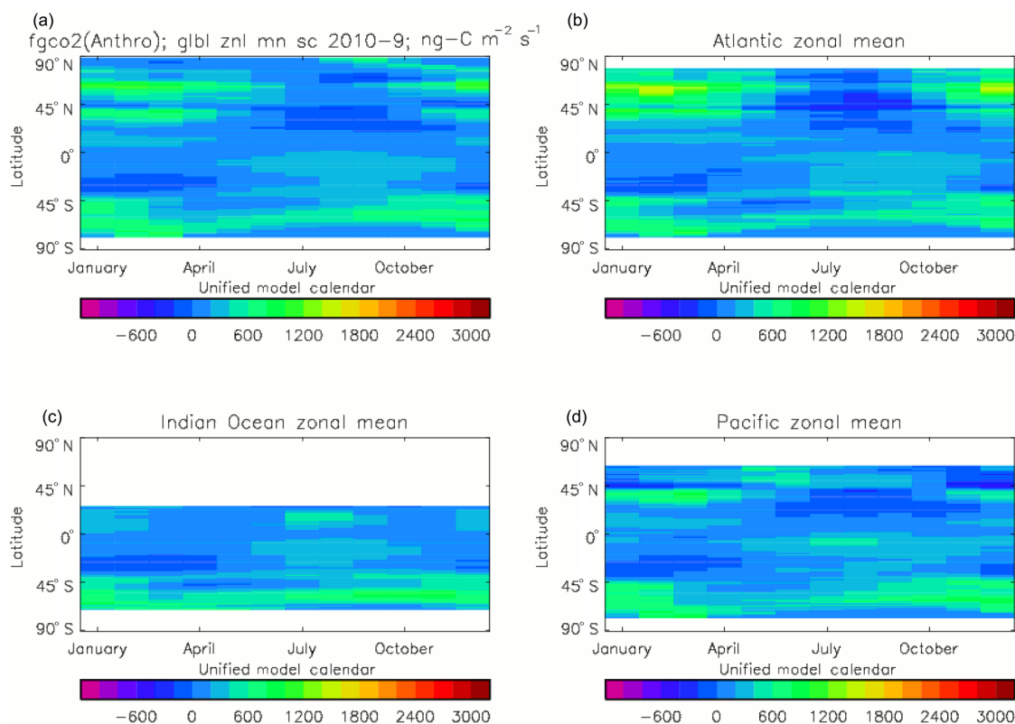
Figure 21. As Fig. 20, but for the air-to-sea flux of anthropogenic CO 2 only (ng C m -2 s -1 ).
