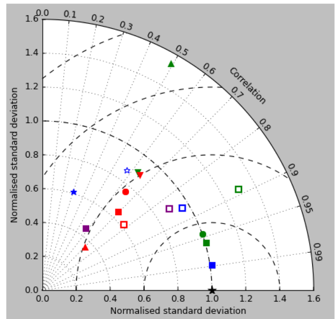
Figure 29. Taylor diagram of nitrate (green), silicate (red), oxygen (blue) and apparent oxygen utilisation (purple); model values are averaged over the years 2010 to 2019, and observations are from the 2013 World Ocean Atlas. Filled squares show the surface concentrations, open squares the concentrations at the nearest depth level to 1050 m, and circles, upward-pointing triangles and downward triangles respectively show the midpoint, amplitude and phase of the sine curve that best fits the seasonal cycle (only at points for which the residual variance is less than half the original). The filled and open stars respectively show the vertical extent of the water column where the O 2 concentration is below 50 and 100 mMol O 2 m -3 .
