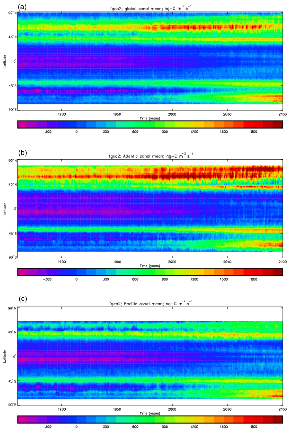
Figure 41. Change in the annual mean total air-to-sea CO 2 flux ( \text{ng C m}^{-2} \text{s}^{-1} ) during model years 1860 to 2099 in the historical and RCP8.5 simulations. (a) Global zonal mean; (b) Atlantic Ocean basin zonal mean; (c) Pacific Ocean basin zonal mean.
