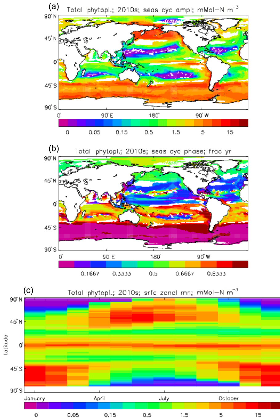
Figure 7. Total phytoplankton surface biomass mean seasonal cycle, averaged over the model years 2010 to 2019. (a) Amplitude ( \text{mMol N m}^{-3} ) and (b) phase (fraction of year when peak value occurs) of the seasonal cycle, determined by the best-fitting sine curve (only points for which the residual variance is less than half that of the original cycle are shown). (c) The global zonal mean for each month ( \text{mMol N m}^{-3} ).
