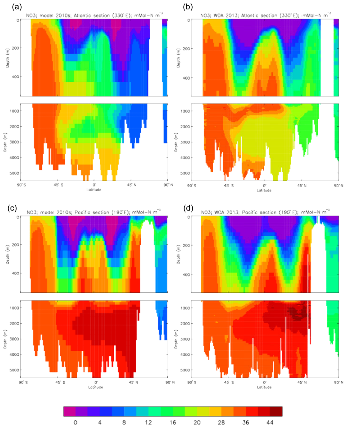
Figure 23. Meridional sections of dissolved nitrate ( \text{mMol N m}^{-3} ): panels (a) and (b) show sections in the Atlantic Ocean along 330^\circ ; (c, d) Pacific Ocean sections along 190^\circ . Panels (a) and (c) show model concentrations averaged over 2010–2019; panels (b) and (d) show concentrations from the 2013 World Ocean Atlas gridded field.
