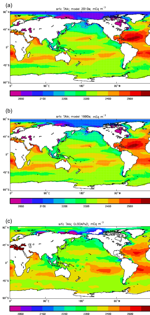
Figure 12. Surface concentration of total alkalinity ( \text{mEq m}^{-3} ): (a) model field averaged over model years 2010–2019; (b) model field averaged over model years 1990–1999; (c) the gridded field from the GLODAPv2 database.
