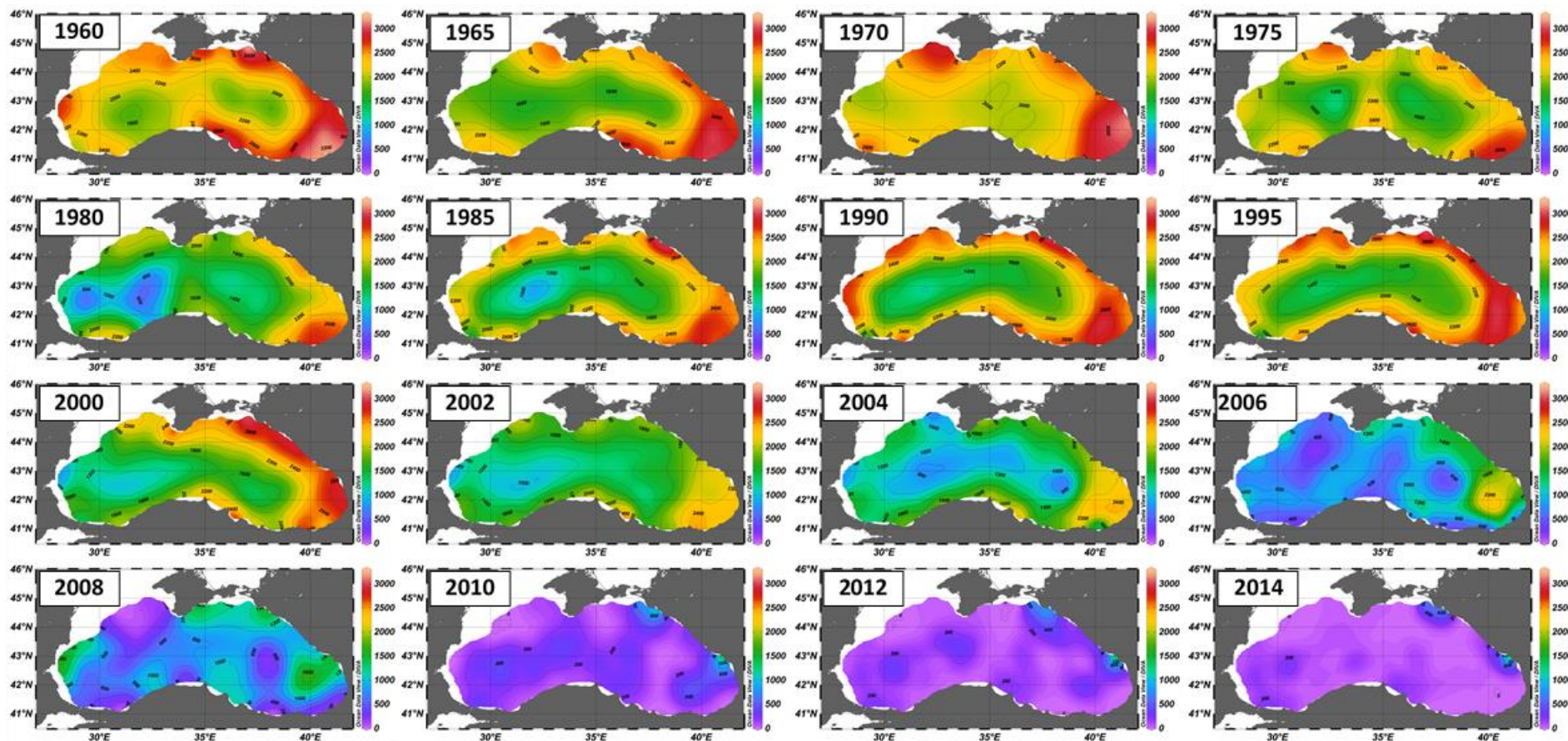
Figure 8 Decadal CCC [ 10^6 \text{ J/m}^2 ] fields (the year on the map indicates the centre of decade)
