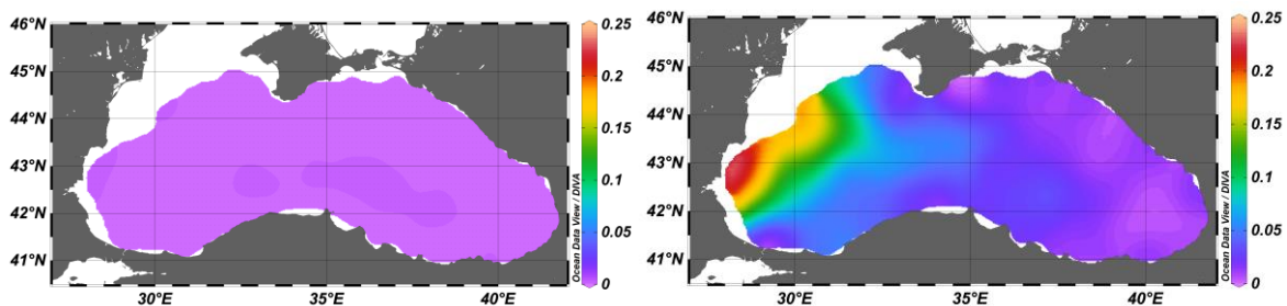
Figure 10 Relative error for CCC field in decade 1985-1994 (left) and 1961-1970 (right)
