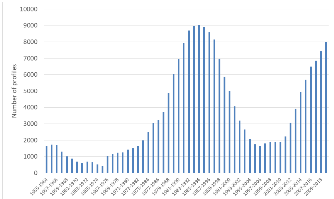
Figure 9 Data availability per decades
