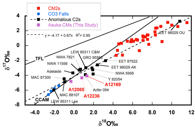
Fig. 10. Oxygen three isotope diagram showing the relationship between the Asuka CMs, anomalous C2 chondrites, “normal” CM2 chondrites and CO3 chondrites. The regression line shown was calculated using only the analyses of anomalous C2 samples. TFL = Terrestrial Fractionation Line. CCAM = Carbonaceous Chondrite Anhydrous Mineral line (Clayton and Mayeda, 1999). Data sources – “normal” CM2s: Clayton and Mayeda (1999); Haack et al. (2012); Hewins et al. (2014), CO3 chondrite falls: Alexander et al. (2018); Anomalous C2 chondrites Clayton and Mayeda (1999); with the exception of: EET 85311 “OU” and EET 85311 “AK” (Lee et al., 2016); LEW 85311 “Lee” (Lee et al., 2019); NWA 5958 (Jacquet et al., 2016).
