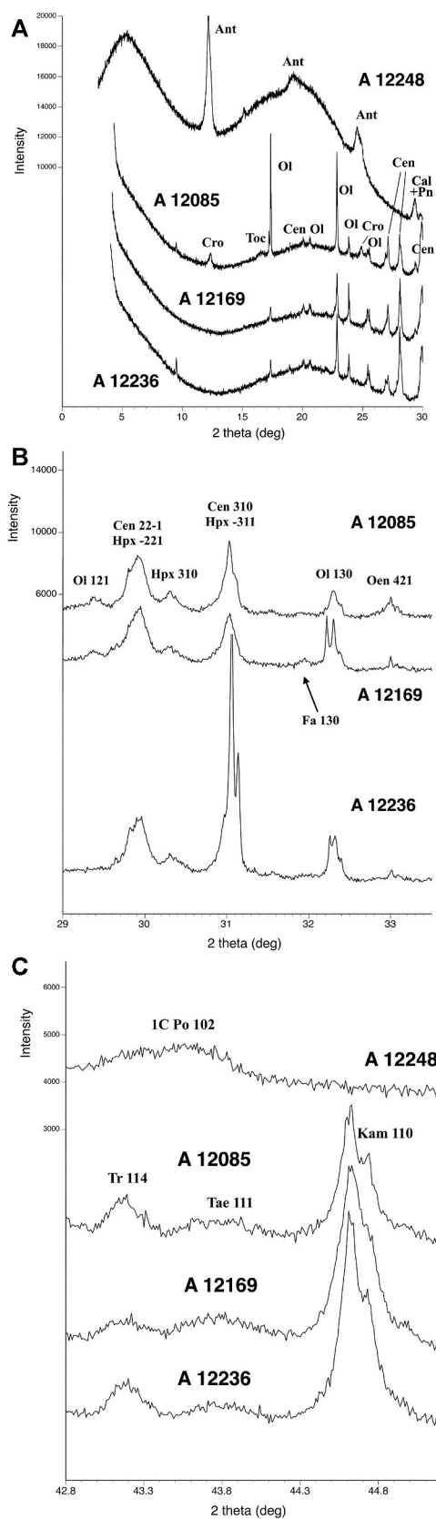
Fig. 7. (a) X-ray diffraction of 2 theta, 0–30° for the Asuka chondrites, in comparison with A 12248 (CM2.0). (b) Diffraction of 2 theta, 29–33.5°. (c) Diffraction of 2 theta, 42.8–45.2°. Ant = antigolite, Cro = cronstedtite, Cen = clinoenstatite, Fa = fayalitic olivine, Kam = kamacite, Oen = orthoenstatite, Tae = taenite, Toc = tochilinite, and Tr = troilite.
