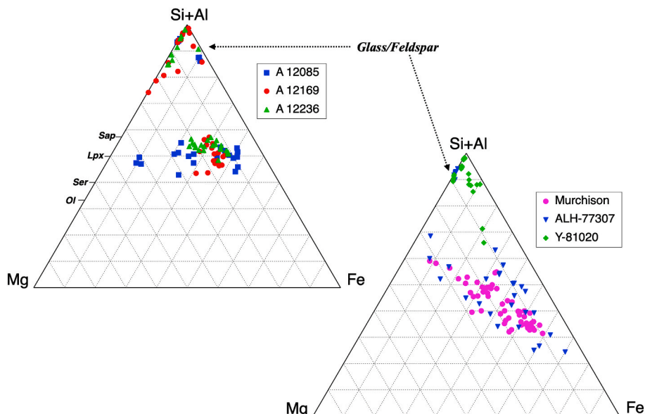
Fig. 4. The mesostasis composition on (Si + Al)-Mg-Fe diagram (atomic ratio) for the Asuka chondrites and other CM and CO chondrites.
