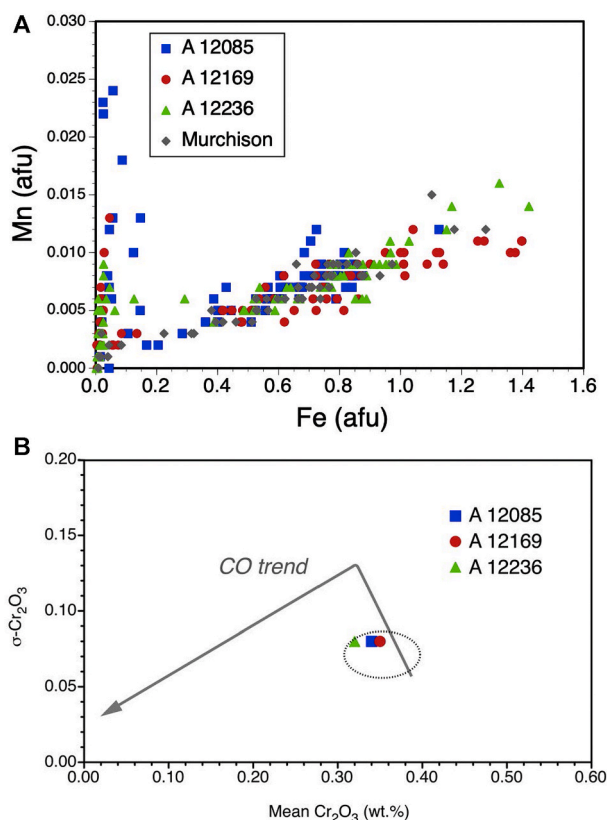
Fig. 3. Olivine compositions. (a) Fe vs. Mn plot of olivine from the Asuka chondrites, in comparison with that of Murchison (CM2.5). (b) Mean \text{Cr}_2\text{O}_3 vs. \sigma\text{-Cr}_2\text{O}_3 plot in ferroan olivine for Asuka chondrites. The diagram and CO trend are after Grossman and Brearley (2005) and Schrader and Davidson (2017). A dotted circle shows the area of CO3.0 and CM chondrites.
