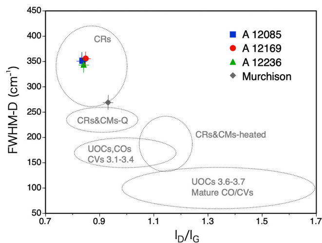
Fig. 8. Spectral parameters of Raman bands of carbonaceous matter from the matrix of the Asuka chondrites and Murchison. Dotted areas summarize data from the other chondrites. CRs, COs, CVs, and UOCs are after Komatsu et al. (2018). CMs-B is after Buseman et al. (2007), and CRs&CMs-Q is after Quirico et al. (2014).
