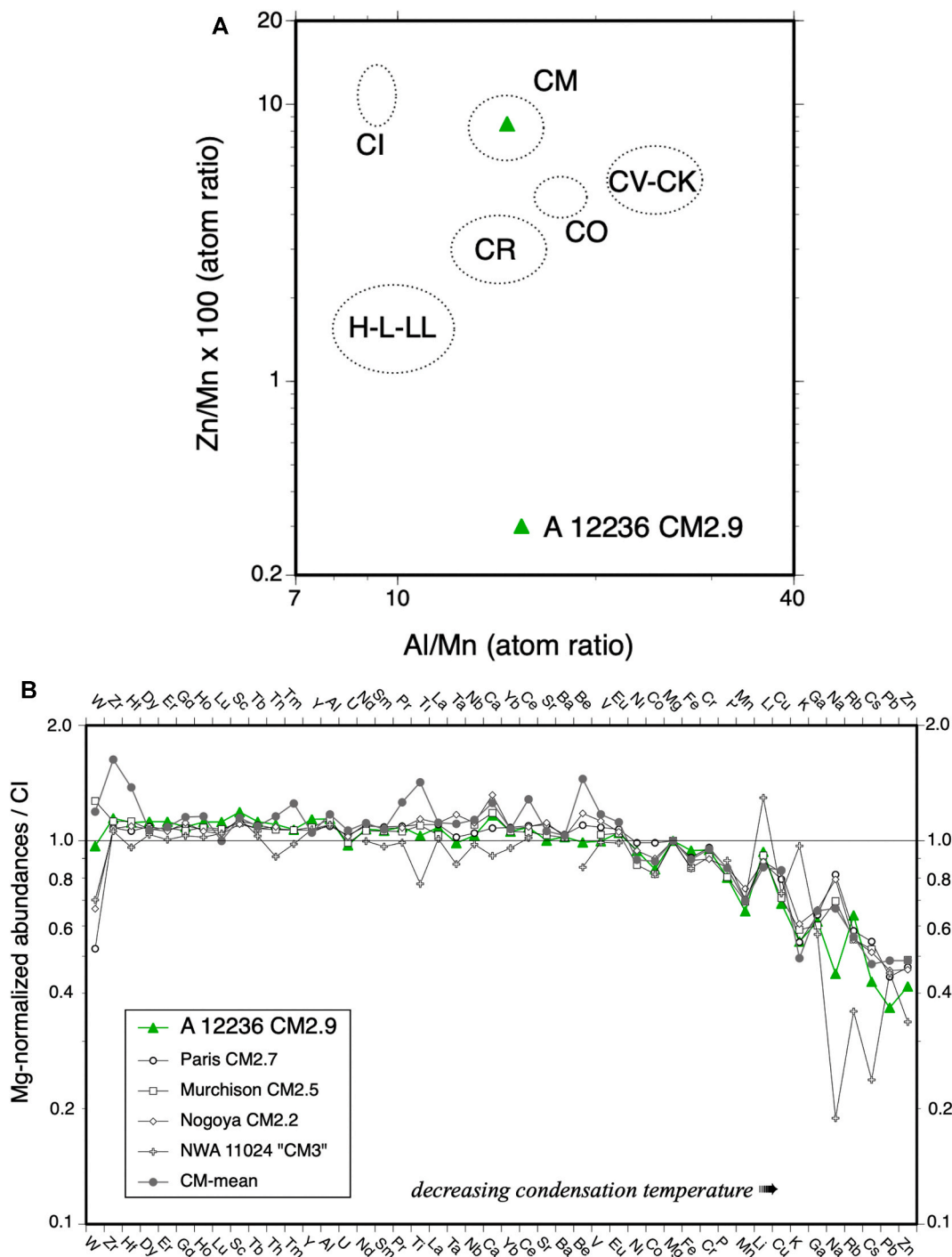
Fig. 9. (a) Al/Mn versus (Zn/Mn)×100 atomic ratios of the Asuka chondrites. Dotted areas for chondrites are after Krot et al. (2014) . (b) The CI-normalized bulk composition of A 12236 (CM2.9), compared with those of Paris (CM2.7), Murchison (CM2.5), Nogoya (CM2.2), NWA 11024 (dehydrated CM), and CM-mean. The data of Paris and Nogoya are after Hewins et al. (2014) , Murchison after Wolf and Palme (2001) and Hewins et al. (2014) , NWA 11024 after Ebert et al. (2019) , and CM-mean after Lodders and Fegley (1998) . In NWA 11024, the data of Sr, Ba, and U, are not plotted because of terrestrial weathering effect ( Stelzner et al., 1999 ). The condensation temperatures for elements are after Lodders and Fegley (1998) .
