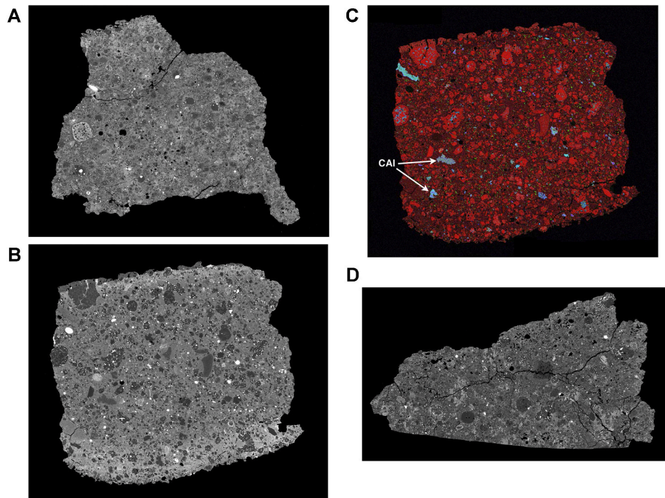
Fig. 1. Backscattered electron (BSE) images of (a) A 12085, 41-1 (width of sample 12.8 mm), showing chondrules among matrix, (b) A 12169, 31-1 (6.7 mm), containing fusion crusts in both sides of the section (gray areas), and (c) combined elemental (Mg-Ca-Al) map of A 12169 showing CAIs, and (d) BSE image of A 12236, 51-1 (12.6 mm).
