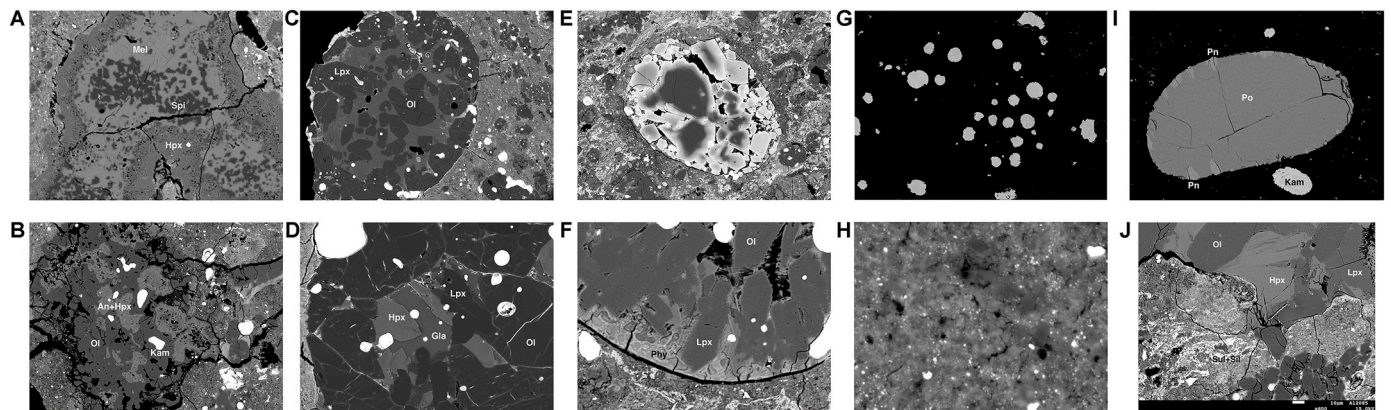
Fig. 2. BSE images of constituent components. (a) A melilite (Mel)-rich CAI with spinel (Sp) and high-Ca pyroxene (Hpx) in A 12169. The width is 210 \mu\text{m} . (b) An AOA, consisting of forsteritic olivine (Ol) with interstitial anorthite and high-Ca pyroxene (An + Hpx) and kamacite (Kam) in A 12236. The width is 280 \mu\text{m} . (c) A Type I chondrule in A 12169, mainly consisting of phenocrysts of olivine and low-Ca pyroxene (Lpx), among feldspathic mesostasis (light gray). The width is 0.76 mm. (d) A Type I chondrule in A 12169 consisting of olivine, low- and high-Ca pyroxene, and glassy mesostasis (Gla). The width is 240 \mu\text{m} . (e) A type II chondrule in A 12085, consisting of ferroan olivine with abundant relict forsteritic olivine (dark), surrounded by fine-grained rim. The width is 0.65 mm. (f) A peripheral part of type I chondrule in A 12085. Mesostasis is replaced by phyllosilicate (Phy). The width is 170 \mu\text{m} . (g) Homogeneous kamacite spherules in a type I chondrule of A 12236. The width is 210 \mu\text{m} . (h) A matrix area of A 12169, consisting of very fine-grained silicate phases with abundant sulfide of submicron in size (bright). The width is 20 \mu\text{m} . (i) A sulfide grain in A 12169, consisting of pyrrhotite (Po) with small amounts of pentlandite (Pn). The width is 190 \mu\text{m} . (j) A type I chondrule and matrix area of A 12085, including fine-grained aggregates of Fe-sulfide with silicate phases (Sul + Sil). The width is 210 \mu\text{m} .
