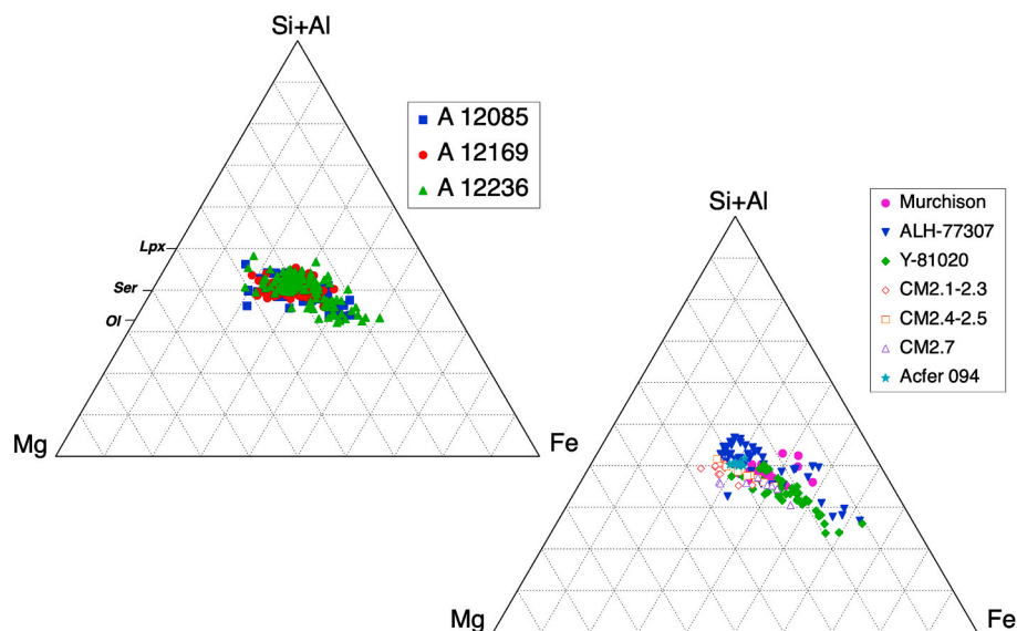
Fig. 6. Matrix compositions of the Asuka chondrites in atomic (Si + Al)–Mg–Fe plot, compared with other CMs, COs, and Acfer 094 (this work; Metzler et al., 1992; Zolensky et al., 1993; Marrocchi et al., 2014; Wasson and Rubin, 2010).
