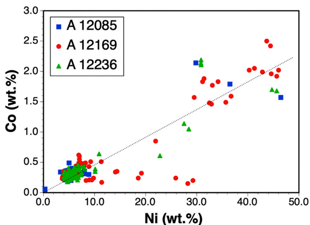
Fig. 5. Ni vs. Co (wt.%) plot of Fe–Ni metal grains in the Asuka chondrites. The dotted line shows the CI chondritic Co/Ni ratio after Anders and Grevesse (1989).
