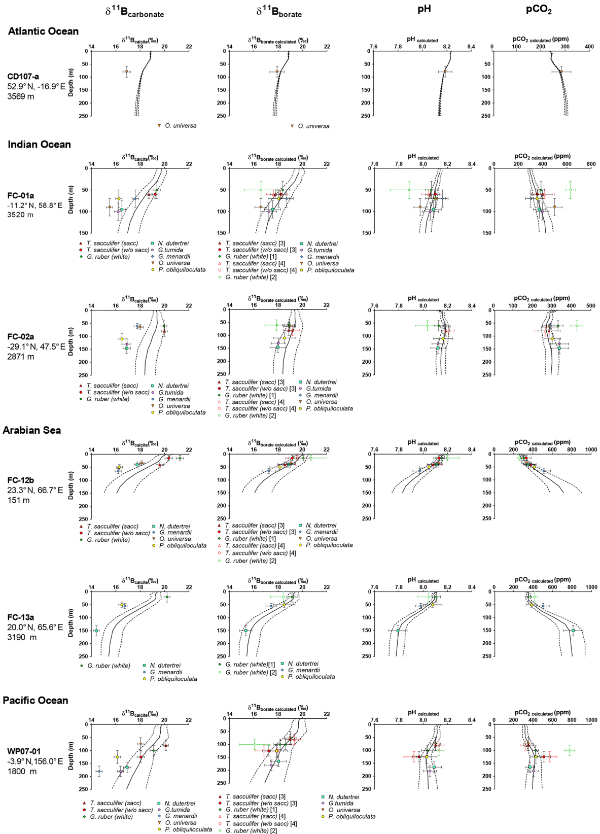
Figure 8. Water depth pH profiles reconstructed at every site applying the monospecific calibrations derived from our results (Table 3). The figure shows measured \delta^{11}\text{B}_{\text{carbonate}} , \delta^{11}\text{B}_{\text{borate}} calculated according to different calibrations (see Table 3 and text), calculated pH based on \delta^{11}\text{B} ( \text{pH}_{\delta^{11}\text{B}} ), and \text{pCO}_2 calculated from \text{pH}_{\delta^{11}\text{B}} and alkalinity.
