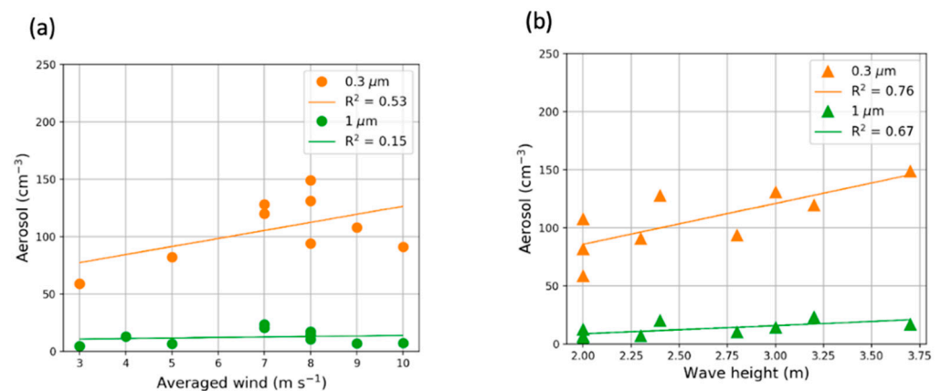
Figure 16. Aerosol concentrations (diameter >0.3 \mu\text{m} and >1.0 \mu\text{m} ) measured during the BOREAL flights as a function of (a) the averaged horizontal wind in the marine boundary layer and (b) the measured wave height.
