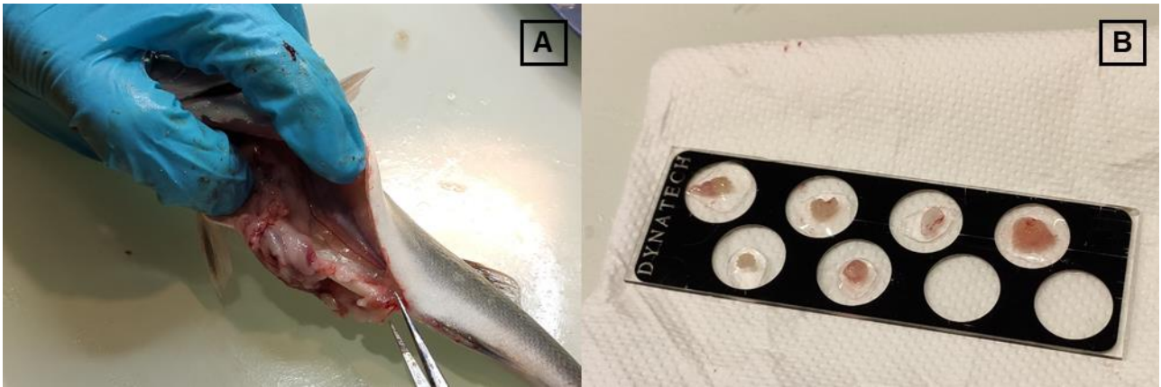
Fig. S2. Determination of the sex of 358 dph (3229 degree days above 10 °C) fish, either through macroscopically observation of the gonads (A) or gonadal squash (B) following Menu et al. (2005).
