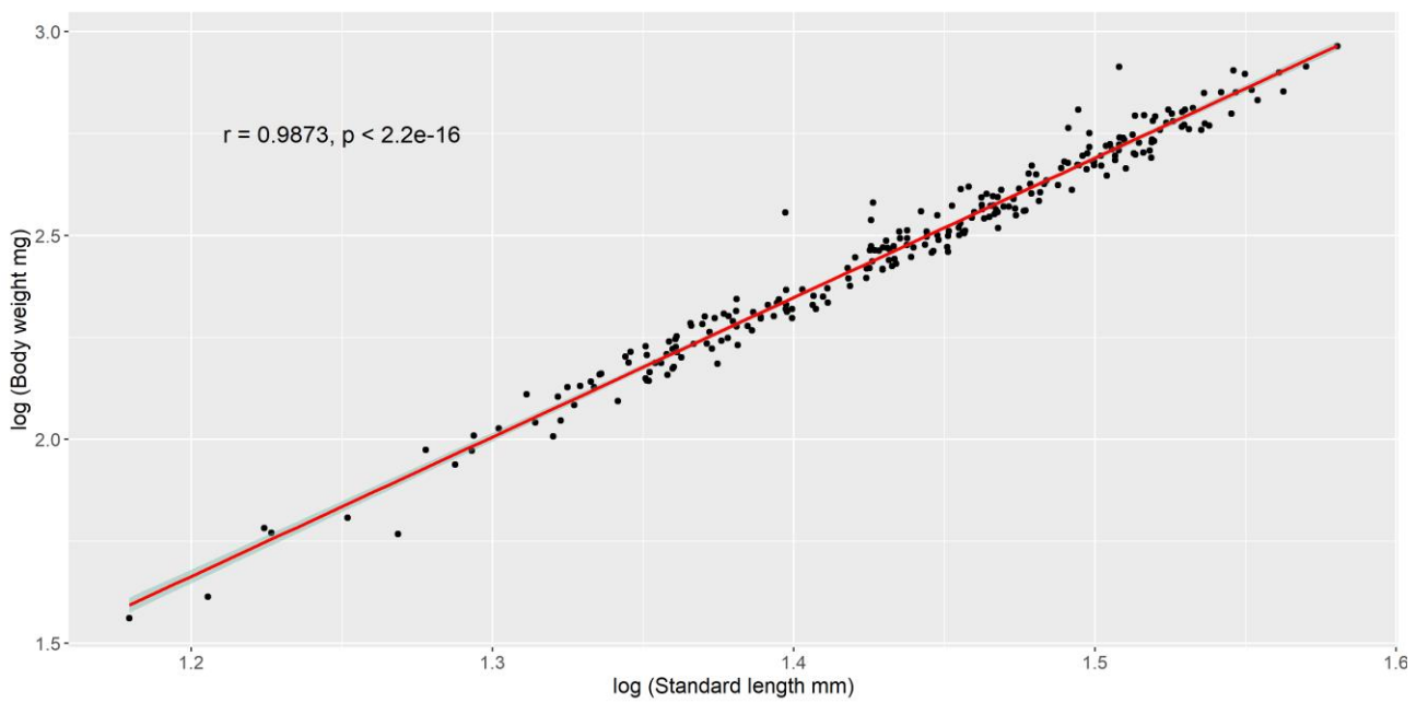
Fig. S4. Regression between logarithm of the measured standard length and logarithm of the measured body weight.
