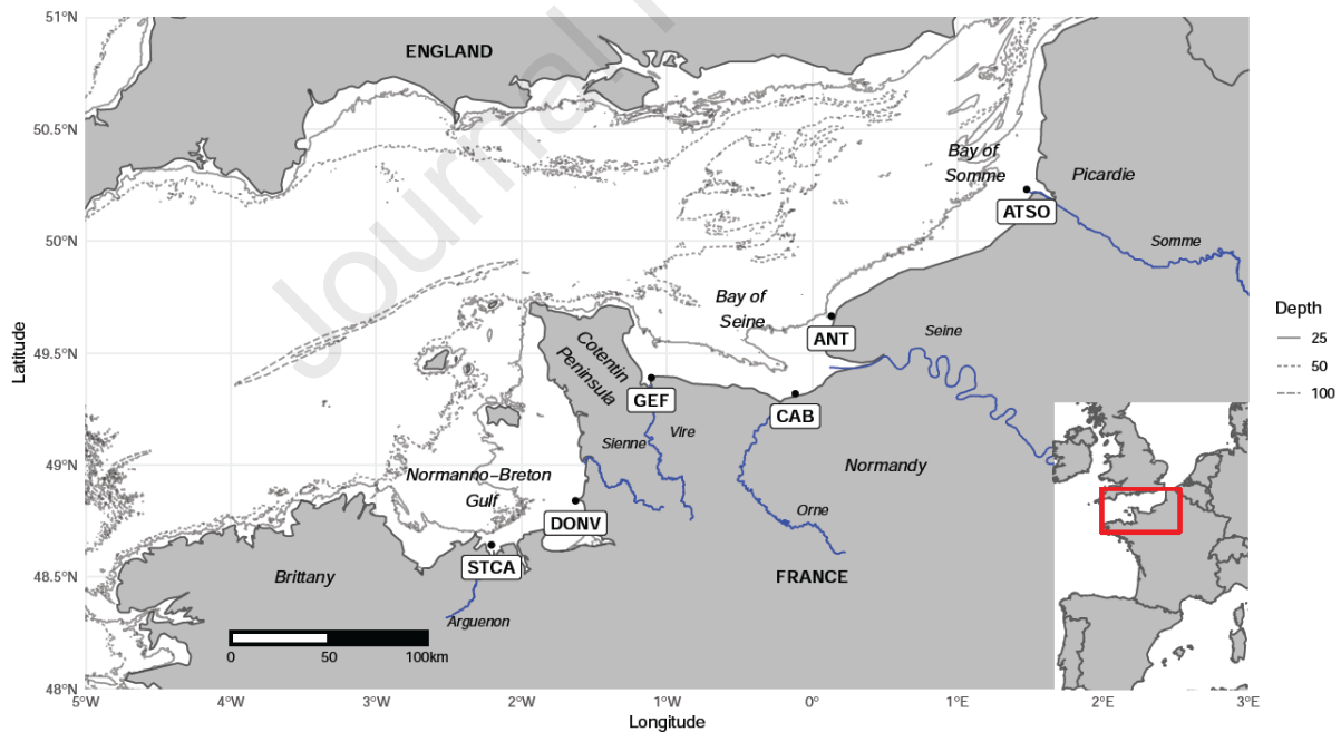
Figure 1 : Study area: The Eastern English Channel. (R package : naturalearth (South, 2020))
