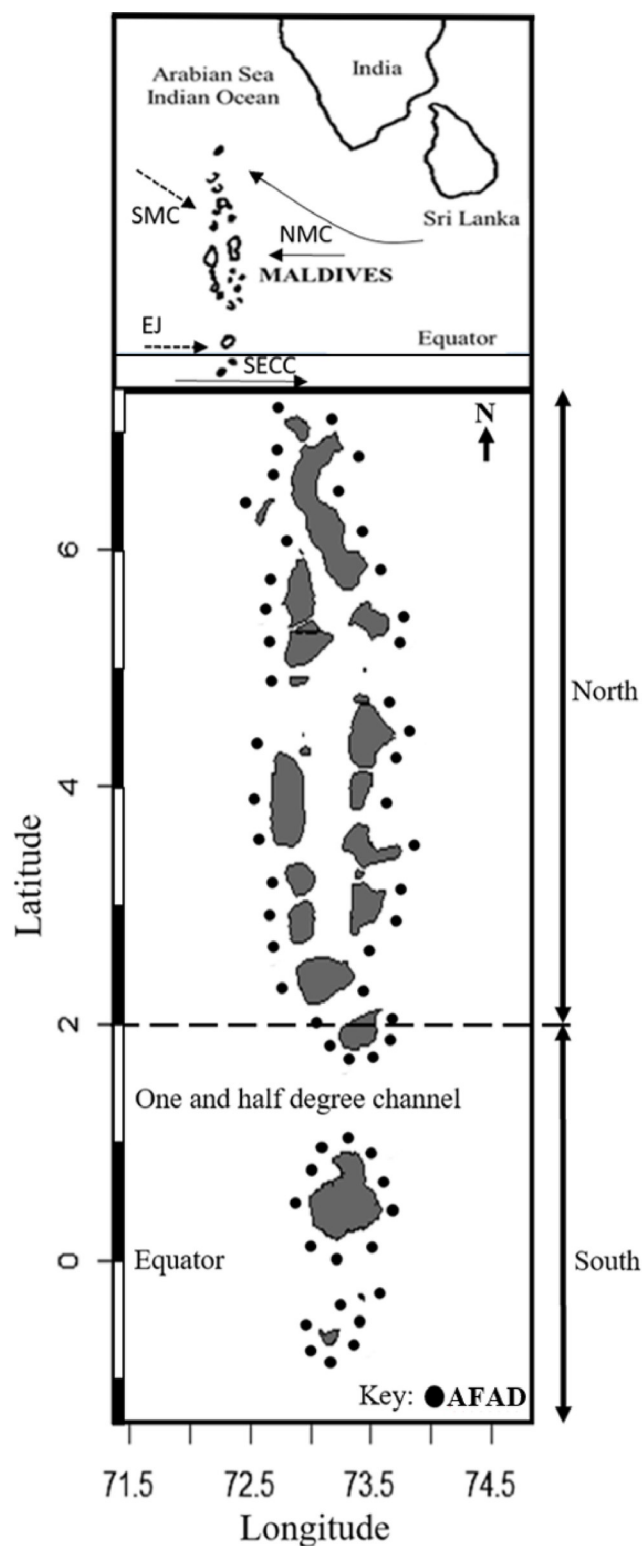
Fig 1. The study area, AFAD network outside Maldives atolls and the direction of monsoon related currents. (Dotted arrows indicate southwest monsoon currents and the continuous arrows indication northeast monsoon currents. NMC–northeast monsoon current, SECC–south equatorial counter current, SMC–southwest monsoon current, EJ–equatorial jet).
