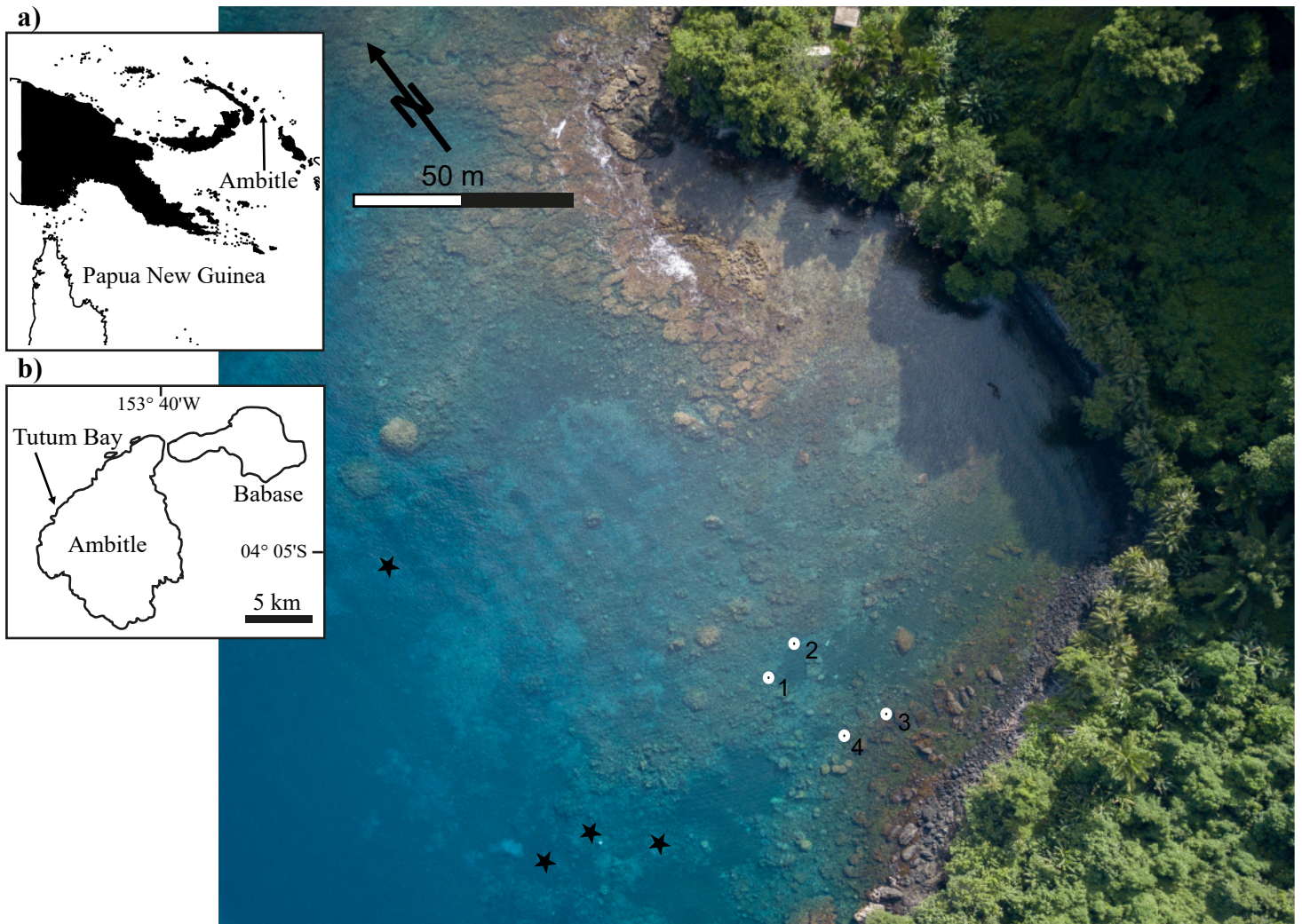
Supplementary Figure S1: Aerial picture of Tutum Bay showing the position of the stations where the pH was measured using SeaFETs during May 2018. White dots indicate the position of the selected reef area (within Sts 1, 2, 3, 4), referred to as high CO 2 site. Black stars indicate the four main massive vents. Ambient station was around one mile south of Tutum Bay
