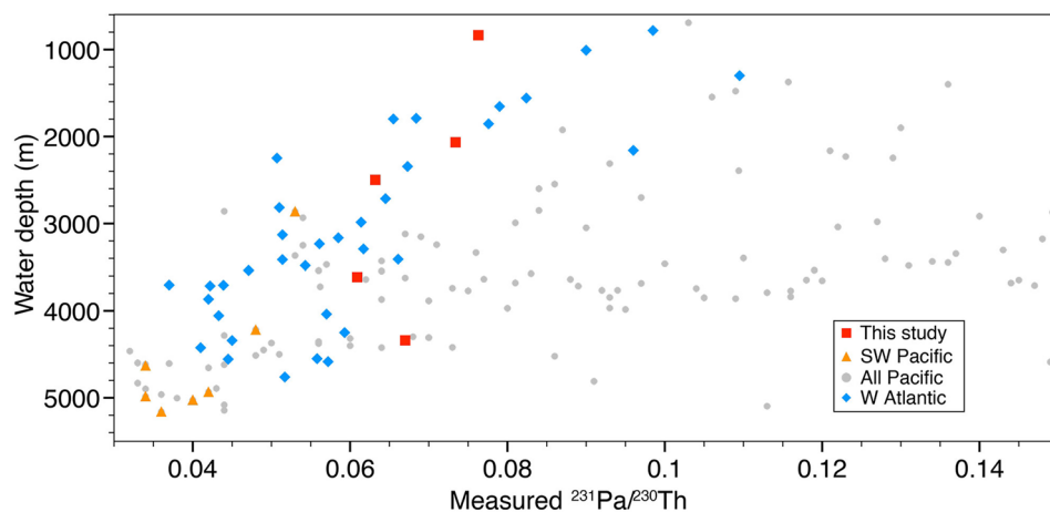
Figure 1. Holocene ^{231}\text{Pa}/^{230}\text{Th} from the Pacific (grey dots) 15 , the SW-Pacific (orange triangles 15 ; red squares, this study), and the W Atlantic (blue diamonds; Table S1). Decreasing ^{231}\text{Pa}/^{230}\text{Th} with water depth in the W Atlantic (blue) is interpreted as an imprint of AMOC, while in the Pacific (grey) a similar correlation is observed only for the SW region (orange, red).
