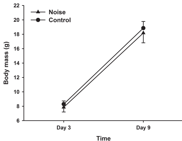
Figure 1. Body mass growth (mean \pm SE) between day 3 and day 9 of house sparrow nestlings exposed to natural rural background noise (control, n = 13 ) or exposed to traffic noise (noise, n = 6 ).
