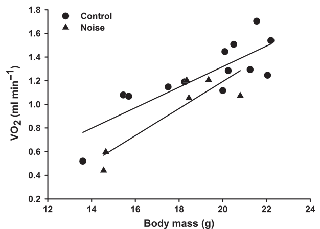
Figure 2. RMR in relation to body mass in house sparrow nestlings exposed to natural rural background noise (control, n = 13 ) or exposed to traffic noise (noise, n = 6 ).
