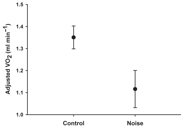
Figure 3. Mass-adjusted RMR (mean \pm SE) of house sparrow nestlings exposed to natural rural background noise (control, n = 13 ) or exposed to traffic noise (noise, n = 6 ). See text for details on the analyses.
