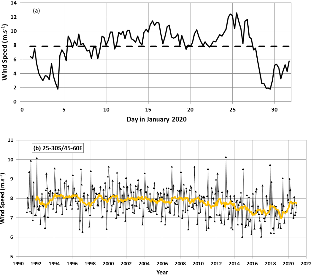
Figure S4: Top (a): 6-hour wind speed ( \text{m.s}^{-1} ) at location 27^{\circ}\text{S}-54^{\circ}\text{E} in January 2020 (dashed line is the average, 7.8 \text{ m.s}^{-1} ). Bottom (b): Average monthly wind speed ( \text{m.s}^{-1} ) in the region 25-30^{\circ}\text{S}/45-60^{\circ}\text{E} from 1991 to 2020 (orange line is the 12 month running mean). Top: data downloaded at https://resources.marine.copernicus.eu/ (WIND_GLO_WIND_L4_NRT_OBSERVATIONS_012_004), last access 20-April-2021. Bottom: data downloaded at https://giovanni.gsfc.nasa.gov/giovanni/ (GMAO, 2015), last access 19-April-2021.
