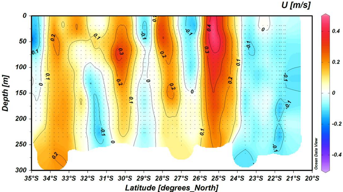
Figure S6: Top: Meridional section (Latitude/Depth) of zonal current ( U in \text{m}\cdot\text{s}^{-1} ) observed from ADCP data collected in January 2005 in the South-Western Indian Ocean (OISO-12 cruise, see the track in Figure S5). The eastward South Indian Counter Current (SICC) is well identified at 25^{\circ}\text{S} down to 250m. Figures produced with ODV (Schlitzer, 2013). Bottom: Map of monthly surface current for January 2005 in the South-Western Indian Ocean showing the retroflexion of the East Madagascar Current and the SICC around 25^{\circ}\text{S} bounding the Chl-a distribution (Figure S5). Figure produced from https://resources.marine.copernicus.eu/ (MULTIOBS_GLO_PHY_REP_015_004) last access, 08-June-2021. ADCP data from OISO-12 cruise available at JAS-ADCP database ( http://uhslc.soest.hawaii.edu/sadcp/DATABASE/01545.html )
