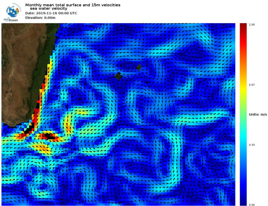
Figure S2: Map of monthly surface current ( \text{m}\cdot\text{s}^{-1} ) for November 2019 in the South-Western Indian Ocean showing the retroreflection of the South-East Madagascar Current and large cyclonic eddies at that period. Figure produced from https://resources.marine.copernicus.eu/ (MULTIOBS_GLO_PHY_REP_015_004) last access, 08-June-2021.
