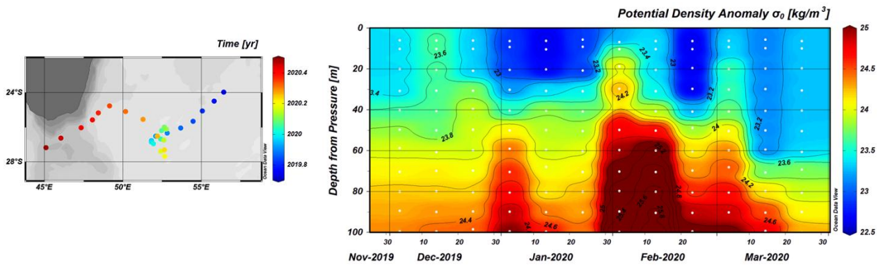
Figure S8: An ARGO float (Code 5904423) in the region of the bloom. Left: trajectory of the float from November 2019 to March 2020. Right: Potential Density ( \sigma_0 ) time-series in the top 100m recorded during this period, showing the strong stratification in January 2020 (mixed layer = 20m) when the float stayed around 27°S-52°E. Source: http://www.coriolis.eu.org/Data-Products/Data-Delivery/Data-selection . (last access, 09-Apr-2021). Figures produced with ODV (Schlitzer, 2013).
