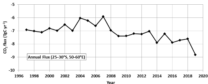
Figure 11. Annual air–sea \text{CO}_2 flux ( \text{TgC yr}^{-1} ) in the south-western Indian Ocean (region of 25\text{--}30^\circ \text{S} , 50\text{--}60^\circ \text{E} ) for the period 1996–2019 from the CMEMS-LSCE-FFNN model. The carbon uptake progressively increased after 2007 with a maximum \text{CO}_2 sink estimated in 2019 when the SEMB was particularly strong.
