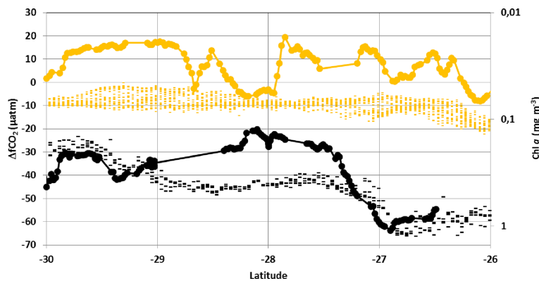
Figure 4. \Delta f\text{CO}_2 ( \mu\text{atm} ) ( \Delta f\text{CO}_2 = f\text{CO}_2^{\text{oce}} - f\text{CO}_2^{\text{atm}} ) and sea surface Chl a ( \text{mg m}^{-3} ) distribution in January 2020 (black) and February 2005 (orange) along the same track around 54° E in the south-western Indian Ocean. Here Chl a is in \log_{10} scale and inverted. In 2020 when the SEMB was particularly strong, \Delta f\text{CO}_2 was negative (ocean CO 2 sink), whereas in 2005 when the bloom was small, \Delta f\text{CO}_2 was close to 0 or positive (ocean CO 2 source).
