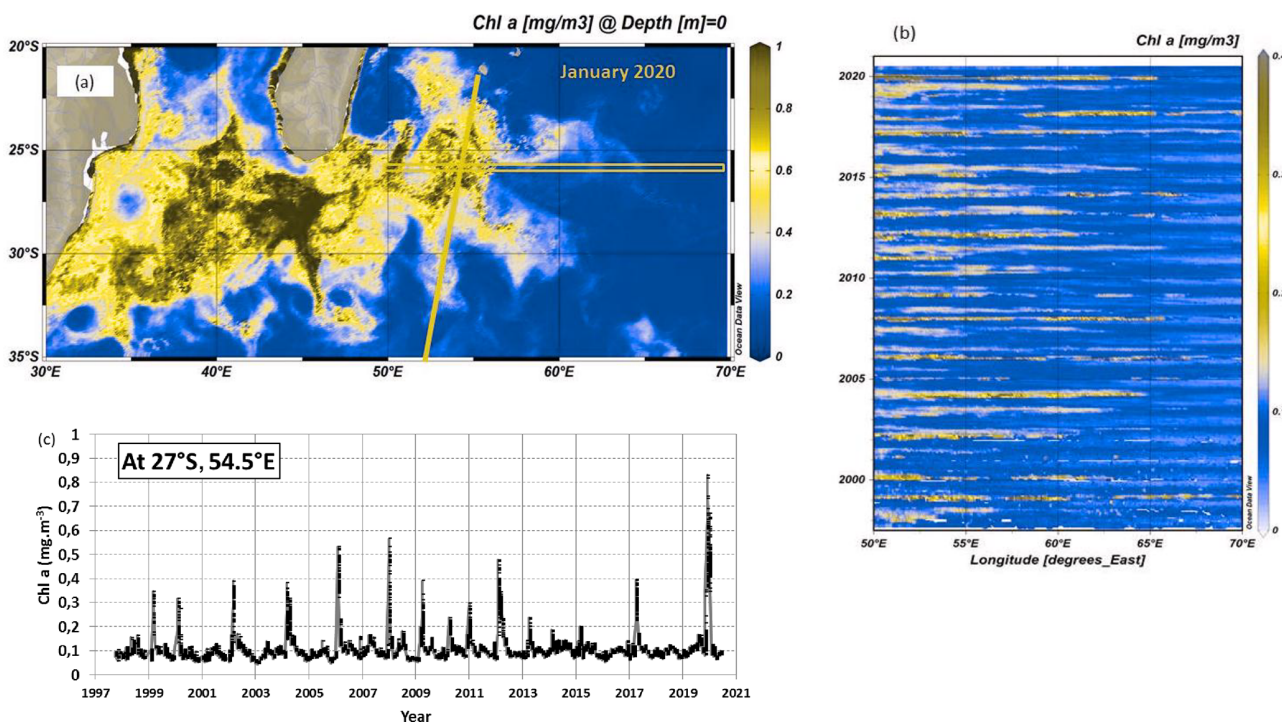
Figure 1. (a) Map of monthly surface Chl a (mg m -3 ) in the south-western Indian Ocean in January 2020 derived from MODIS data (4 km × 4 km resolution), highlighting the bloom south and south-east of Madagascar. (b) Hovmöller time series (time and longitude) of Chl a (mg m -3 ) around 26.5° S along 50–70° E (orange box in a). (c) Time series of monthly Chl a (mg m -3 ) at 27° S, 54.5° E (only when the valid number of pixels is greater than five for each point). The orange line on the map identifies the track of the OISO-30 cruise. The figures highlight the high Chl a concentration in austral summer 2020. Panels (a) and (b) produced with ODV (Ocean Data View; Schlitzer, 2013) from data downloaded from https://resources.marine.copernicus.eu/ (OCEANCOLOUR_GLO_CHL_L4_REP_OBSERVATIONS_009_093, last access: 10 April 2021).
