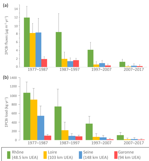
Figure 5. Comparison of specific \Sigma\text{PCBi} flux ( \mu\text{g m}^{-2} \text{yr}^{-1} ) (a) and the mean annual load ( \text{kg yr}^{-1} ) (b) on the French rivers. Fluxes and loads are estimated at the lower station upstream of the tidal influence: Arles–Beaucaire for the Rhône, Montjean for the Loire, Poses–Poissy for the Seine and La Réole–Lamagistère for the Garonne (see locations in Fig. 1). The distance of each station to the sea is expressed as kilometres upstream of estuarine areas (km UEA).
