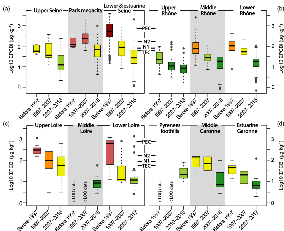
Figure 4. Detailed spatio-temporal distribution of \Sigma\text{PCBi} (log10 scale) in the (a) Seine, (b) Rhône, (c) Loire and (d) Garonne. Colours describe pollution levels in sediments, ranked from forest green (lowest levels) to dark red (highest levels). TEC, PEC, N1 and N2 refer to the main thresholds for PCBs: TEC (threshold effect concentration) and PEC (probable effect concentration) are 59.8 and 676 \mu\text{g kg}^{-1} for total PCBs, respectively (MacDonald et al., 2000); French regulatory levels N1 and N2 refer, respectively, to 80 and 160 \mu\text{g kg}^{-1} of \Sigma\text{PCBi} (order of 17 July 2014).
