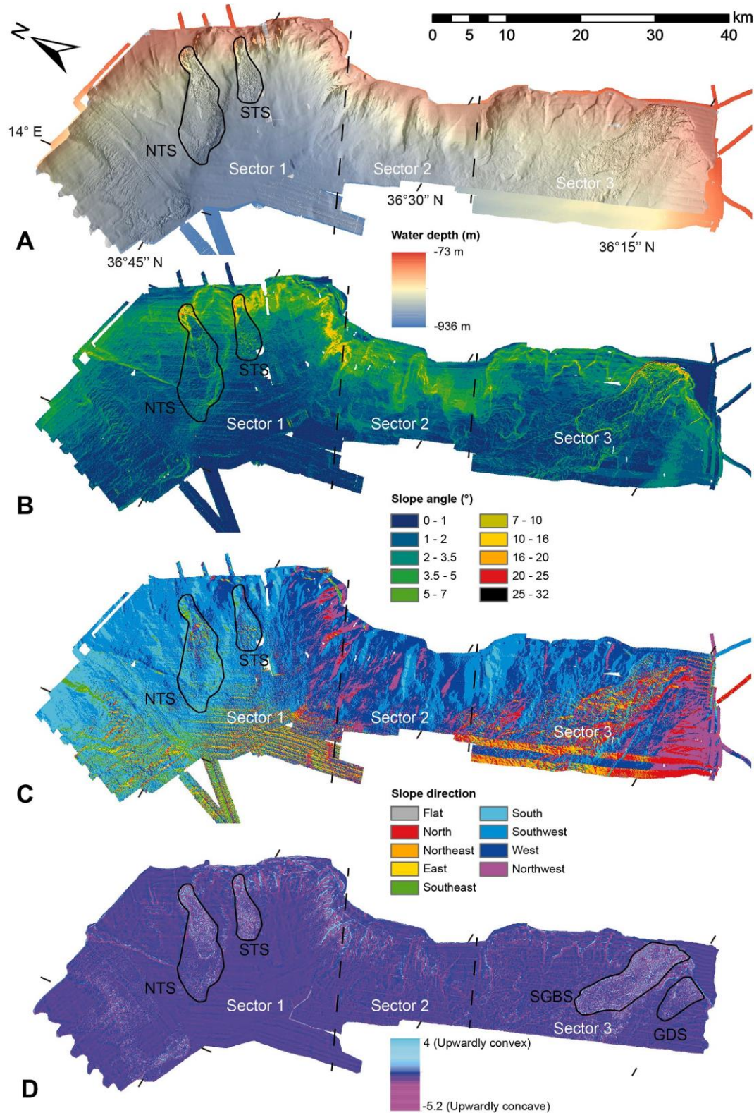
Fig. 11. A. Shaded-relief map of the 25-m-resolution DTM of the eastern margin of the Gela Basin subdivided in three sectors and highlighting the mass-transport deposits (MTDs) described in previous studies (Northern Twin Slide–NTS and Southern Twin Slide–STS). B. Slope gradient map showing an average gradient of 2.1° and up to 32° at the shelf edge of sectors 1 and 3. C. Aspect map showing a southern direction in Sector 1 and an N–NW direction in sectors 2 and 3. D. Curvature map revealing hummocky surfaces corresponding to the MTDs discovered by this study (Southern Gela Basin Slide–SGBS and Gela Drift Slide–GDS).
