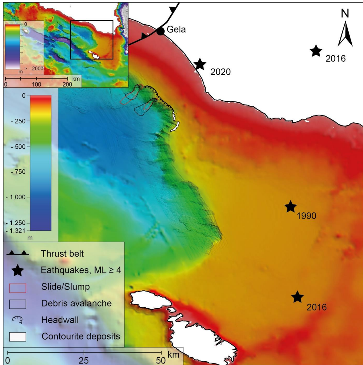
Figure 3.1: Morpho-bathymetric map showing the location of mass-transport deposits (slide/slump and debris avalanche; Kuhlmann et al., 2017) and their headwalls, of contourite deposits (Verdicchio and Trincardi, 2008) and earthquakes (INGV) previously studied along the eastern Gela Basin. ML: Magnitude Local.
