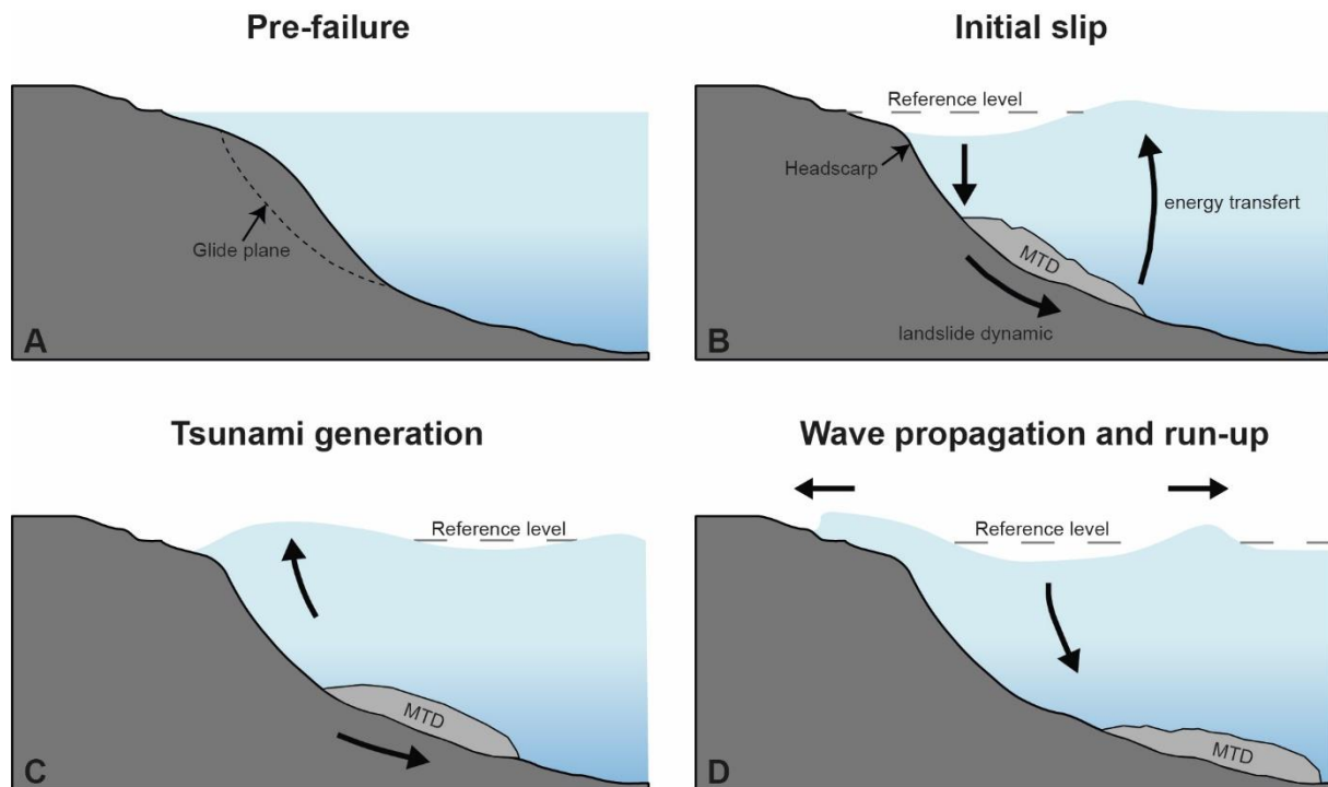
Figure 1.7: Conceptual diagram showing the stages and mechanisms of a tsunami generation from a mass-transport deposit (MTD) with A) the pre-failure, B) the initial landslide dynamic, C) the positive and negative wave generation and D) the wave propagation and run-up (modified after Tappin, 2017; Pakoksung et al., 2019).
