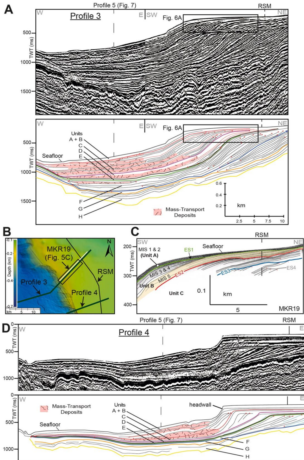
Fig. 5. A. Original seismic section and line drawing of MCS profile 3 showing the largest prograding set of the eastern Gela Basin. B. Bathymetric map showing the location of the enlarged area in Fig. 6A (black rectangle) and of SBS profile (white line) shown in C. C. Interpretation of SBS “MKR19” showing seismic units A, B and C (Table 3). D. Original seismic section and line drawing of MCS profile 4 showing oblique clinoforms during the Pliocene, top truncated strata and a net change in shelf aggradation after the MPT; same vertical and horizontal scales as in Fig. 5A. See Fig. 3A and Table 3 for the description and interpretation of the seismic units.
