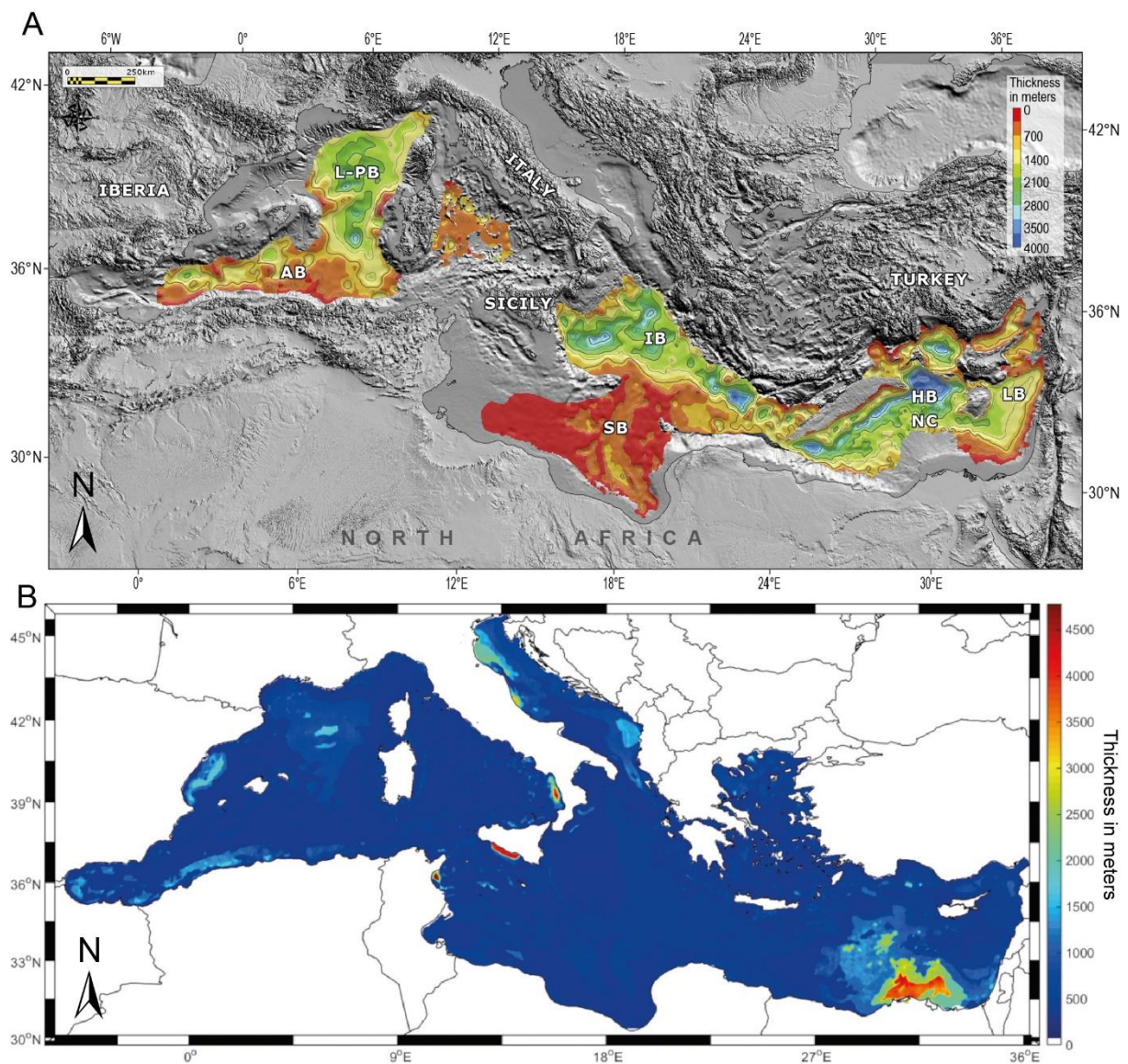
Figure 2.7: A) Thickness map of Messinian evaporites deposited during the Messinian Salinity Crisis in the Mediterranean Sea from Haq et al., (2020). L-PB: Liguro-Provençal Basin, AB: Algerian
