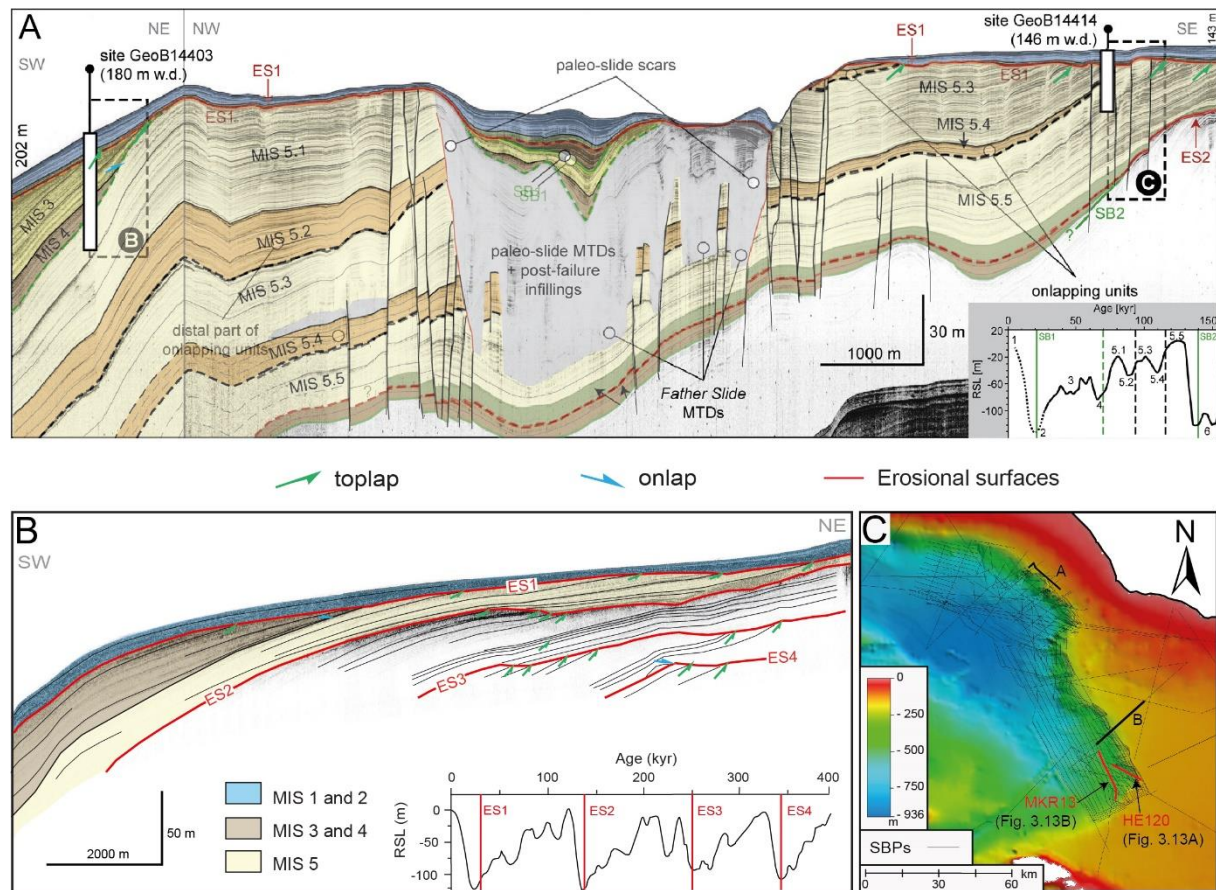
Figure 3.12: A) Sequence-stratigraphic interpretation of an acoustic sub-bottom profile from the northern Gela Basin correlated to long piston cores. Modified after Kuhlmann et al. (2015). B) Example of an interpreted sub-bottom profile studied in this thesis and based on the characteristics of the seismic units identified in Kuhlmann et al. (2015). C) Map showing the location of the sub-bottom profiles of A and B among all the sub-bottom profiles available in the study area.
