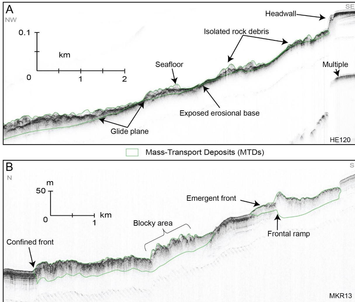
Figure 3.13: Examples of sub-bottom seismic (SBS) profiles showing A) the clear evidence at the seafloor of a headwall and an erosional base and B) two MTDs characterized by different toe domains and separated by high-amplitude seismic reflectors. Note the reduced penetration of the acoustic signal below the MTDs.
