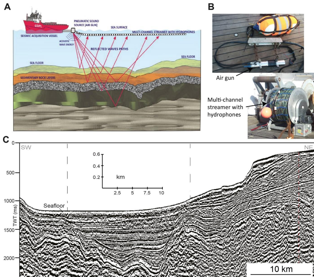
Figure 3.3: A) Sketch representing the acquisition of multi-channel seismic profiles modified after Geostar Survey (2009). B) Pictures showing an example of air gun and multi-channel streamer used onboard a research vessel. C) Example of a multi-channel seismic profile after processing.
