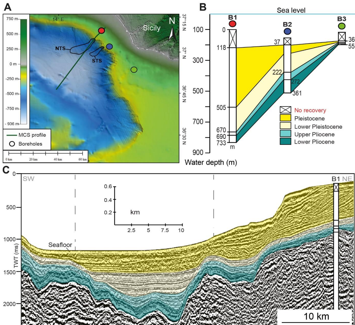
Figure 3.9: A) Bathymetric map showing the location of the three selected deep boreholes and the multi-channel seismic (MCS) profile. B) Correlation of the key time intervals of the selected deep boreholes. C) Geochronology of a MSC profile by the deep borehole B1. Location of the MCS profile in Fig. 3.9A.
