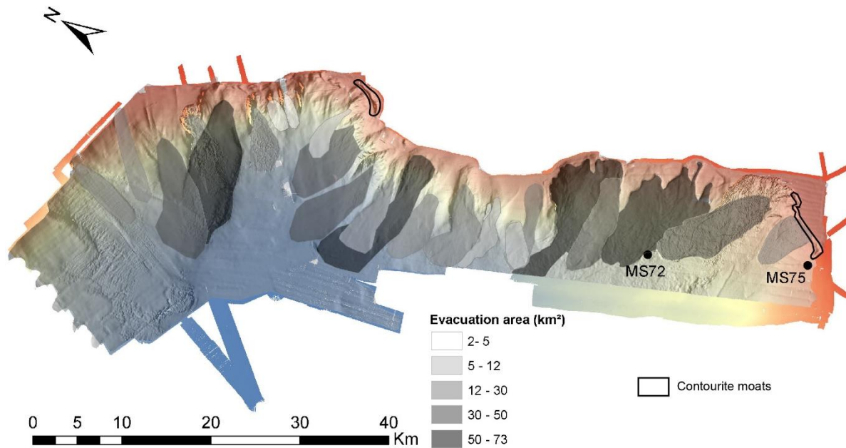
Figure 3.18: High-resolution bathymetric map showing the location of the MTDs and contourite moats identified with a geomorphometric approach compared to the position of the sediment cores recovered in the Gela Basin.
