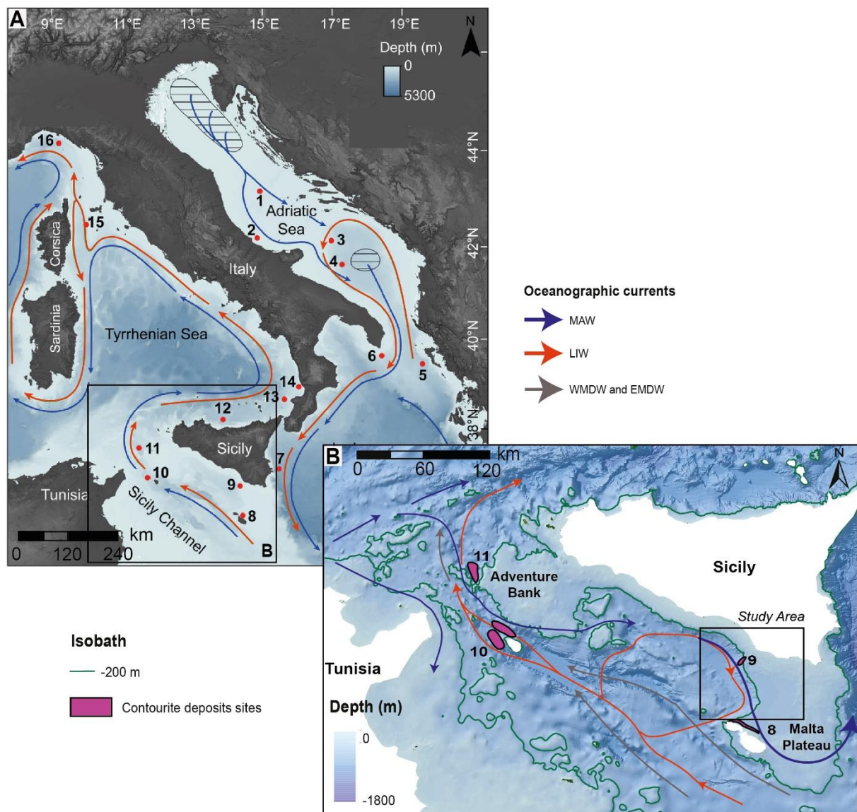
Figure 2.5: Location of contourite deposits in the central Mediterranean Sea along the main bottom current path, modified after Cattaneo et al. (2017). Black rectangle indicates the location of B. B) Zoom on the water masses circulation and exchange in the Strait of Sicily. The purple circles represent the locations and sizes of the previously studied contourite deposits. 8 = Micallef et al., 2013; 9 = Verdicchio and Trincardi, 2008; 10 = Martorelli et al., 2011; 11 = Marani et al., 1993.
