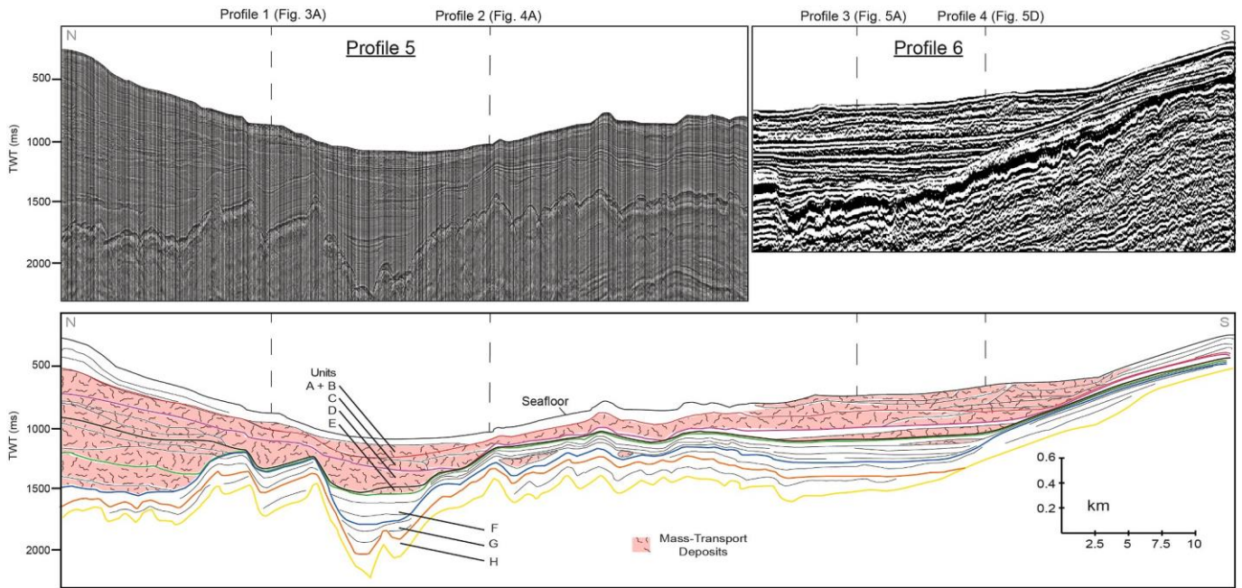
Fig. 7. A. Original seismic section and line drawing of MCS profiles 5 and 6 showing the along-strike variability (NW–SE direction) of the Pliocene–Pleistocene succession. See Fig. 2A for location.
