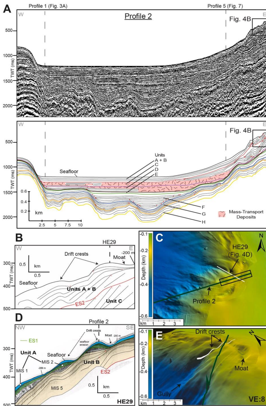
Fig. 4. A. Original seismic section and line drawing of MCS profile 2 highlighting the initiation of contourite deposits during the Upper Pliocene and their evolution through time. B. Enlargement of the prograding shelf-edge of MCS profile 2. C. Bathymetric map showing the location of B (black rectangle) and of SBS profile (white line) shown in D. D. Interpretation of SBS "HE29" highlighting the timing of contourite growth in Sector 1. E. 3D bathymetric view of the area in C. See Fig. 3A and Table 3 for the description and interpretation of seismic units.
