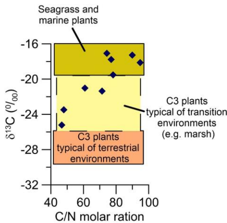
Fig. 6. Bulk composition (carbon/nitrogen ratio combined with stable carbon isotopes) of plant debris sampled in core MS72 (see Figs. 4B and 7 for location of the samples, “vr”). End-members \delta^{13}C values are from Vizzini et al. (2003) and DeLaune and Lindau (1987).
