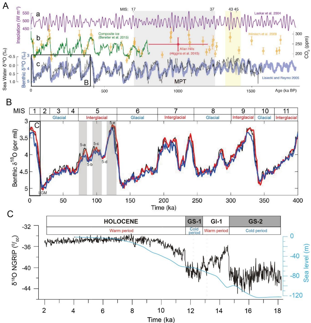
Figure 2.8: A) (a) 65°N summer solstice insolation. (b) Atmospheric CO_2 concentration, Allan Hills vertical error bars indicate 2\sigma spread with horizontal age uncertainty, (c) Global LR04 benthic stacked \delta^{18}O (blue) and ODP 1123 seawater \delta^{18}O (black). The MPT and the "typical 41 ka-world" intervals are highlighted in grey and yellow respectively, from Chalk et al. (2017). B) Correlation of the marine isotope stages (MIS) based on Lopes et al. (2014) with oxygen isotope curve (=ice volume) from Atlantic and Pacific Ocean cores from Lisiecki and Raymo (2009). The positioning of the sub-units of MIS 5 is based on Toucanne et al. (2012). C) \delta^{18}O of NGRIP ice core from Desprat et al. (2013) and sea-level curve from Lambeck et al. (2014). (GS-1: Glacial Stadial 1, GI-1: Glacial Interstadial 1, GS-2: Glacial Stadial 2).
