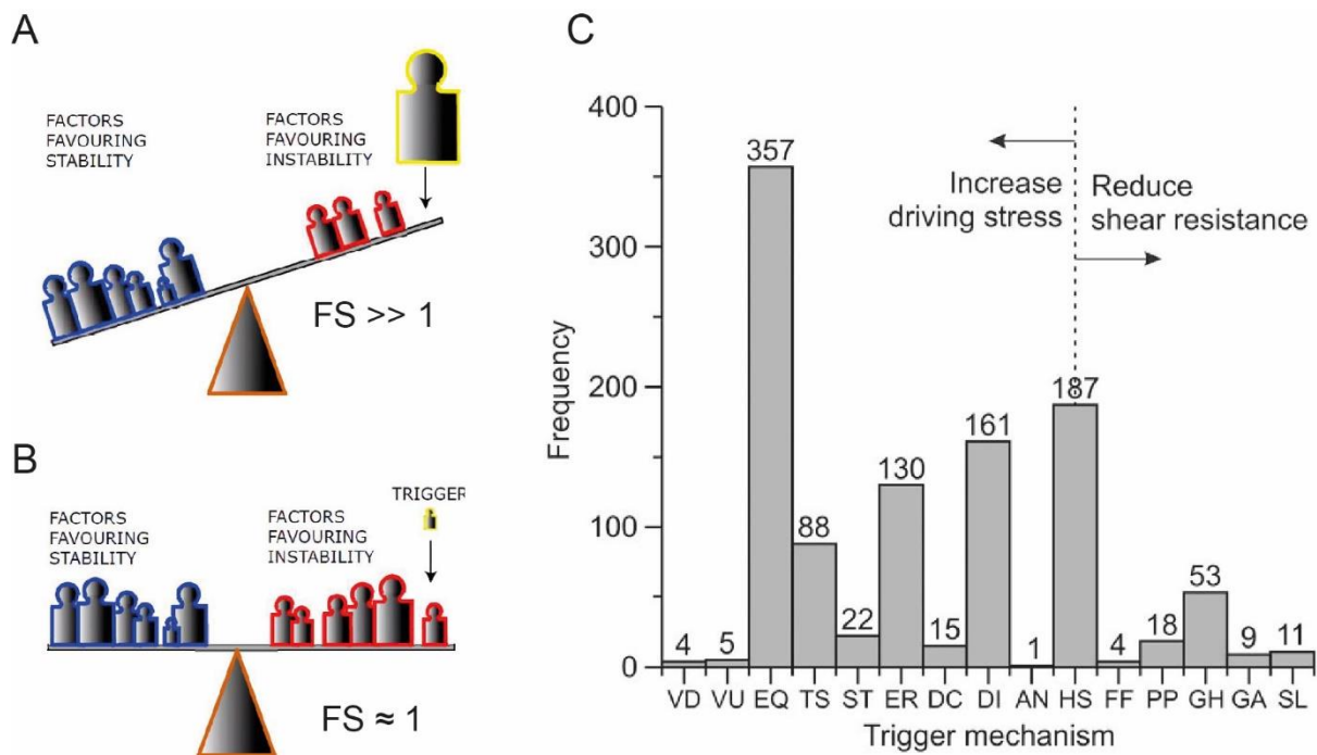
Figure 1.6: A) Representation to understand the role of pre-conditioning factors and B) triggering mechanisms in slope failures (pers. com. Dr. Angelo Camerlenghi). FS: factor of safety. C) Frequency of the slope failures in the Mediterranean Sea versus the major triggering mechanisms (Urgeles and Camerlenghi, 2013). In addition, the triggering mechanisms are separated according to those that increase the driving stress and those that reduce the shear strength. VD: volcano development, VU: volcano uplift, EQ: earthquake, TS: tectonic steepening, ST: steepening, ER: erosion, DC: differential compaction, DI: diapirism, AN: anthropic, HS: high sedimentation rates, FF: fluid flow, PP: pore pressure, GH: gas hydrates, GA: gas, SL: sea level.
