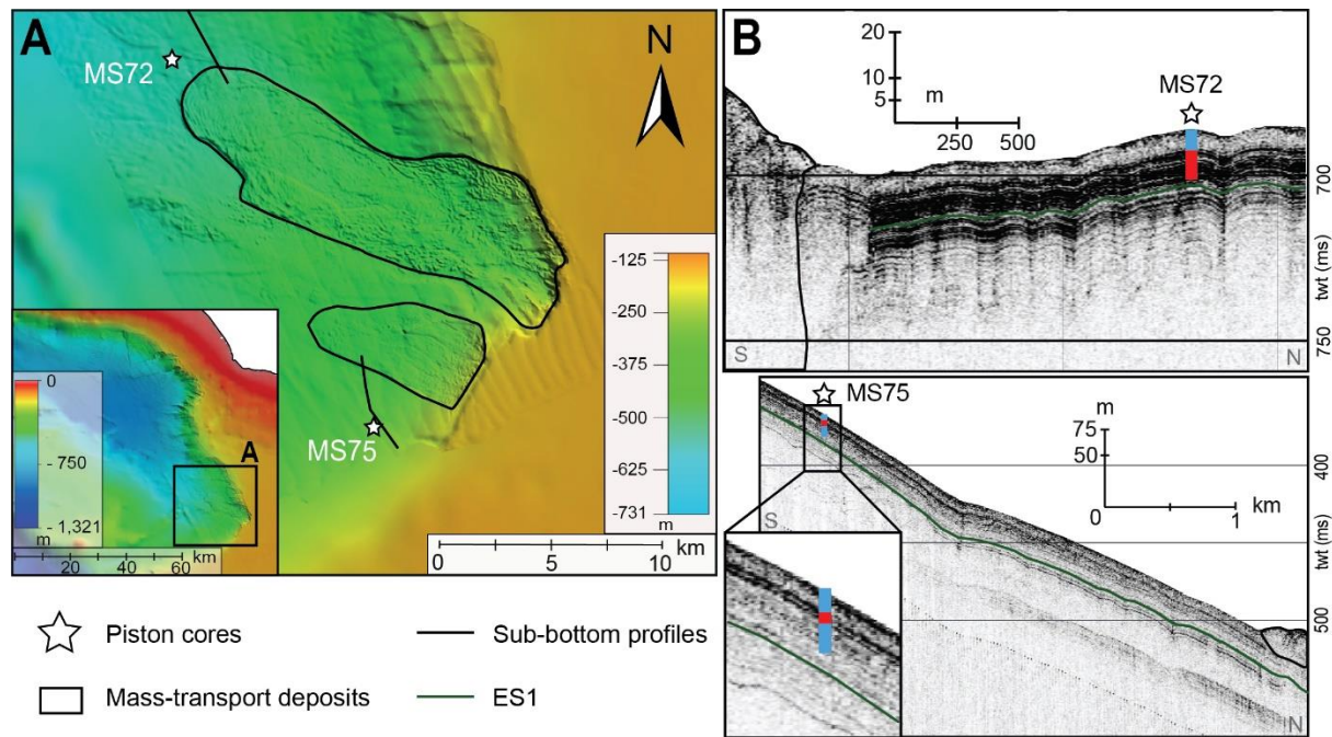
Figure 3.14: A) Morpho-bathymetric map showing the location of the two piston cores studied in this research. B) Location and representation of the penetration depth of the piston cores on sub-bottom profiles. The different colours is used to indicate the changes of amplitude reflectors crossed by the cores. Red = high amplitude reflectors, blue = low amplitude reflectors.
