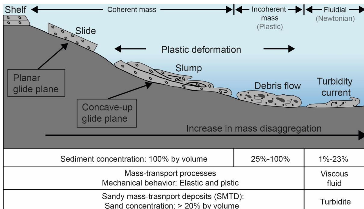
Figure 1.3: Schematic illustration of a complex subaqueous landslide transformed in terms of sediment concentration and mechanical behaviour as it moves downslope, modified from Shanmugam (2013).
