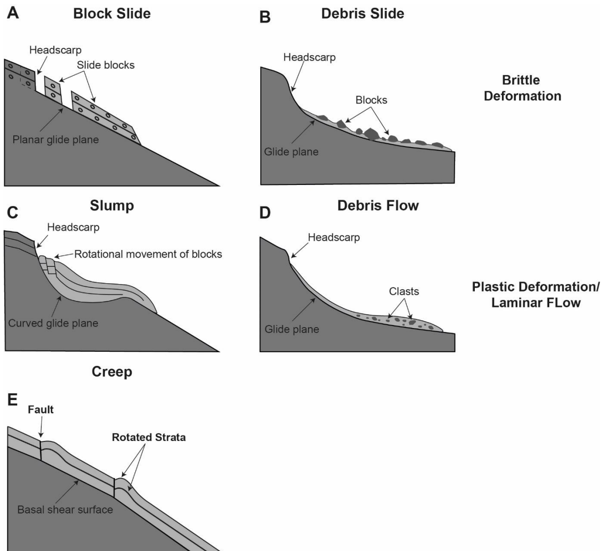
Figure 1.2: Schematic illustration of the major types of submarine gravity-driven depositional processes modified and adapted from Hugh et al. (2002); Harders et al. (2011).
