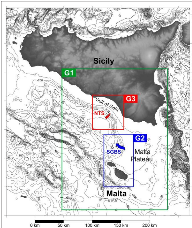
FIGURE 4 | Tsunami computational grids: the larger (G1) is characterized by a 250-m step, while the smaller ones (G2 and G3) have higher resolution (50-m spaced nodes) and are focused on the SGBS and NTS areas, respectively. The propagation of the tsunami over domains with different spatial intervals is possible through the nested-grids technique.
