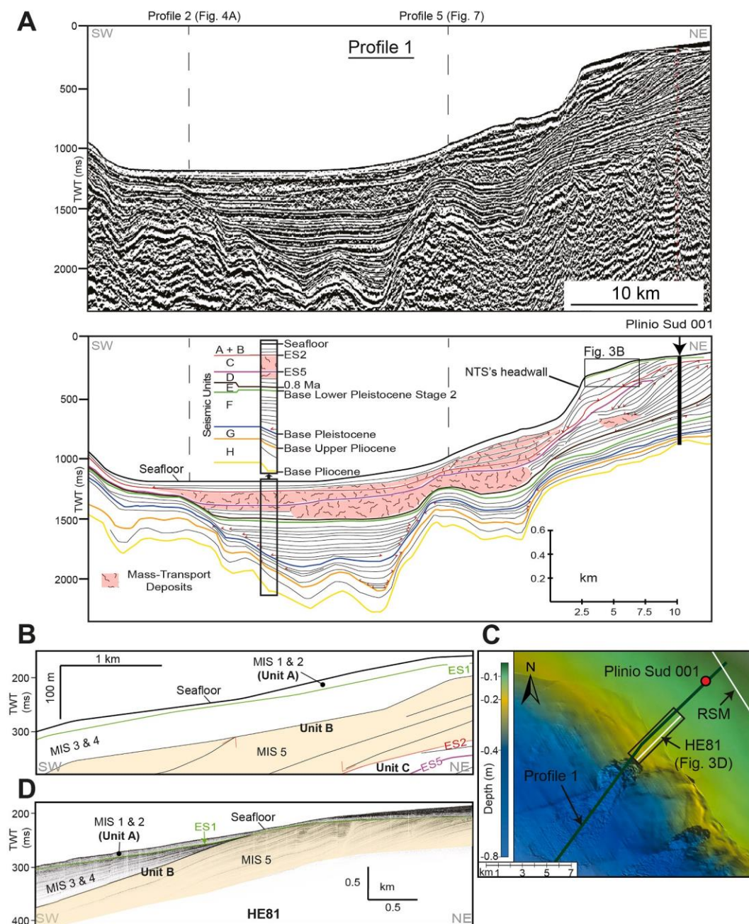
Fig. 3. A. Original seismic section and line drawing of MCS profile 1 crossing the borehole “Plinio Sud 001” (location in Fig. 2A). B. Enlargement of the prograding shelf-edge of MCS profile 1. C. Bathymetric map showing the location of B (black rectangle) and of SBS profile (white line) shown in D. D. Interpretation of SBS profile “HE81” showing the geometry of the seismic units A and B (Table 3) at the shelf edge. This profile was used to correlate the unconformity ES1 on MCS profile 1.
