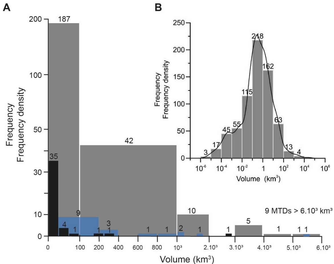
Figure 1.5: A) Histogram showing the number of slope failures and their estimated volumes worldwide (grey bars), in the western (black bars) and eastern North Atlantic (blue bars) (modified and adapted from Hühnerbach et al., 2004, Moscardelli and Wood, 2016) and B) in the Mediterranean Sea (after Urgeles and Camerlenghi, 2013).
