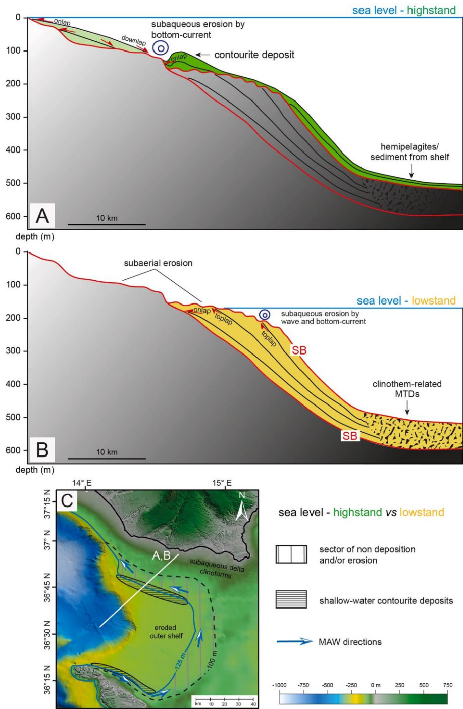
Fig. 14. Along-dip shelf stratigraphic reconstructions illustrating the changes in sediment deposition during the current Holocene highstand (A) and the Last Glacial Maximum (B). C. The occurrence of an elongated area of non-deposition adjacent to contourite deposits on the Malta Plateau indicates the path of bottom currents flowing at around 100 m w.d.
