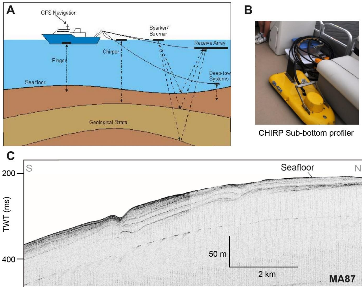
Figure 3.4: A) Schema representing the deployment of various shallow-water sub-bottom profiling systems from Stoker et al. (1997). B) Picture of a CHIRP sub-bottom profiler from WHOI (2020). C) Example of a CHIRP sonar seismic profile used in this research.
