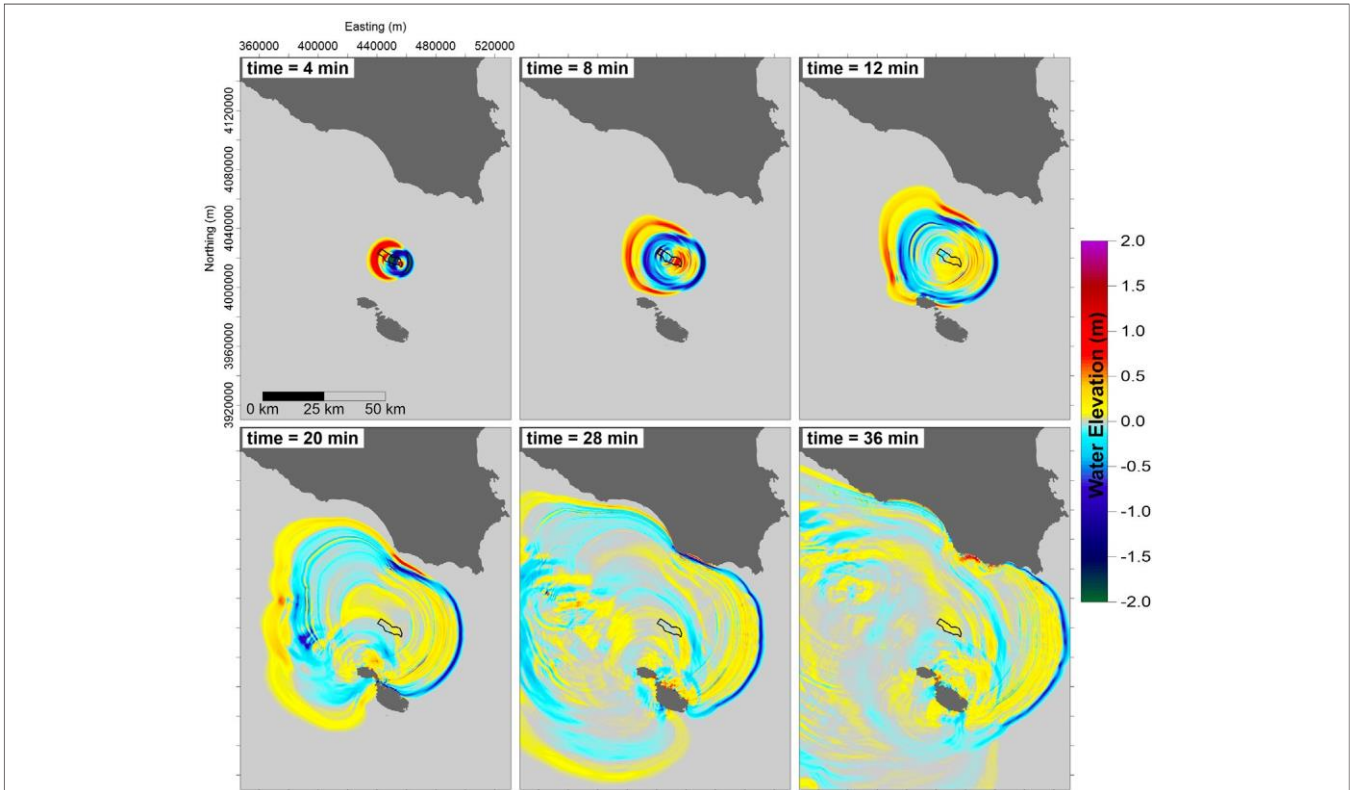
FIGURE 7 | Propagation frames for the SGBS-generated tsunami. The color scale spans the interval [-2;2] m and is saturated for values out of this range. The black contour delimits the SGBS slide area.
