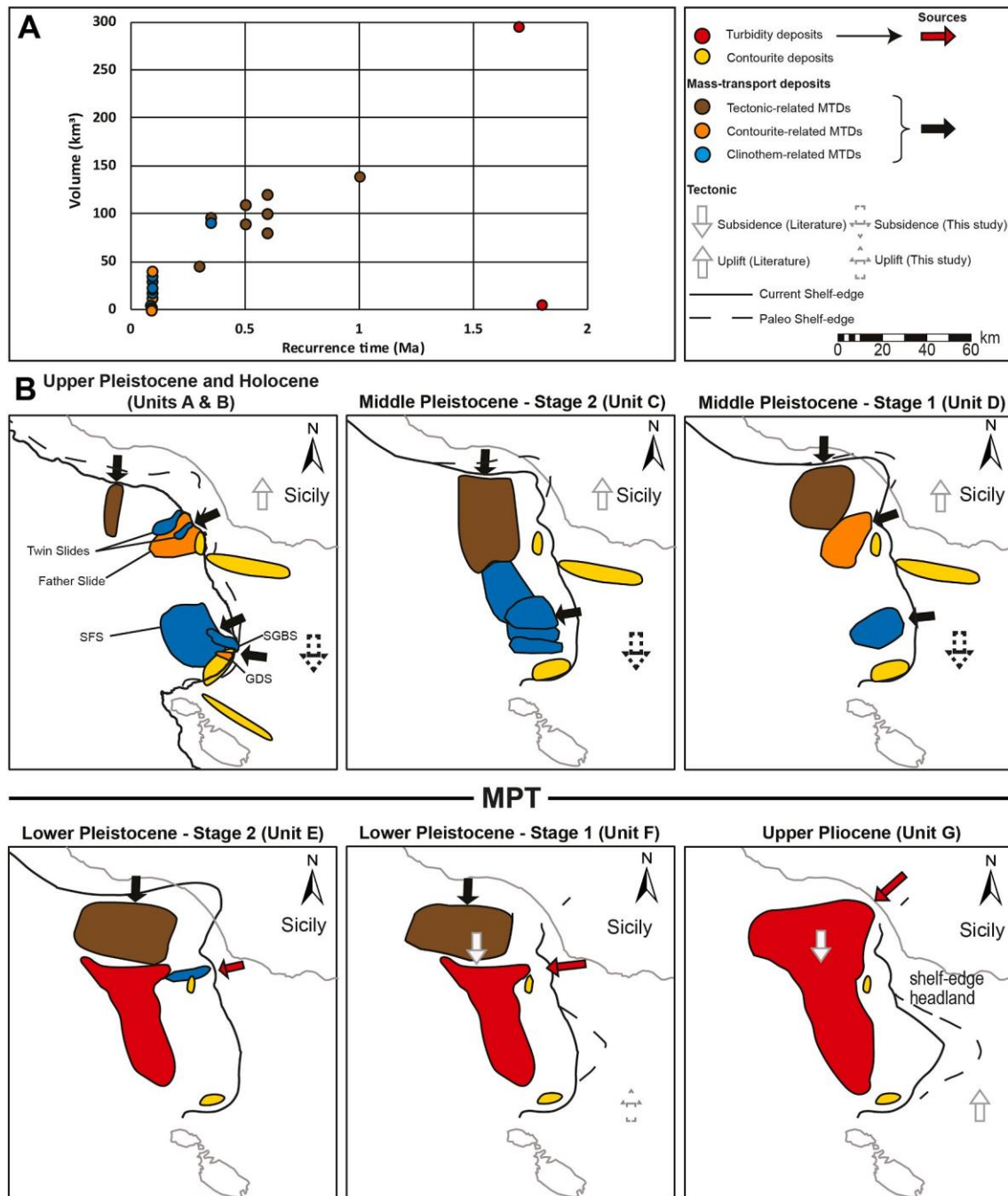
Fig. 13. A. Recurrence time plotted against reconstructed volumes of mass-transport deposits (MTDs) and turbidite deposits mapped in the eastern Gela Basin since the Pliocene (see also Table 4). B. Time sketch of the eastern Gela shelf-edge margin growth (black lines) for the Pliocene to Quaternary along with the distribution of sedimentary bodies and MTDs.
