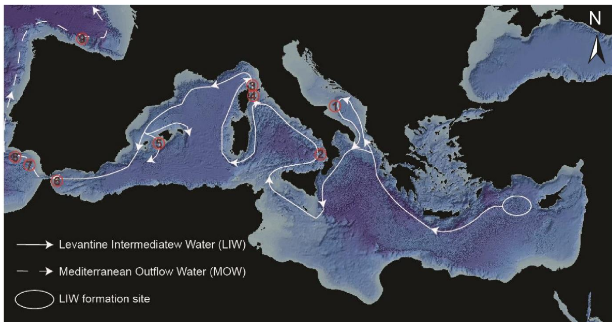
Figure 2.6: Morpho-bathymetric map of the Mediterranean Sea with the location of buried contourite deposits discovered along the present-day path of the LIW based on multiple references (Table 2.1).
