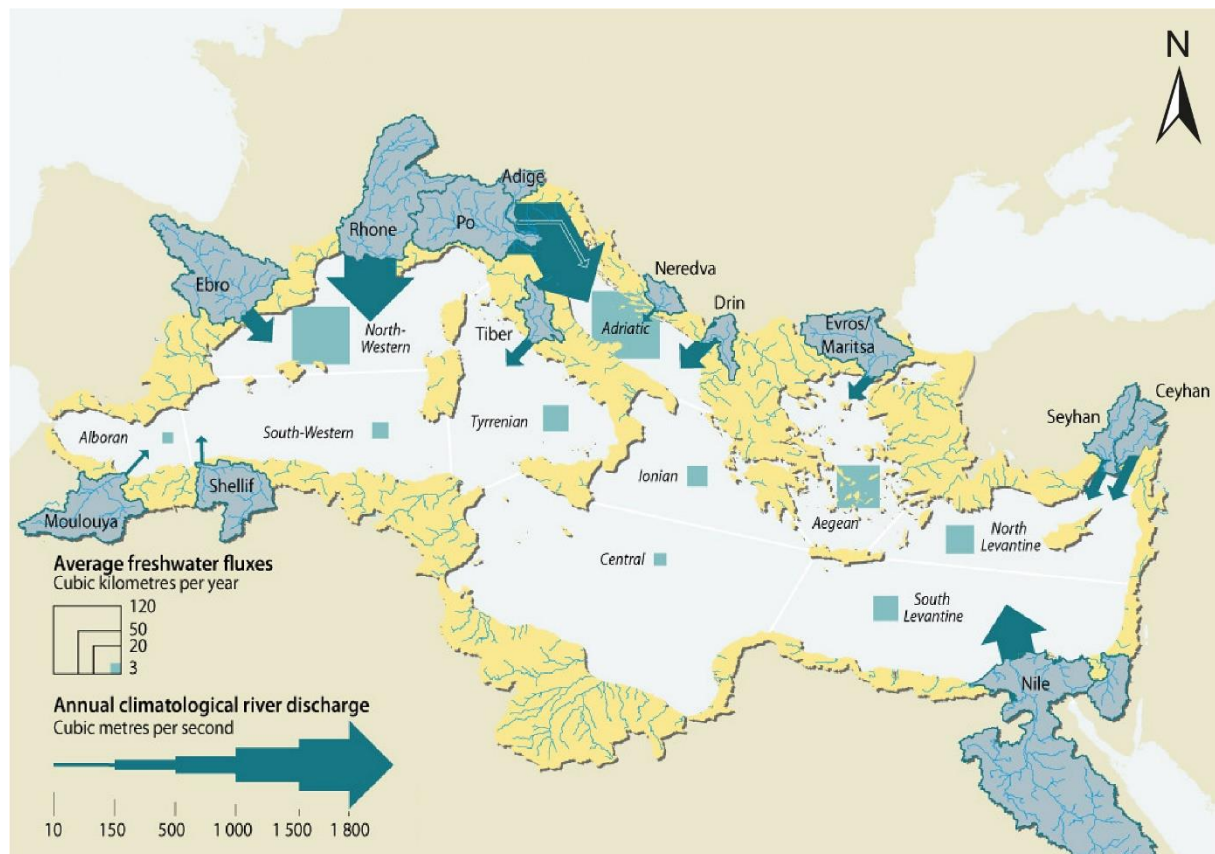
Figure 2.11: River discharge of freshwater into the Mediterranean Sea modified from GRID-Arendal ( http://www.grida.no/resources/5897 ) based on Struglia et al. (2004) and Ludwig et al. (2009).
