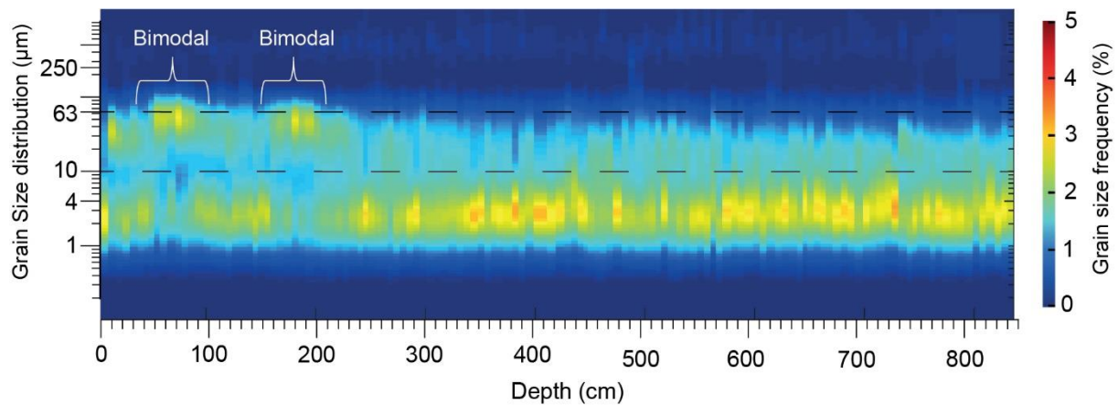
Figure 3.17: Example of grain distribution and frequency for core MS75. Note the changes from unimodal to bimodal distribution with an increase in the sortable silt fraction.
