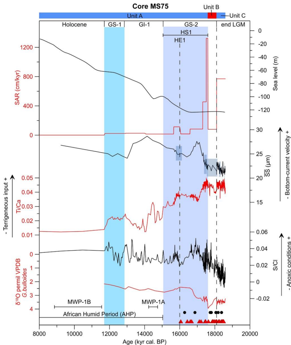
Fig. 9. Isotopic stratigraphy ( \delta^{18}\text{O} ), geochemical element composition ( \text{S/Cl} , \text{Ca/Ti} ), sortable silt mean size ( \overline{\text{SS}} ) and LSR of core MS75 displayed in age. Sea-level curve from Lambeck et al. (2014). Reworked foraminifera = black circles, pyrites = red triangles. GS-1 = Glacial Stadial 1 (sky blue bar), GI-1 = Glacial Interstadial 1, HS1 = Heinrich Stadial 1 (dark blue bar), HE1 = Heinrich Event 1, LGM = Last Glacial Maximum. Pale blue rectangles on \overline{\text{SS}} data represent sediments unsorted by bottom currents. (For interpretation of the references to colour in this figure legend, the reader is referred to the web version of this article.)
