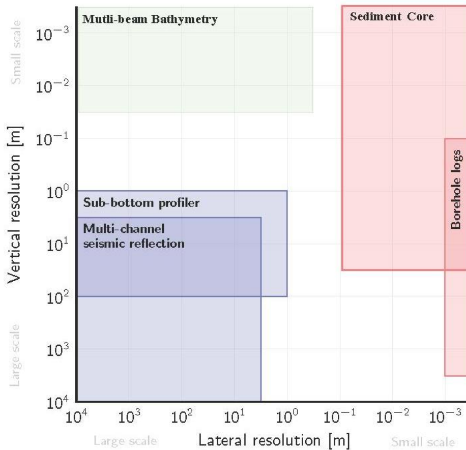
Figure 3.8: Comparison of the resolution of the data used in this research adapted and modified from pers. com. Dr. Johnathan Ford.
