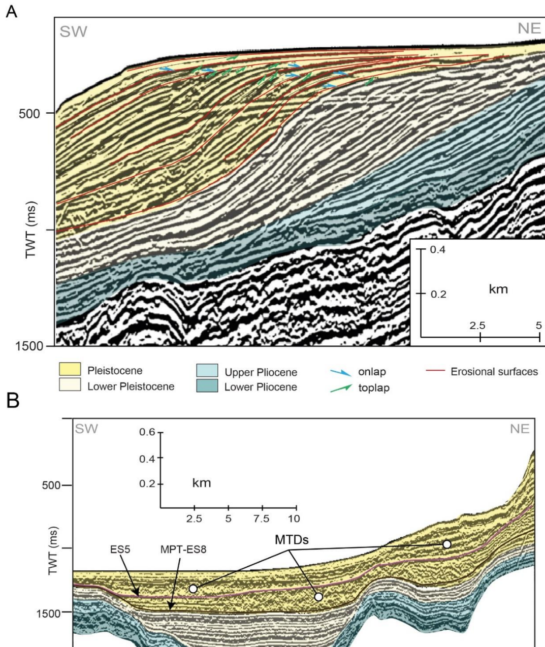
Figure 3.11: Zoom on 2 selected MCS profiles to explain the methods for the identification of A) erosional surfaces (red lines) and B) mass transport deposits (MTDs) on seismic profiles. Location of the profiles in Fig. 3.10.
