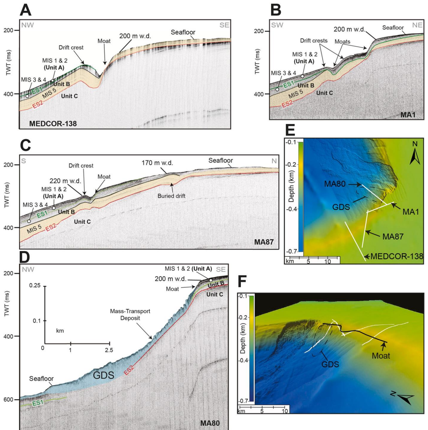
Fig. 10. A. SBS profile “MEDCOR-138” showing the internal structures of the most prominent contourite deposit in the upper slope of Sector 3. Seismic units A and B show that the deposition of the drift crests occurred mainly during MIS 5 (see also Table 3). B. SBS profile “MA1” showing the continuity of the contourite deposits along the shelf edge and upper slope. C. SBS “MA87” showing the presence of a buried drift developed on top of ES2. D. SBS “MA80” shows a moat and the Gela Drift Slide (GDS) gliding on top of the erosional surface ES2. E. Bathymetric map with location of the seismic profiles shown in A, B, C and D. F. 3D bathymetric view showing the GDS deposit located downslope the failed drift crests. Horizontal and vertical scales of SBS profiles are given in Fig. 10D.
