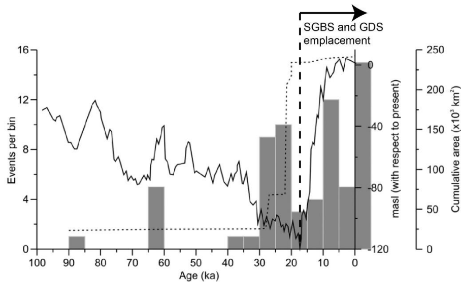
Figure 7.4: Representation of the number of MTDs found in the Mediterranean Sea with respect to their age constrained plotted versus the sea level curve of the last 100 kyr. Figure modified from Urgeles and Camerlenghi (2013).
