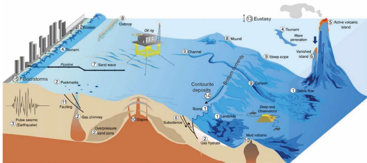
Figure 1.8: Sketch representing the different marine geohazards present on a continental margin (modified from Camargo et al., 2019).
