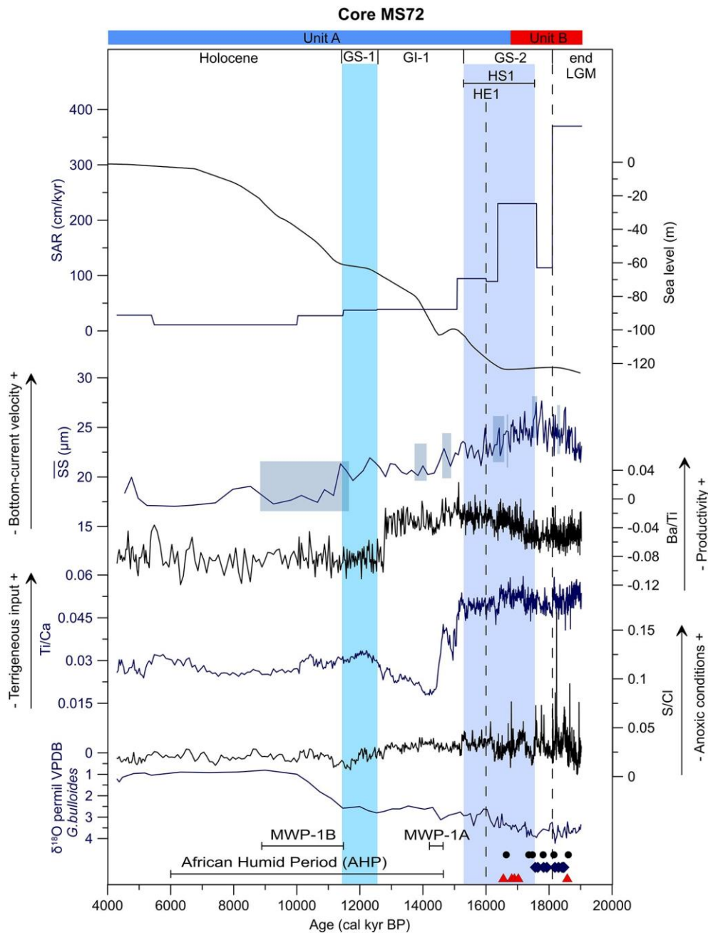
Fig. 10. Isotopic stratigraphy ( \delta^{18}\text{O} ), geochemical element composition (S/Cl, Ca/Ti, Ba/Ti), sortable silt mean size ( \overline{SS} ), and LSR of core MS72 displayed in age. Sea-level curve from Lambeck et al. (2014). Reworked foraminifera = black circles, pyrites = black triangles, plant debris = blue diamonds. See Fig. 9 for other symbols and abbreviations. (For interpretation of the references to colour in this figure legend, the reader is referred to the web version of this article.)
