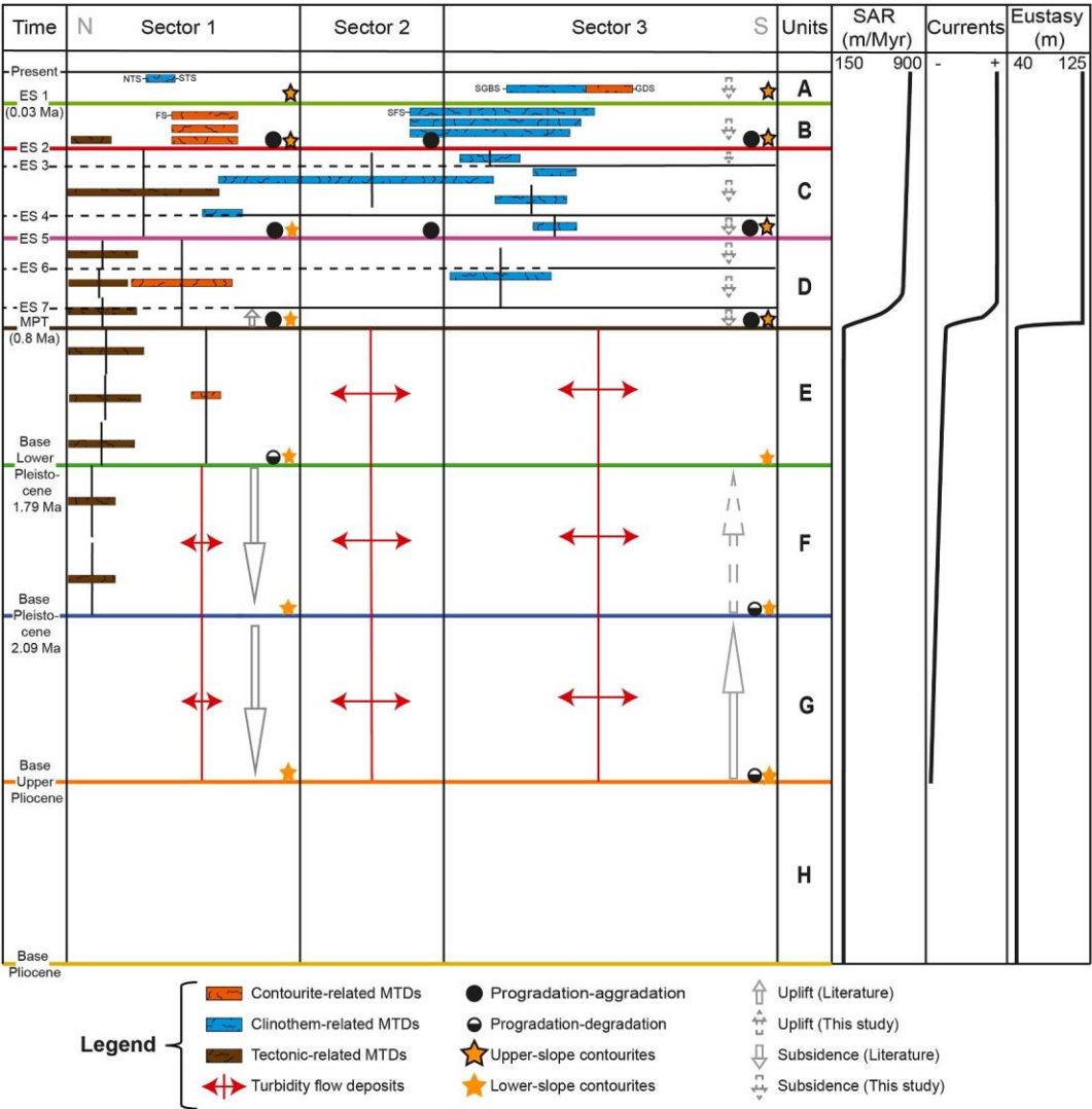
Fig. 12. N–S oriented chronostratigraphic cross-section summarizing the evolution of the eastern Gela Basin since the Pliocene. The temporal distribution of the deposits is schematic. SAR: sediment accumulation rate.
