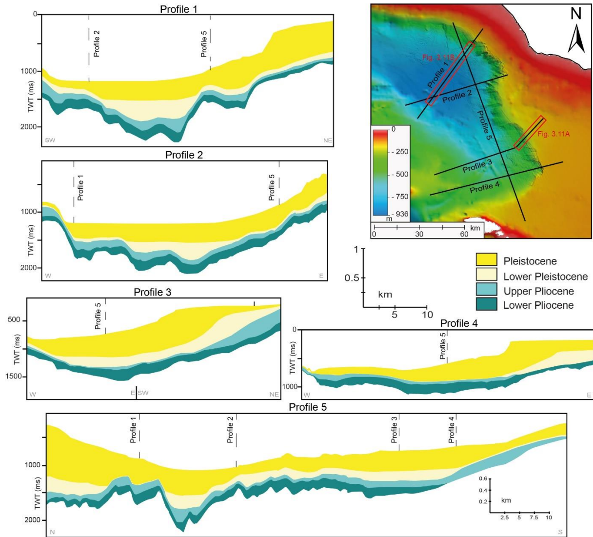
Figure 3.10: Identified geochronology of the selected MCS profiles based on profile 1 from Lower Pliocene to Pleistocene. Location of the MCS profiles on the map. Note the junction of all the MCS profiles.
