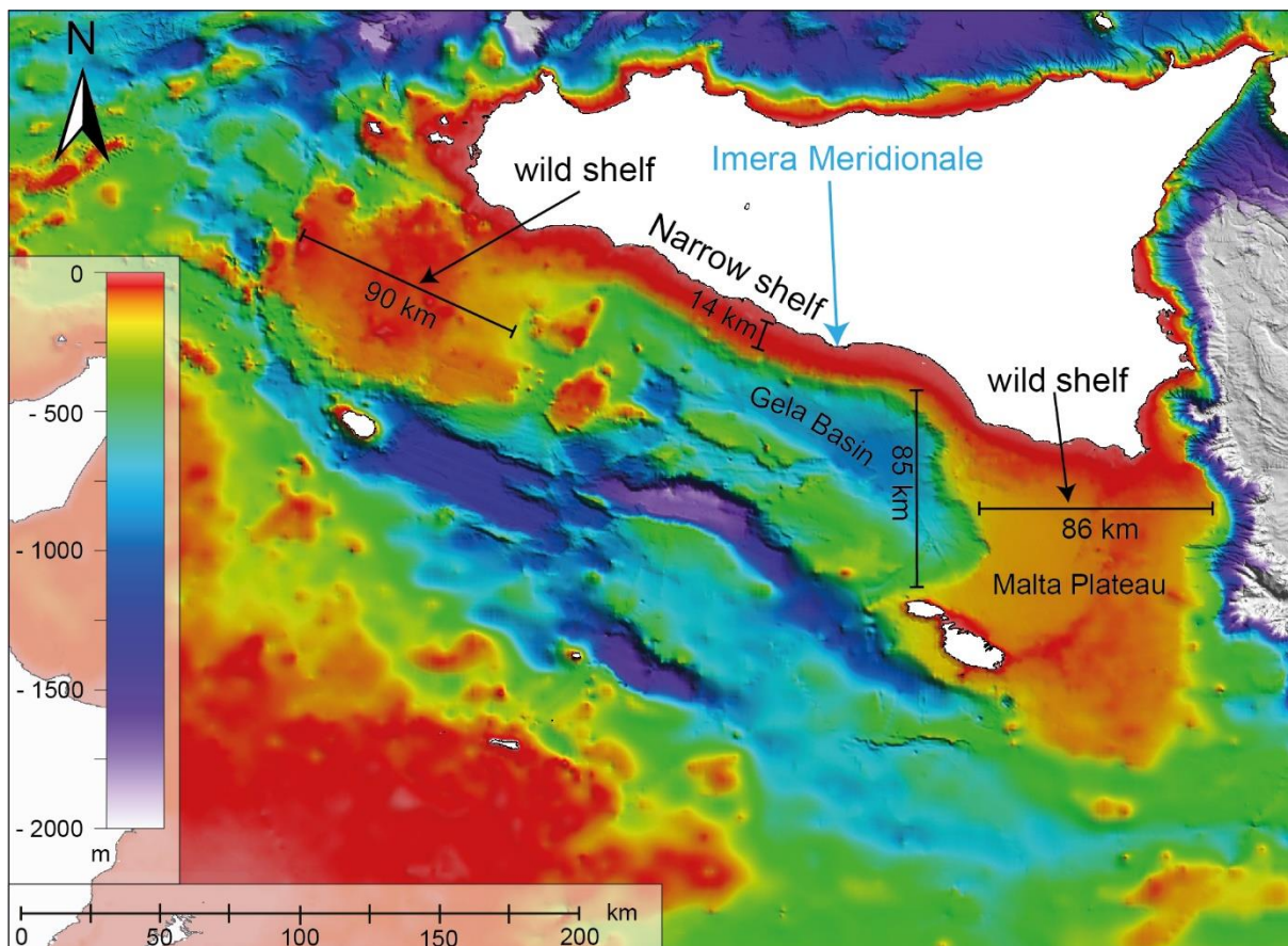
Figure 2.10: Morpho-bathymetric map of the Strait of Sicily. Location of the Imera Meridionale mouth based on Verri et al. (2017).
