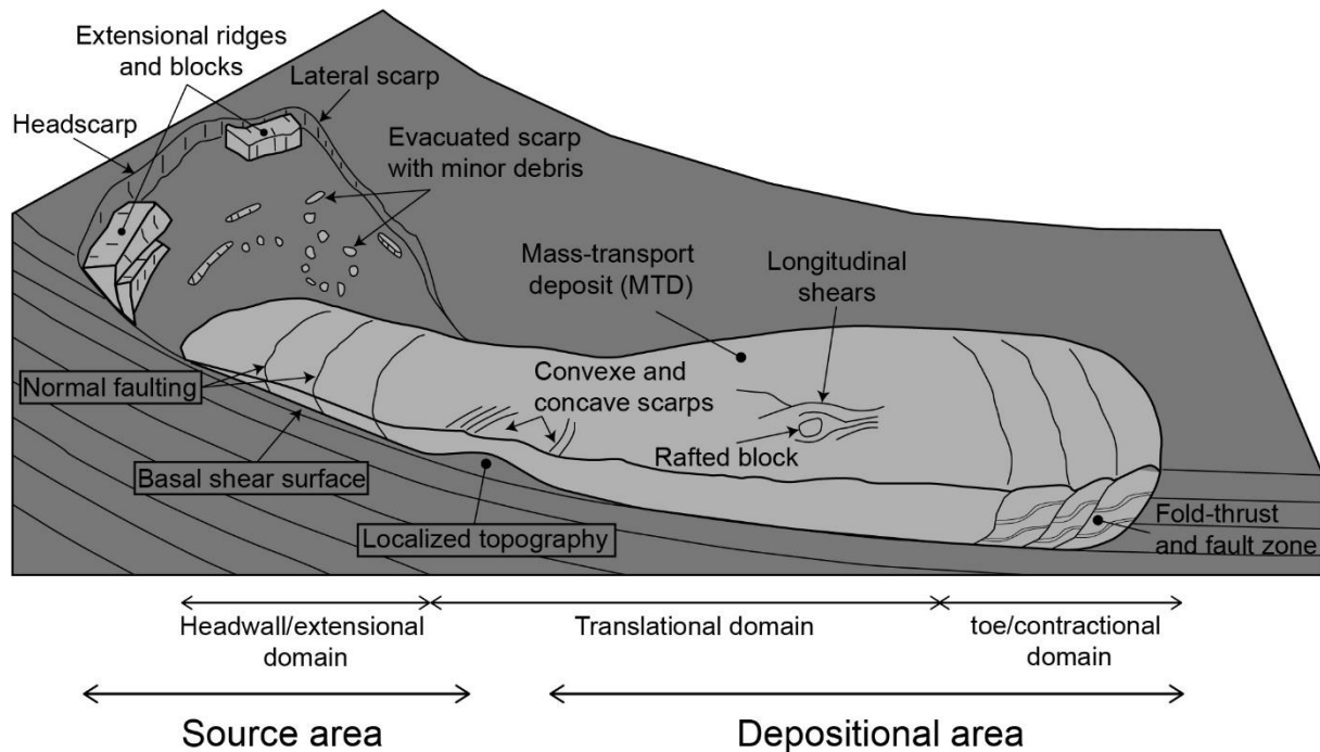
Figure 1.1: Schematic representation of the anatomy of a subaqueous landslide adapted and modified from Bull et al. (2009; Mountjoy and Micallef (2018); Steventon et al. (2019).
