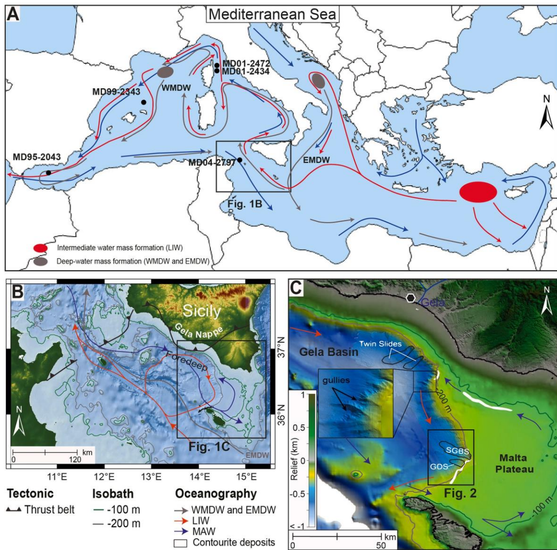
Fig. 1. A) Circulation of the surface (Modified Atlantic Water – MAW), intermediate (Levantine Intermediate Water – LIW) and deep-waters (Western and Eastern Mediterranean Deep Water – WMDP and EMDW) in the Mediterranean Sea (modified from Astraldi et al., 2001 ). The black circles indicate the location of the reference cores used in this study. B) Relief and bathymetric map of the Strait of Sicily area with superimposed the water mass circulation and the general tectonic framework (modified from Millot, 1999 ; Millot and Taupier-Letage, 2005 ). C) Relief and bathymetric map of the Gela Basin highlighting mass-transport deposits: Twin Slides ( Minisini et al., 2007 ), Southern Gela Basin Slide (SGBS) and Gela Drift Slide (GDS) ( Gauchery et al., 2021 ). White polygons indicate contourite deposits ( Verdicchio and Trincardi, 2008 ; Gauchery et al., 2021 ).
