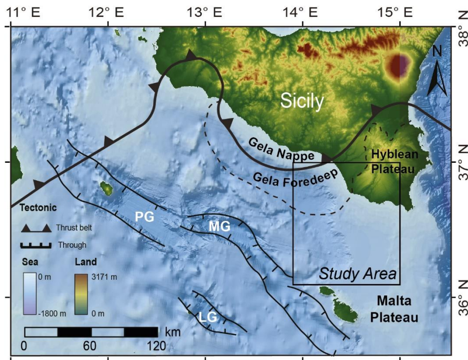
Figure 2.3: Relief and bathymetric map showing the modern emplacement of the Apenninic arc (Maghrebian fold and-thrust belt) in the Strait of Sicily as well as the location of the grabens, which represents the extensional rift system. PG = Pantelleria Graben, MG = Malta Graben, LG = Linosa Graben.
