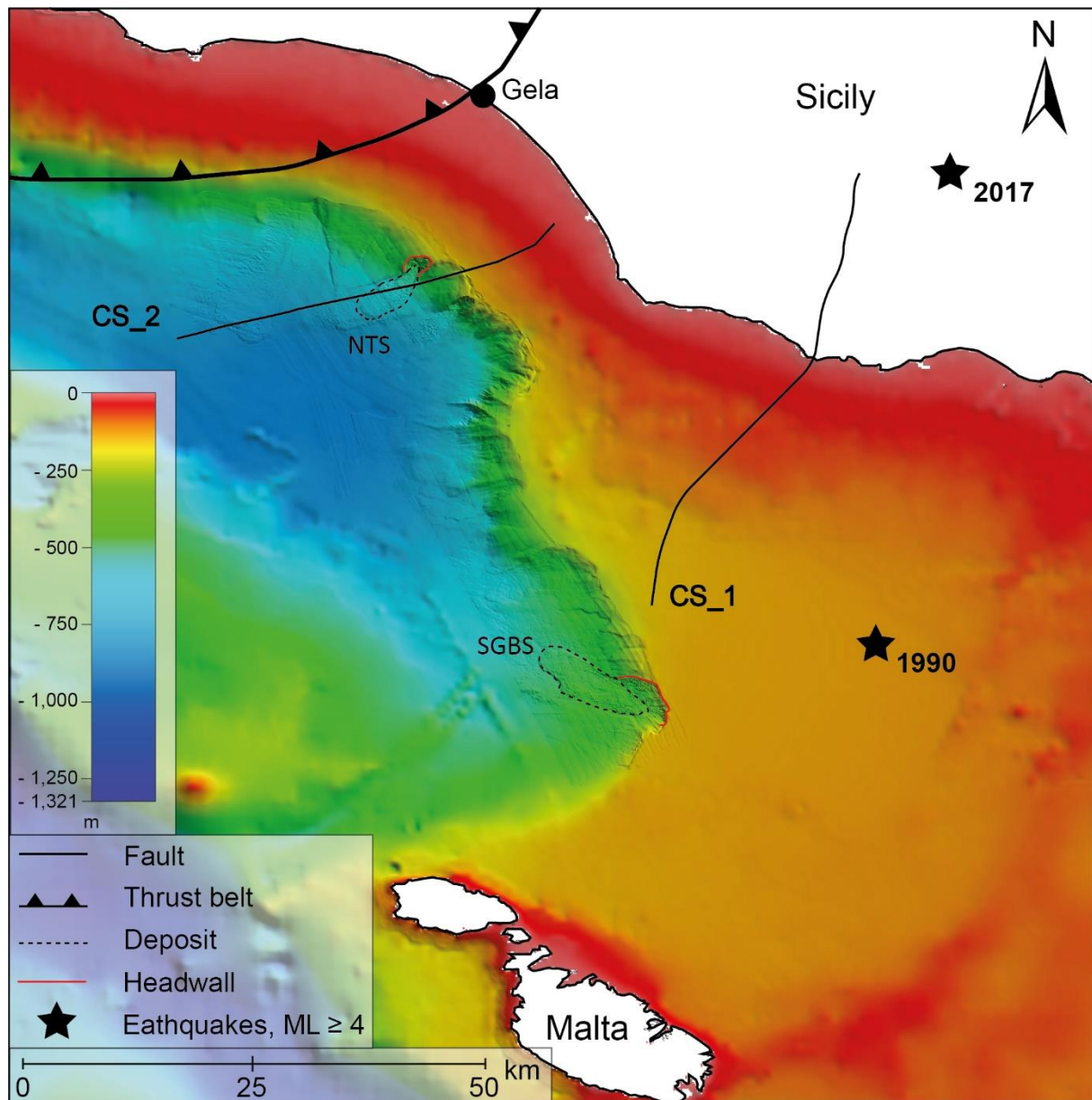
Figure 7.2: Bathymetric map showing the location of the North Twin Slide (NTS) and South Gela Basin Slide (SGBS) and the location of the recent seismic sequences registered near the Gela Basin as well as the positioning of the faults (CS_1 and CS_2) used in the stability analysis based on Antoncicchi et al. (2020). CS_01 represents the offshore continuation of the Scicli-Ragusa fault where a few NE-SW small fault segments until 8 km were identified in the near offshore area (Azzaro and Barbono, 2000). CS_2 is a normal fault offsetting the Meso-Cenozoic sedimentary succession until Top Messinian at the Gela Nappe front and possibly reactivated in compression.
