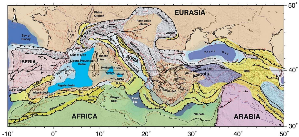
Figure 2.1: Present day location of the plate tectonic setting in the Mediterranean from Faccenna et al. (2014).
