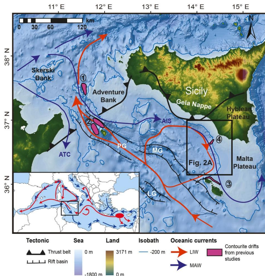
Fig. 1. Relief and bathymetric map of the Strait of Sicily; red and blue arrows represent the Levantine Intermediate Water (LIW) and the Modified Atlantic Water (MAW) (adapted from Lermusiaux and Robinson, 2001). 1–4 = previously studied contourite deposits: 1 = Marani et al. (1993), 2 = Martorelli et al. (2011), 3 = Micallef et al. (2013) and 4 = Verdicchio and Trincardi (2008). AIS = Atlantic Ionian Stream, ATC = Atlantic Tunisian Current, PG = Pantelleria Graben, MG = Malta Graben, LG = Linosa Graben. Inset: general oceanographic circulation in the Mediterranean Sea. (For interpretation of the references to colour in this figure legend, the reader is referred to the Web version of this article.)
