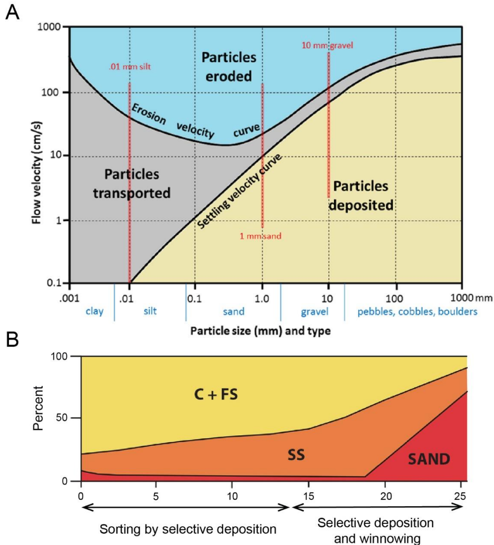
Figure 3.16: A) Hjulström-Sundborg diagram and B) sediment percentage-flow speed relationship modified from McCave and Hall (2006).
