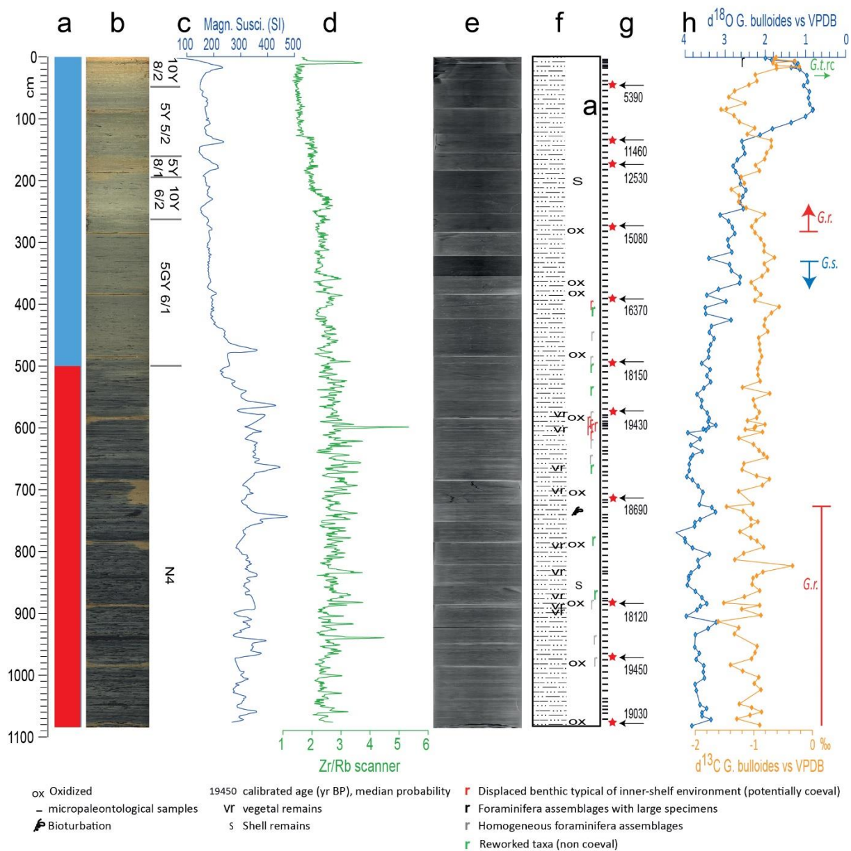
Figure 3.15: Data example of core MS72 with a) a representation of the amplitude reflectors crossed by the piston corer, b) a photograph of the core with the colour code, c) the magnetic susceptibility measured, d) an elemental ratio, e) the X-ray images and f) the foraminifera assemblages identified as well as the presence of other components (i.e. vegetal remains, oxidation, bioturbation, shell remains, etc.), and g) the position of the radiocarbon dating and h) the stable isotopes analysed.
