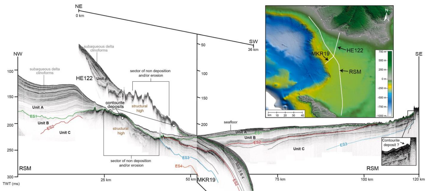
Fig. 8. SBS profile “RSM” which shows the younger clinothem (units A and B) crossed by SBS profiles “HE122” and “MKR19” (NE–SW direction) to highlight the changes in clinothem thickness along the shelf and the overall along-strike variability of the margin.
