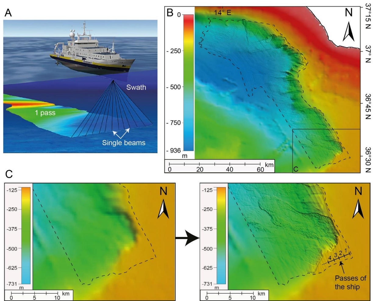
Figure 3.7: A) Representation of how a multibeam echosounder system acquires high-resolution bathymetric data (Ifremer, 2020). B) Bathymetric map showing the surface mapped with the multibeam echosounder along the eastern Gela Basin (surrounded by a black dotted line). C) Bathymetric maps demonstrating the increase in resolution of the bathymetry with the use of a multibeam echosounder. Note that each parallel lines observed on the high-resolution bathymetry (NW-SE) represent a pass of the ship during the acquisition with the swath echosounder.
