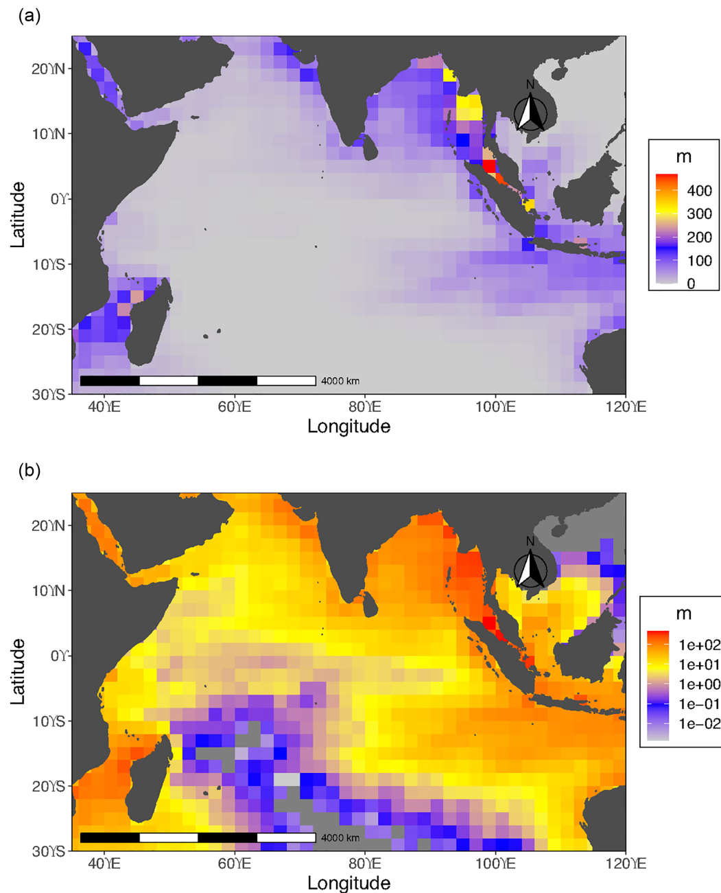
Figure 6. Putative spatial distribution of NLOGs obtained from simulated trajectories for the IO, in 2014. The mean number of simulated NLOG per cell is shown (m), aggregated over a transport time of 180 days, using forcing currents produced by NEMO at surface. Linear color scale (a) and log transformed color scale (b).
