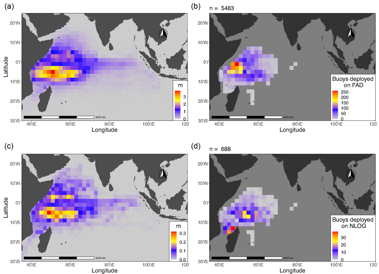
Figure 5. Spatial distribution of instrumented FOBs, from 2014 to 2018. Mean number of buoys associated with an object per day per cell (m), obtained from the GPS buoy trajectories dataset, for FADs (a) and NLOGs (c). Number of buoys deployment per cell, obtained from the observers' dataset, on FADs (b) and on NLOGs (d); n: total number of deployments. Dark grey: less than 10 days of observation per cell.
