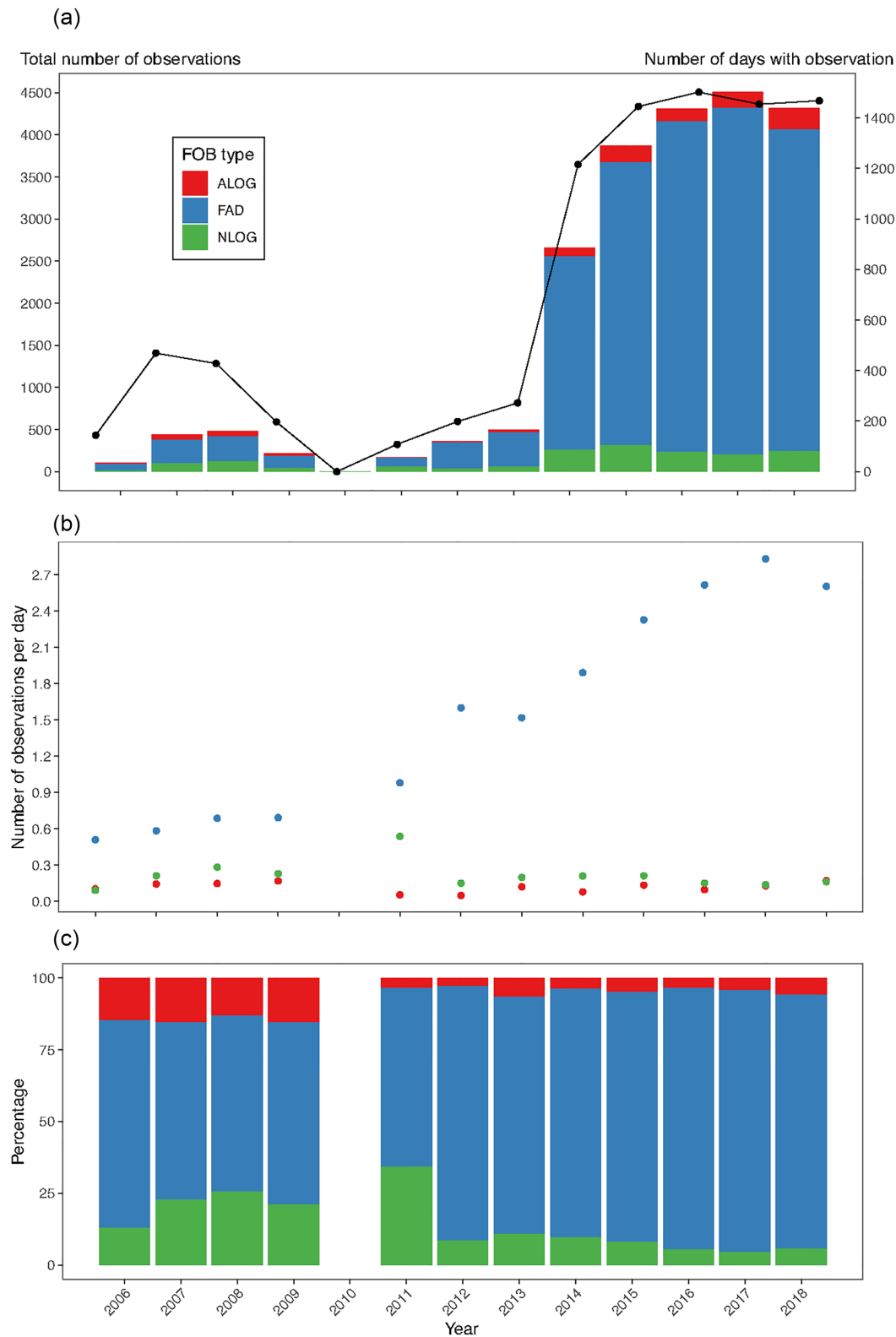
Figure 1. Change in the number of FOBs observed from 2006 to 2018 in the IO. (a) Number of FOBs observed over time, by FOB type, and number of days with observations per year (black line). (b) Number of observed FOBs, by FOB type, divided by the number of days of observation. (c) Proportion of each FOB type per year. FAD (in blue): fish aggregating device; NLOG (in green): natural floating object; ALOG (in red): artificial log resulting from human activity (other than FADs).
