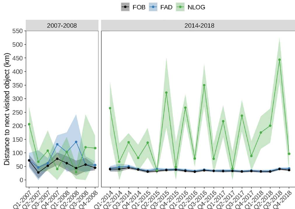
Figure 2. Quarterly median spatial distance between two consecutive encounters of FOBs for the two study periods (2007–2008 and 2014–2018). The distance was calculated between two consecutive encounters of any type of FOBs (FAD, ALOG, or NLOG; black line), between encounters of FADs only (blue line) and between encounters of NLOGs only (green line). The colored areas around the lines represent the SE.
