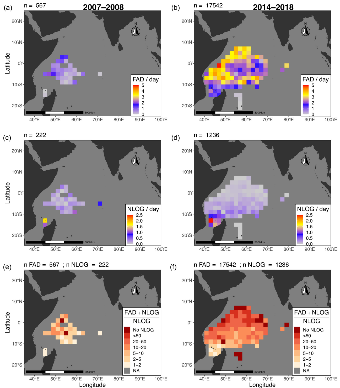
Figure 4. Spatial distribution of FOBs observed in the western IO for the two periods (2007–2008 and 2014–2018). (a–b) Number of FAD observations divided by the number of days of observations. (c–d) Number of NLOG observations divided by the number of days of observations. (e–f) multiplication factor (ratio of FADs + NLOGs over NLOGs). Dark grey: less than 10 days of observation per cell.
