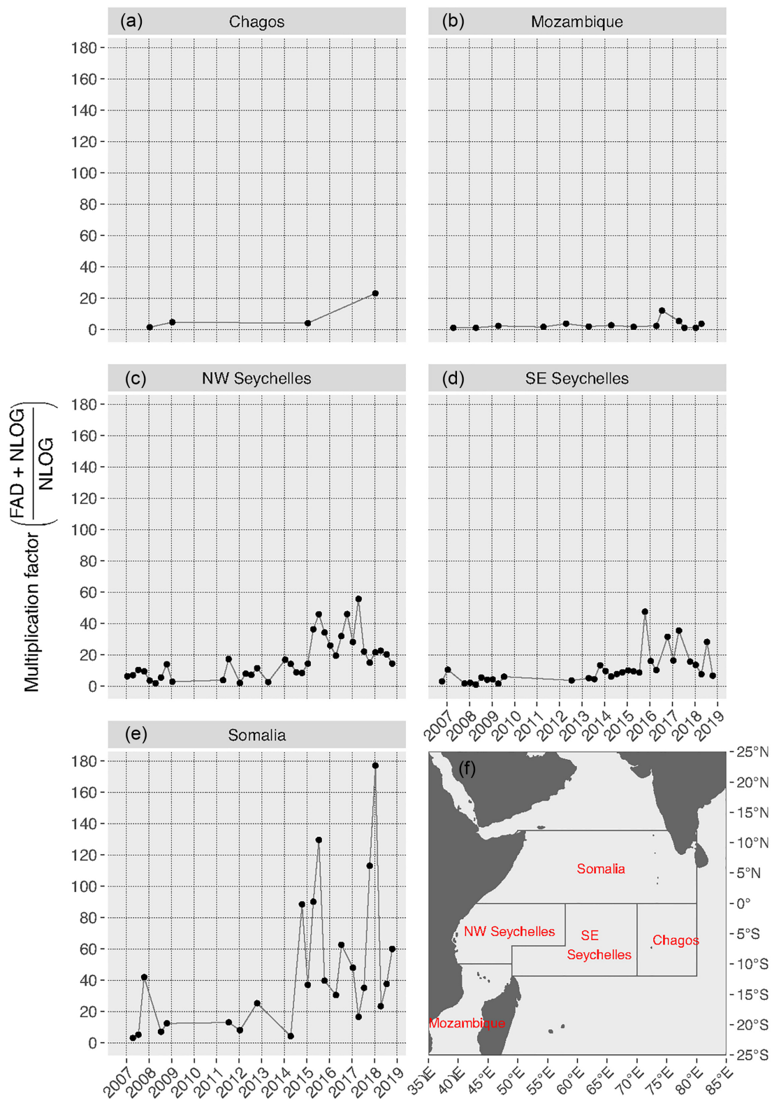
Figure 3. Quarterly multiplication factor in the different IOTC areas from 2007 to 2018: in Chagos (a), Mozambique Channel (b), North-West Seychelles (c), South-East Seychelles (d), and Somalia (e). Map of the IOTC areas as defined in Dagorn et al. (2013a) (f). The multiplication factor was calculated only for the quarters with observations of both NLOGs and FADs.
