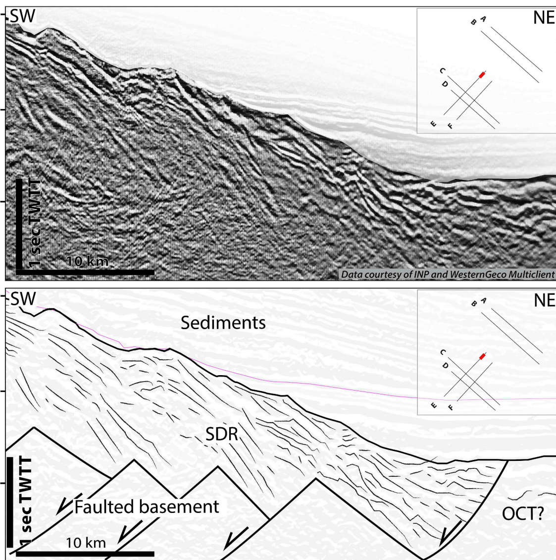
Fig. 13. Profile E – Structural interpretation of the northeast of the Beira High showing SDR formed by volcanic or volcanoclastic material deposited over a faulted crystalline basement. This indicates that this region of the Beira High experienced an extension, likely associated with the rifting episode. The SDR are reasonably well expressed, however extension appears to be attenuated when compared to the structures observed along the southern Beira High margin. OCT: Ocean Continent Transition.
