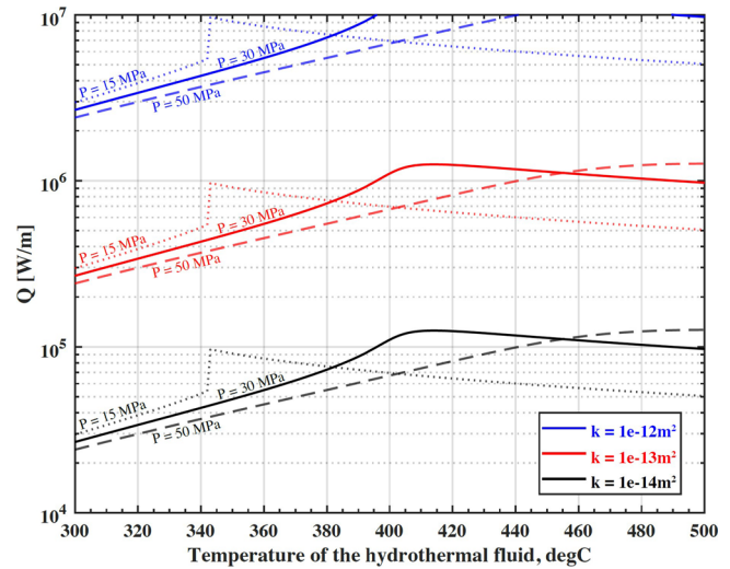
Fig. 6 Heat transported advectively by a hydrothermal fluid of temperature T_f for a given permeability k (line colors). Lines were computed from the Eq. (1) (i.e., Eq. (6) of Driesner 67 ), using a width for the hydrothermal plume ( L_D ) of 50 m and for fluid properties at 15, 30, and 50 Mpa shown as dotted lines, solid lines and dashed lines, respectively.
