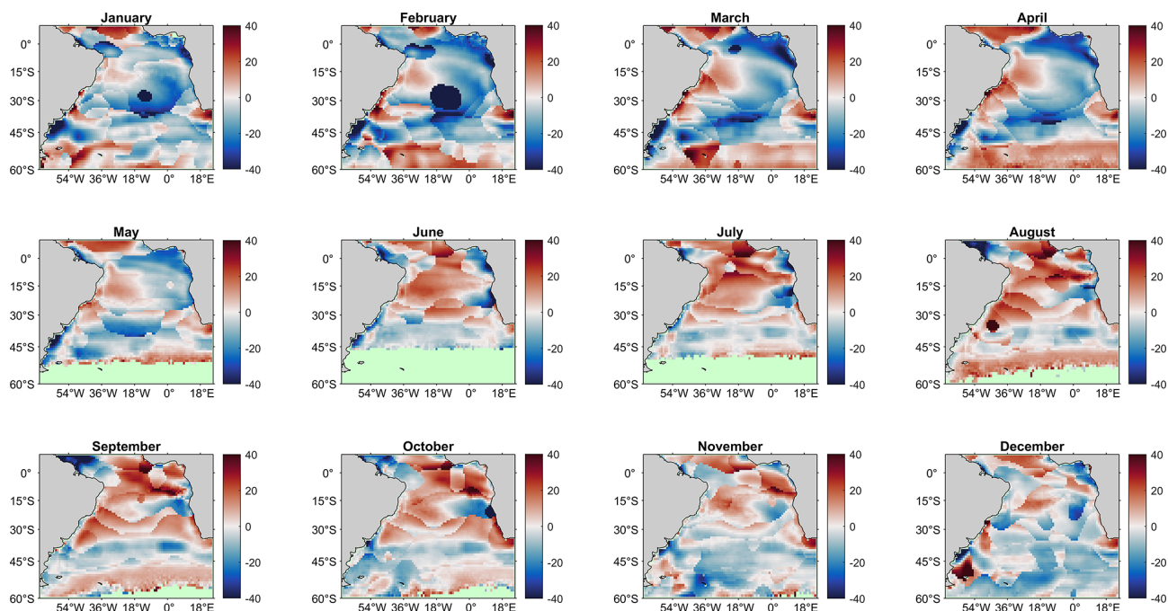
Figure B3. Monthly comparison between p\text{CO}_2(\text{sw}) climatologies estimated by the SA-FNN NCP and W2020 (Watson et al., 2020a) climatology referenced to 2010 (SA-FNN NCP p\text{CO}_2 - \text{W2020 } p\text{CO}_2 ). Red (Blue) shades indicate regions where SA-FNN NCP is greater (less) than the W2020 climatology.
