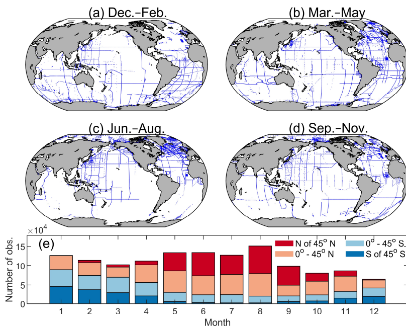
680 Figure 9. Distribution of data in GLODAPv2.2021 in (a) December–February, (b) March–May, (c) June–August, (d) September–November, and (e) number of observations for each month in four latitude bands.
