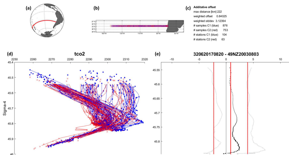
315 Figure 3. Example crossover figure, for TCO 2 for cruises 320620170820 (blue) and 49NZ20030803 (red), as it was generated during the crossover analysis. Panel (a) shows all station positions for the two cruises and (b) shows the specific stations used for the crossover analysis. Panel (d) shows the data of TCO 2 (μmol kg -1 ) below the upper depth limit (in this case 2000 dbar) versus potential density anomaly referenced to 4000 dbar, as points and the interpolated profiles as lines. Non-interpolated data either did not meet 320 minimum depth separation requirements (Table 4 in Key et al., 2010) or are the deepest sampling depth. The interpolation does not extrapolate. Panel (e) shows the mean TCO 2 (μmol kg -1 ) difference profile (black, dots) with its standard deviation, and also the weighted mean offset (straight, red) and weighted standard deviation. Summary statistics are provided in (c).
