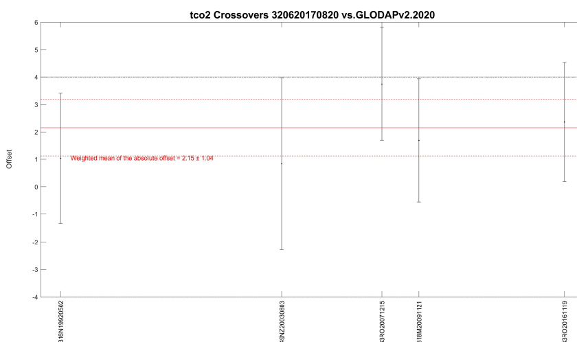
325 Figure 4. Example summary figure, for TCO 2 crossovers for 320620170820 versus the cruises in GLODAPv2.2020 (with cruise EXPOCODE listed on x-axis sorted according to year the cruise was conducted). The black dots and vertical error bars show the weighted mean offset and standard deviation for each crossover (in μmol kg -1 ). The weighted mean and standard deviation of all these offsets are shown in the red lines and are 2.15 \pm 1.04 μmol kg -1 . The black dashed line is the reference line for a +4 μmol kg -1 offset (the corresponding line for -4 μmol kg -1 offset is right on top of x-axis and not visible).
