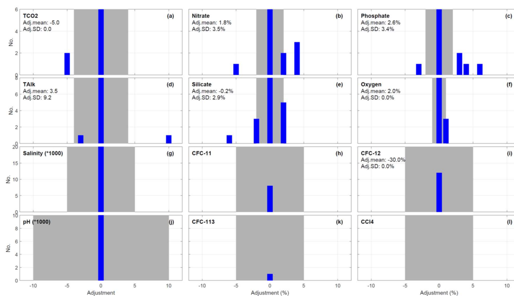
560 Figure 6. Distribution of applied adjustments for each core variable that received secondary QC, in \mu\text{mol kg}^{-1} for TCO 2 and TALK, unitless for salinity and pH (but multiplied with 1000 in both cases so a common x-axis can be used), while for the other properties adjustments are given in percent ((adjustment ratio-1)x100). Grey areas depict the initial minimum adjustment limits. The figure includes numbers for data subjected to secondary quality control only. Note also that the y-axis scale is set to render the number of adjustments to be visible, so the bar showing zero offset (the 0 bar) for each variable is cut off (see Table 6 for these numbers).
