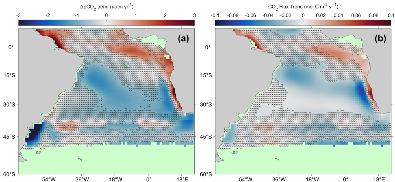
Figure 5. Linear trends in (a) \Delta p\text{CO}_2 and (b) the air–sea CO 2 flux between 2002 and 2018. Hashed areas indicate non-significant trends when accounting for the uncertainties. Green regions indicate insufficient data to calculate trends.
