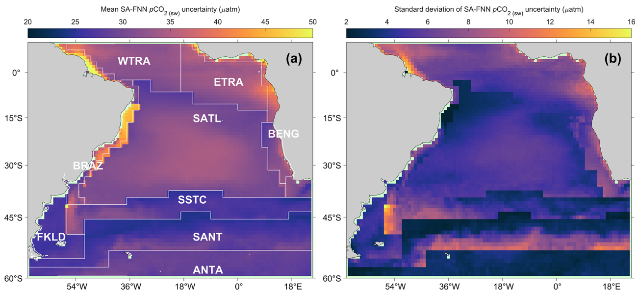
Figure B1. (a) Mean SA-FNN p\text{CO}_2 (sw) uncertainty between July 2002 and December 2018. Longhurst provinces (Longhurst, 1998) used within the SA-FNN training described in Ford et al. (2022; note the WTRA and ETRA are merged into one province). The province area acronyms are listed as follows: WTRA is western tropical Atlantic, ETRA is eastern equatorial Atlantic, SATL is South Atlantic gyre, BRAZ is the coastal Brazilian Current, BENG is Benguela Current coastal upwelling, FKLD is southwest Atlantic shelves, SSTC is South Subtropical Convergence, SANT is sub-Antarctic, and ANTA is Antarctic. (b) Standard deviation of SA-FNN p\text{CO}_2 (sw) uncertainty.
