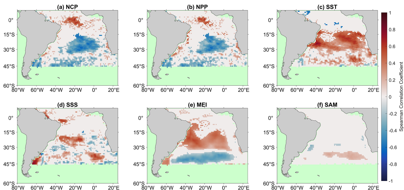
Figure 4. Significant Spearman correlations between the air–sea CO 2 flux inter-annual component of the X-11 analysis and (a) net community production (NCP), (b) net primary production (NPP), (c) sea surface temperature (SST), (d) sea surface salinity (SSS), (e) multivariate ENSO index (MEI), and (f) Southern Annular Mode (SAM) inter-annual components. White regions indicate no significant correlations, and green regions indicate no analysis was performed due to missing satellite data.
