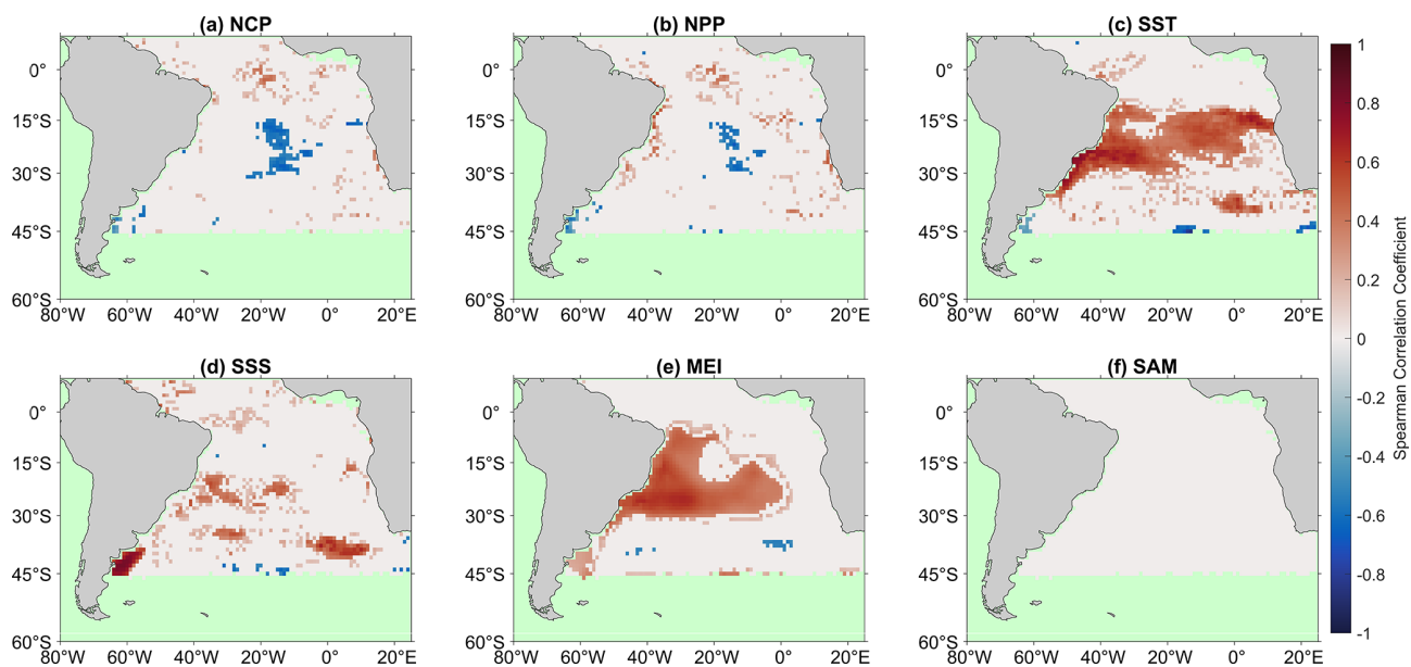
Figure 3. Significant Spearman correlations between the \Delta p\text{CO}_2 inter-annual component of the X-11 analysis and (a) net community production (NCP), (b) net primary production (NPP), (c) sea surface temperature (SST), (d) sea surface salinity (SSS), (e) multivariate ENSO index (MEI), and (f) Southern Annular Mode (SAM) inter-annual components. White regions indicate no significant correlations, and green regions indicate no analysis was performed due to missing satellite data.
