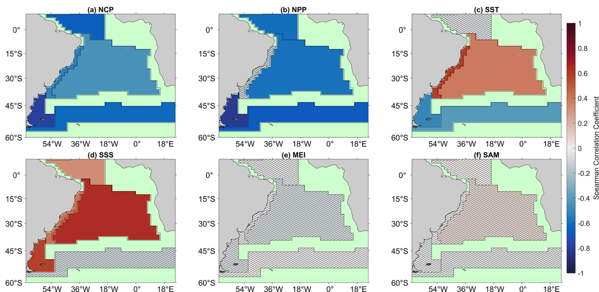
Figure A1. Spearman correlations between the in situ \Delta p\text{CO}_2 seasonal component of the X-11 analysis and (a) net community production (NCP), (b) net primary production (NPP), (c) sea surface temperature (SST), (d) sea surface salinity (SSS), (e) multivariate ENSO index (MEI), and (f) Southern Annular Mode (SAM) seasonal components on a per province basis. Hashed areas indicate no significant correlations, and green regions indicate no analysis was performed due to missing data.
