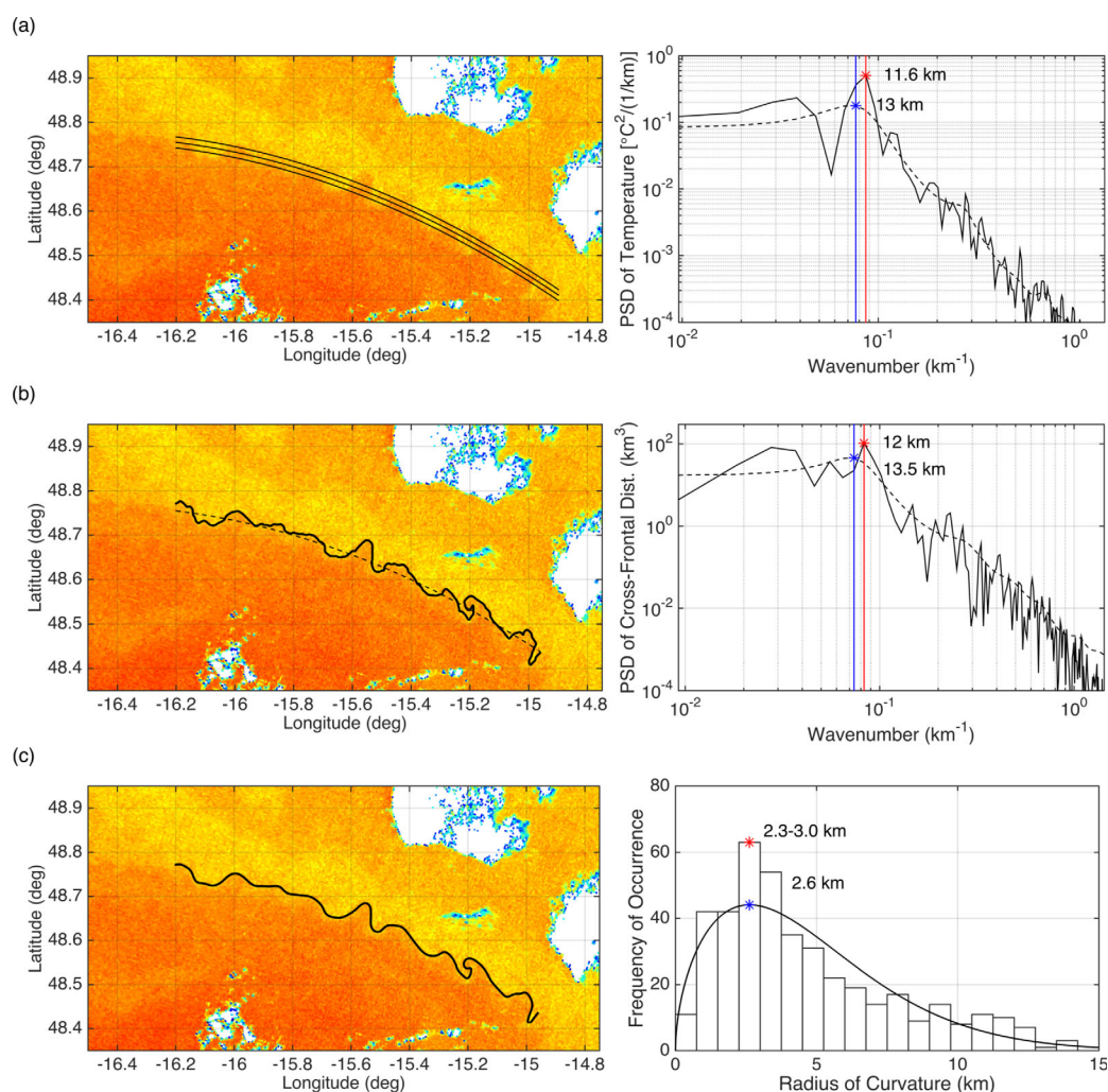
Figure A1. Methods used to estimate observed eddy diameters. In Figures A1a and A1b, we illustrate spectra computed using both traditional (solid) and parametric (dashed) spectral approaches. Asterisks highlight wavelengths corresponding to peaks in the spectral energy. In Figure A1c, we estimated the radius of curvature, R=|1/\kappa| , of the frontal boundary, where the boundary was smoothed slightly to improve estimates of curvature. Asterisks highlight the (red) most frequently occurring and (blue) probable radii given a Weibull fit to the data. Eddy diameters were estimated as (a, b) half the peak wavelength and (c) twice the most probable radius of curvature.
