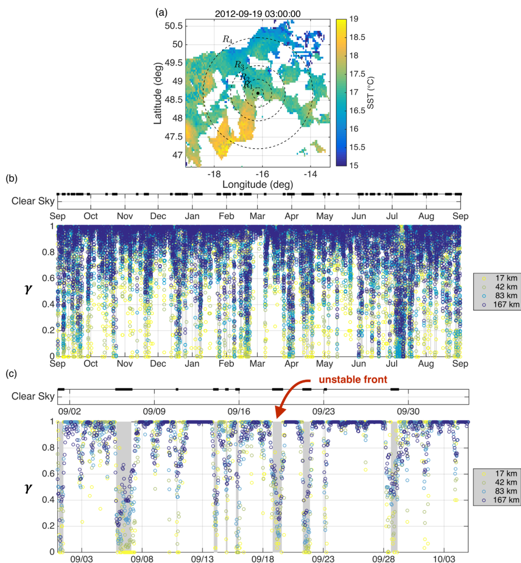
Figure 2. Identification of clear-sky occurrences over the OSMOSIS site (48.69°N, 16.19°W): (a) SST from SEVIRI on MSG-3 valid at the time of the unstable front. Fractional cloud cover, \gamma , was computed as the fraction of cloud-contaminated pixels within circles of increasing distance from the observation center. (b) Clear-sky occurrences and \gamma at the OSMOSIS mooring site (2012–2013). (c) Same as Figure 2b but magnified on 1 September to 5 October 2012; clear-sky occurrences are shown in gray and the red arrow highlights the period during which an unstable front was observed (the focus of this study). Colors correspond to radii of small circles, R_1 to R_4 .
