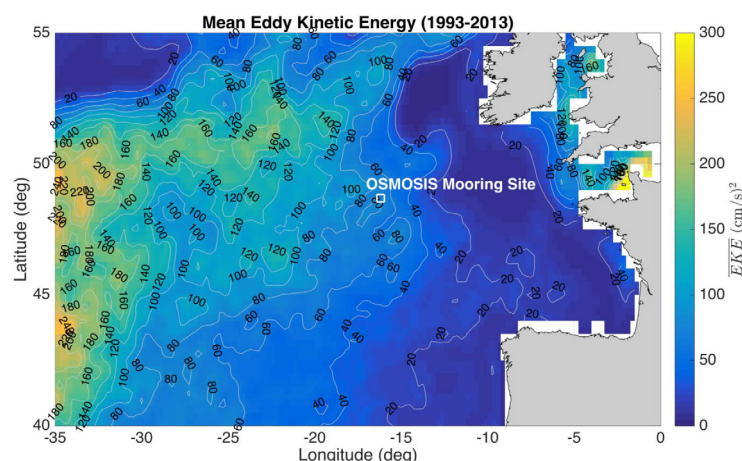
Figure 1. The location of the OSMOSIS mooring site (48.69°N, 16.19°W, September 2012 to September 2013) overlain on mean eddy kinetic energy (EKE). Signatures of the Gulf Stream's extension into the Atlantic is seen to the west while a more latent eastern boundary current is and continental shelf waters are found to the east. Mean EKE was computed from satellite altimetry (1993–2013).
