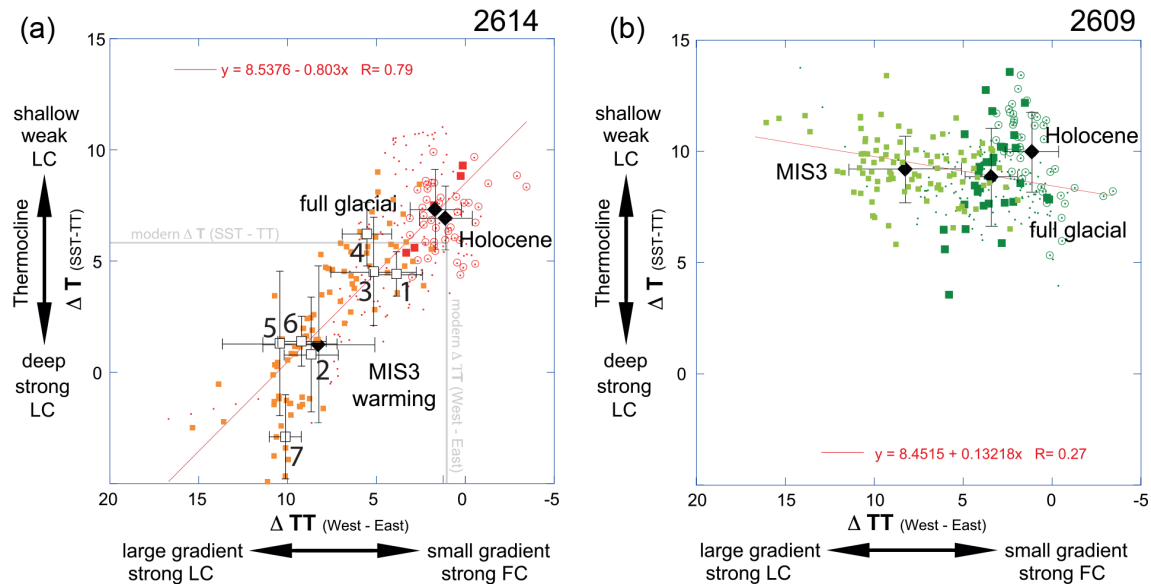
Figure 7. Vertical temperature versus lateral thermocline temperature gradient as expression of Leeuwin Current System variability. The vertical temperature gradient ( \Delta T_{\text{SST-TT}} ; in ^{\circ}\text{C} ) provides insight into the thermocline depth, with low (high) \Delta T_{\text{SST-TT}} pointing to a deep (shallow) thermocline. The lateral gradient at thermocline depth ( \Delta \text{TT}_{\text{west-east}} ; in ^{\circ}\text{C} ) defines how the Leeuwin Current developed in relation to the Flinders Current. (a) Western core 2614 showing a well-defined relationship between \Delta T_{\text{SST-TT}} and \Delta \text{TT}_{\text{west-east}} ( R = 0.8 ). Prominent MIS3 thermocline warming periods (orange symbols; white squares are averages, numbered from 7 to 1) point to a strong Leeuwin Current, which weakened across MIS3 (black diamonds show averages) approaching LGM (red squares) and Holocene conditions (red circles; black diamonds show averages). (b) Eastern core 2609 lacks a relationship between \Delta T_{\text{SST-TT}} and \Delta \text{TT}_{\text{west-east}} , implying that the Leeuwin Current is not affecting this study site over time.
