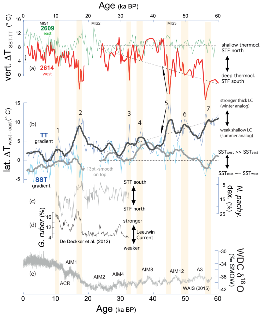
Figure 6. Variability of lateral and vertical temperature gradients south of Australia in comparison to other proxy records over the last 60 kyr. (a) Vertical temperature gradients ( \Delta T_{\text{SST-TT}} ) between sea surface and thermocline reflecting thermocline changes in the western (red) and eastern (green) study areas in line with migrations of the STF. The small double arrow along the y axis marks the modern vertical gradient (30–350 m) in the west (Locarnini et al., 2019). (b) Lateral (west–east) 13-point smoothed temperature gradients at the sea surface (grey) and at thermocline depth (black) reflecting Leeuwin Current strength, underlain by the raw data (equally sampled at 0.2 kyr spacings using AnalySeries 2.0; Paillard et al., 1996). Stippled lines in (a) and (b) indicate long-term trends. (c) N. pachyderma dextral and (d) G. ruber percentages of core MD03-2611 from De Deckker et al. (2012) reflecting lateral migrations of the STF and changes in Leeuwin Current strength, respectively. (e) West Antarctic Ice Sheet Divide Core \delta^{18}\text{O} record (WAIS Divide Project Members, 2015) as a reference for the Southern Hemisphere climate signal. Orange shading shows short time periods of a strong Leeuwin Current. A3 is the Antarctic warming event. AIM stands for Antarctic Isotope Maxima. MIS stands for Marine Isotope Stages 1–3 (Martinson et al., 1987). ACR stands for Antarctic Cold Reversal.
