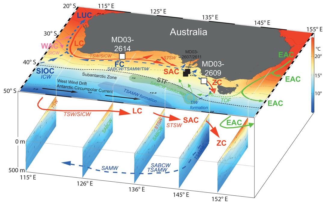
Figure 1. The top of this image shows the regional surface and subsurface circulation pattern off southern Australia underlain by the modern annual SST pattern (using Ocean Data View v. 5.1.7; Schlitzer, 2019; World Ocean Atlas, Locarnini et al., 2019). Sediment core locations (MD03-2614 and -2609) studied here are marked by white squares. Black squares are reference sites. Surface currents are shown in red and green: LC is the Leeuwin Current, WAC is the West Australian Current, SIOC is the South Indian Ocean Current, SAC is the South Australian Current, ZC is the Zeehan Current, EAC is the East Australian Current, and TOF is the Tasman Outflow. Subsurface currents are shown in blue: FC is the Flinders Current, and LUC is the Leeuwin Undercurrent. Water masses transported by currents: TSW is Tropical Surface Water, ICW is Indian Central Water, SICW is South Indian Central Water, STSW is Subtropical Surface Water, SABCW is South Australian Basin Central Water, SAMW is Subantarctic Mode Water, TSAMW is Tasmanian Subantarctic Mode Water, and TIW is Tasmanian Intermediate Water. Sites of SABCW, TIW, and TSAMW formation are indicated. STF is the Subtropical Front (dashed black line). The bottom of the image shows the N–S-oriented temperature profiles (February) of the upper 500 m (dotted white lines; using Ocean Data View v. 5.1.7; Schlitzer, 2019). Currents, water masses, and sites of mode and intermediate water formation are from Richardson et al. (2019).
