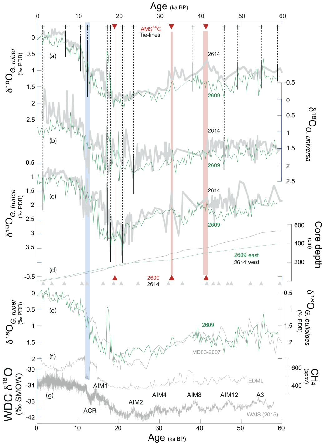
Figure 3. Chronostratigraphy of the eastern core 2609 (King Island). The age model is based on the tuning of various planktonic \delta^{18}\text{O} records of (a) G. ruber , (b) O. universa , and (c) G. truncatulinoides (all in green lines) to similar records (thick grey lines) of the well-dated reference core 2614 (van der Kaars et al., 2017). In total, 13 tuning tie lines (stippled lines; solid for the species-specific correlations) were set in order to achieve an optimal fit of the core 2609 and core 2614 \delta^{18}\text{O} records (mean r^2 = 0.86 ). The age model for core 2609 is supported by three AMS ^{14}\text{C} datings (red triangles and red lines; red shading marks the 1-sigma errors). (d) Sedimentation rates (green = core 2609; grey = core 2614). Grey triangles are age control points established for core 2614 by van der Kaars et al. (2017). (e) The age model for core 2609 is supported by the match of its \delta^{18}\text{O}_{G. ruber} record (green) to the adjacent core MD03-2607 \delta^{18}\text{O}_{G. bulloides} record (grey; Lopes dos Santos et al., 2013). (f) Atmospheric \text{CH}_4 record from EPICA ice core (EPICA Community Members, 2006). Blue shading denotes prominent atmospheric \text{CH}_4 anomaly synchronous to a distinct reflection in the core 2614 \delta^{18}\text{O}_{O. universa} record. (g) West Antarctic Ice Sheet Divide Core \delta^{18}\text{O} record (WAIS Divide Project Members, 2015) as reference for the Southern Hemisphere climate signal.
