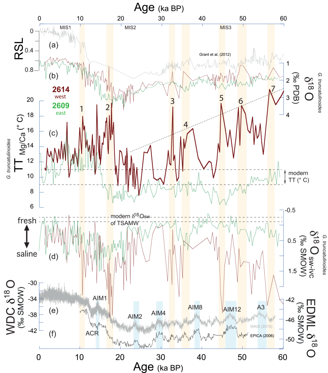
Figure 5. Hydrographic development at thermocline depth over the last 60 kyr. Colored curves represent this study, while grey and black curves represent reference records. (a) Relative sea level curve of Grant et al. (2012) (in ‰). (b) Thermocline \delta^{18}\text{O}_{G. truncatulinoides} records at the western (brown; core 2614) and the eastern (green; core 2609) core locations. (c) \text{TT}_{\text{Mg/Ca}} records derived from G. truncatulinoides (brown: core 2614; green: core 2609). (d) Thermocline salinity approximations ( \delta^{18}\text{O}_{\text{sw-ivc}} ) at the western (brown) and eastern (green) core locations. (e) West Antarctic Ice Sheet Divide Core (grey; WAIS Divide Project Members, 2015) and (f) EDML (black; EPICA Community Members, 2006) \delta^{18}\text{O} records as reference for the Southern Hemisphere climate signal. Blue shading shows the Antarctic Isotope Maxima (AIM). Red shading shows the prominent thermocline warming pulses and changes to high salinities at thermocline depth (black numbers). Dashed lines are the modern annual TT range at 50–100 m water depth (Locarnini et al., 2019) and modern \delta^{18}\text{O}_{\text{sw}} range of TSAMW (Richardson et al., 2019). MIS stands for Marine Isotope Stages 1–3 (Martinson et al., 1987). ACR stands for Antarctic Cold Reversal.
