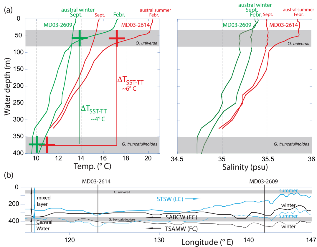
Figure 2. Upper ocean hydrological setting south of Australia: (a) temperature (left) and salinity (right) distribution in the upper 400 m at the western core 2614 location (red) and at the eastern core 2609 location (green; cf. Fig. 1). Only maximum (February; austral summer) and minimum (September; austral winter/spring) temperatures and salinities are indicated. Presumed calcification depths of foraminiferal species analyzed are indicated by grey shading: O. universa at \sim 30 – 80 m water depth (Anand et al., 2003; Farmer et al., 2007) and G. truncatulinoides at \sim 350 – 400 m water depth (Cl  roux et al., 2008; Anand et al., 2003). Modern average temperatures (crosses) and temperature gradients between surface and thermocline are indicated for the respective study areas. Data from Ocean Data View v. 5.1.7 (ODV Station labels 12796 and 11161; Schlitzer, 2019; WOA; Locarnini et al., 2019). (b) Average summer (blue) and winter (black) boundaries between the surface mixed layer (consisting predominantly of STSW, transported eastward by the Leeuwin Current, LC) and the Central Water (composed of SABCW and TSAMW, transported westward by the Flinders Current, FC), taken from Richardson et al., 2019). Core locations (vertical black lines) and assumed calcification depths of foraminiferal species studied are indicated.
