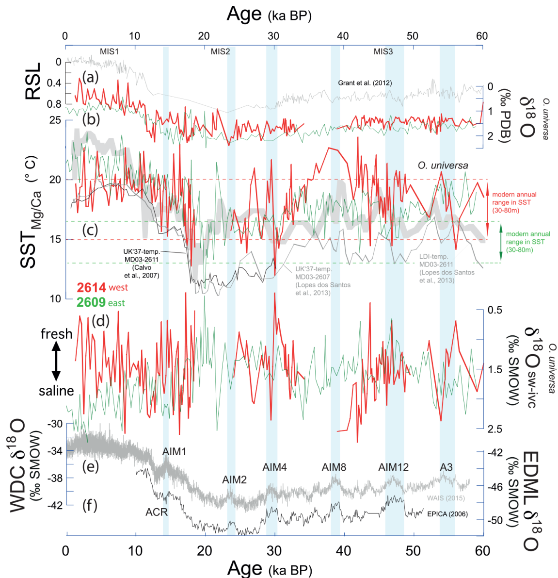
Figure 4. Hydrographic development at sea surface over the last 60 kyr. Colored curves represent this study, while grey and black curves represent reference records. (a) Relative sea level curve of Grant et al. (2012) (in ‰). (b) Sea surface \delta^{18}\text{O}_{O. universa} records at the western (red; core 2614) and the eastern (green; core 2609) core locations. (c) \text{SST}_{\text{Mg/Ca}} records derived from O. universa (red; core 2614; green: core 2609). The long-chain diol-based \text{SST}_{\text{LDI}} (thick grey) and alkenone-based \text{SST}_{\text{UK'37}} records (thin grey and black) of nearby cores MD03-2607 and MD03-2611 (Calvo et al., 2007; Lopes dos Santos et al., 2013) are for comparison. (d) Relative sea surface salinity approximations ( \delta^{18}\text{O}_{\text{sw-ivc}} ) at the western (red) and eastern (green) core locations. (e) West Antarctic Ice Sheet Divide Core (grey; WAIS Divide Project Members, 2015) and (f) the EDML (black; EPICA Community Members, 2006) \delta^{18}\text{O} records as reference for the Southern Hemisphere climate signal. Blue shading shows the Antarctic Isotope Maxima (AIM). Dashed red and green lines show the modern annual SST range at 50–100 m water depth at the eastern and western core locations 2609 and 2614, respectively (Locarnini et al., 2019). MIS stands for Marine Isotope Stages 1–3 (Martinson et al., 1987).
