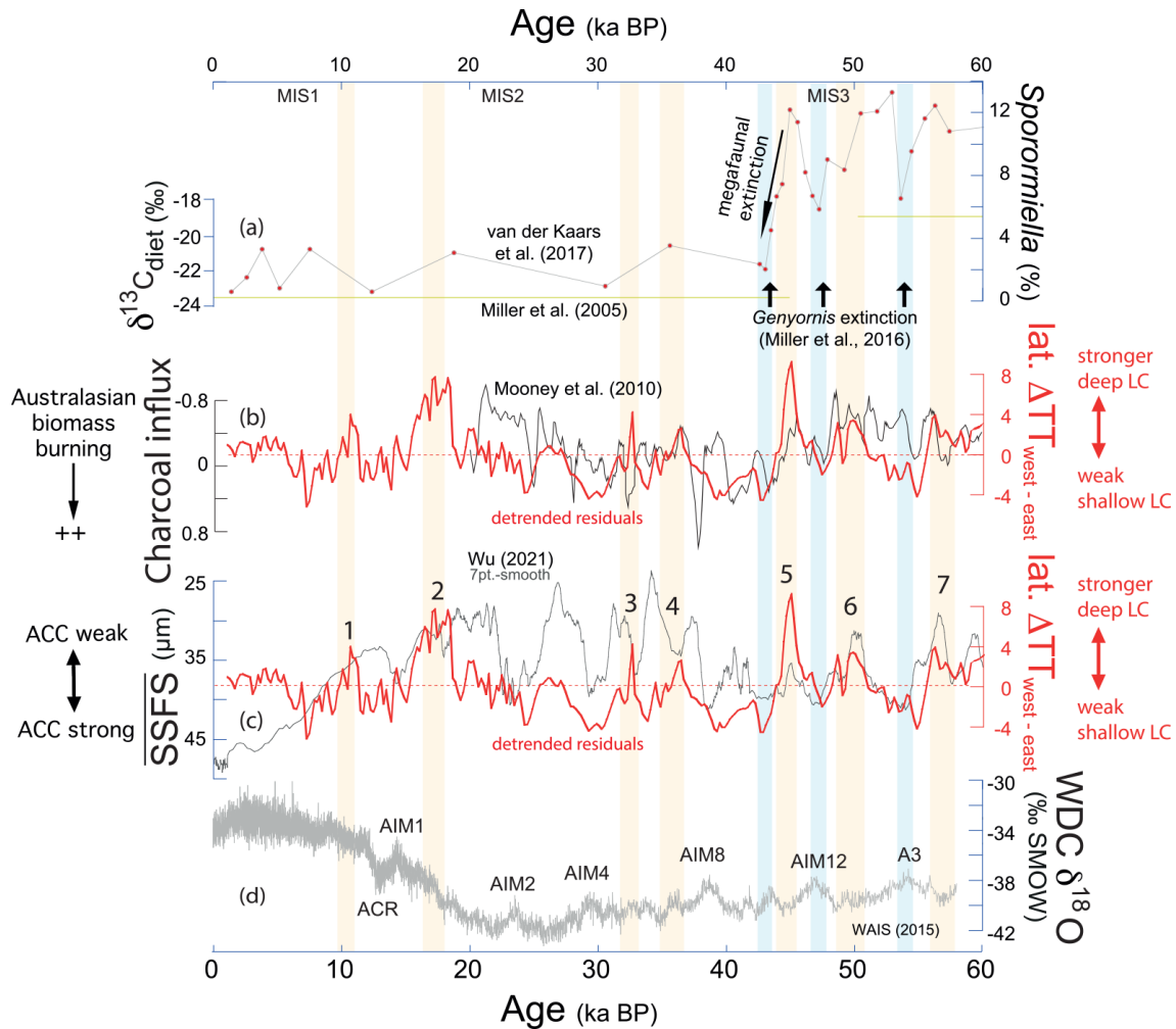
Figure 8. Variability of Leeuwin Current strength in comparison to Australian megafaunal extinction, biomass burning, and Antarctic Circumpolar Current (ACC) strength over the last 60 kyr. (a) Record of dung fungus Sporormiella percentages in western core 2614, pointing to the Australian megafaunal population collapse at \sim 45 to 43.1 ka BP (van der Kaars et al., 2017). The yellow lines depict the Australian emu Dromaius dietary \delta^{13}\text{C} change documenting a permanent change in food sources (Miller et al., 2005). The three black arrows indicate most probable extinction dates of the Australian megafaunal bird Genyornis newtoni at \sim 54 , \sim 47 , and \sim 43 ka BP (Miller et al., 2016). (b) Residuals of detrended lateral (west–east) temperature gradients at thermocline depth reflecting Leeuwin Current strength (red; detrended with Past4 software; https://www.nhm.uio.no/english/research/resources/past/ , last access: 10 November 2022), underlain by the Mooney et al. (2010) record of Australian biomass burning. (c) Residuals of detrended lateral (west–east) temperature gradients at thermocline depth reflecting Leeuwin Current strength (red), underlain by the sortable silt record (SSFS; 7 pt.-smooth) of Drake Passage sediment core PS97-85 reflecting the strength variability of the ACC (Wu et al., 2021). (d) West Antarctic Ice Sheet Divide Core \delta^{18}\text{O} record (WAIS Divide Project Members, 2015) as a reference for the Southern Hemisphere climate signal. Orange shading shows short time periods of a strong Leeuwin Current, mostly accompanied by less Australian biomass burning and ACC weakening. Blue shading shows an Antarctic warming event (A3) and Antarctic Isotope Maxima (AIM 12, 10). MIS stands for Marine Isotope Stages 1–3. ACR stands for Antarctic Cold Reversal.
