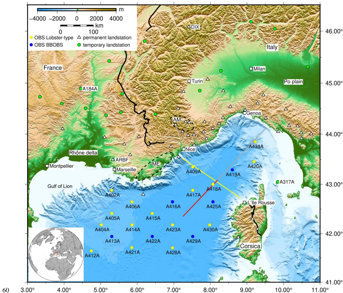
60 65 Figure 1: Map of the Ligurian Sea and adjacent Alpine region and the stations used for this study. OBS stations (network code: Z3) are shown as yellow (Lobster-type) and blue (BBOBS) circles. Permanent land stations (network codes: CH, FR, GU, IV, and MN) are shown as white triangles. Temporary land stations from AlpArray (network code: Z3) are shown as green circles. White squares represent cities. The black line represents the Alpine front (Schmid et al., 2004), AM marks the Argentera Massif, and ME marks the Maures-Esterel Massif. The inlay map in the bottom left shows the location of the research area (red box). The red, grey, and yellow lines show seismic refraction and reflection lines; red: Dannowski et al. (2020), grey: Makris et al. (1999), yellow: LISA01, Contrucci et al. (2001). The topography is plotted based on a GRMT grid (Ryan et al., 2009).
