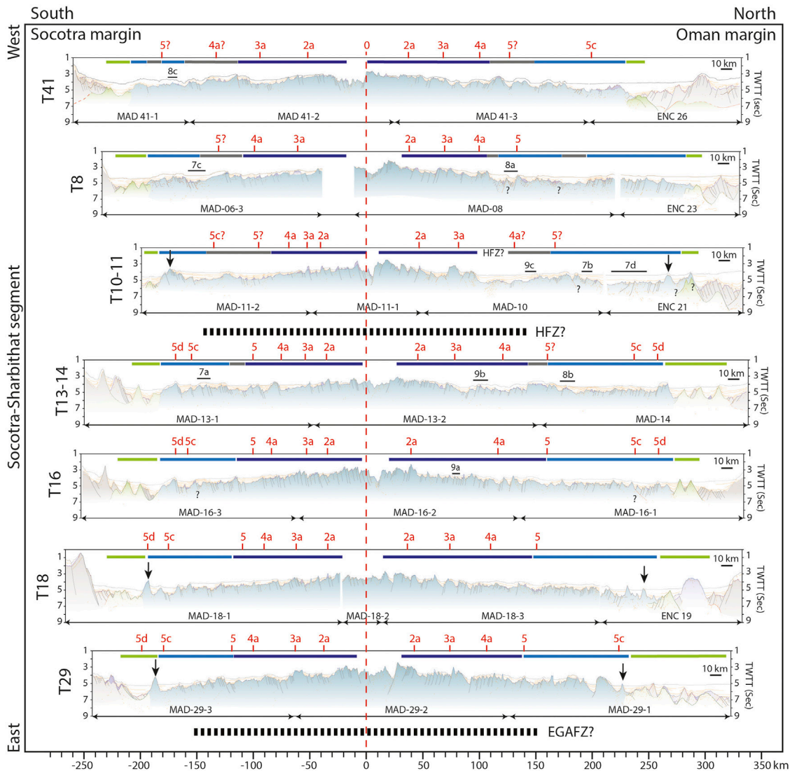
FIGURE 2 | Interpreted seismic transects along the Socotra-Sharbitah segment, in two-ways travel time (TWTT, seconds). Transects T21 and T27 are too noisy and not displayed. The transects are aligned on the magnetic anomaly 0 (ridge axis). The other interpreted magnetic anomalies are displayed in red. In green the OCT domain, in light blue the old oceanic domain (in grey the smooth and regular basement subdomain), in dark blue the young oceanic domain. Black arrays locate the basement ridge associated with the end of the OCT/first oceanic crust. Close up locations shown in Figures 6,7,8 are indicated by figure number on each transect. The dashed dark lines between transects represent the fracture zones (HFZ: Hadibo Fracture Zone, EGAFZ: Eastern Gulf of Aden Fracture Zone).
