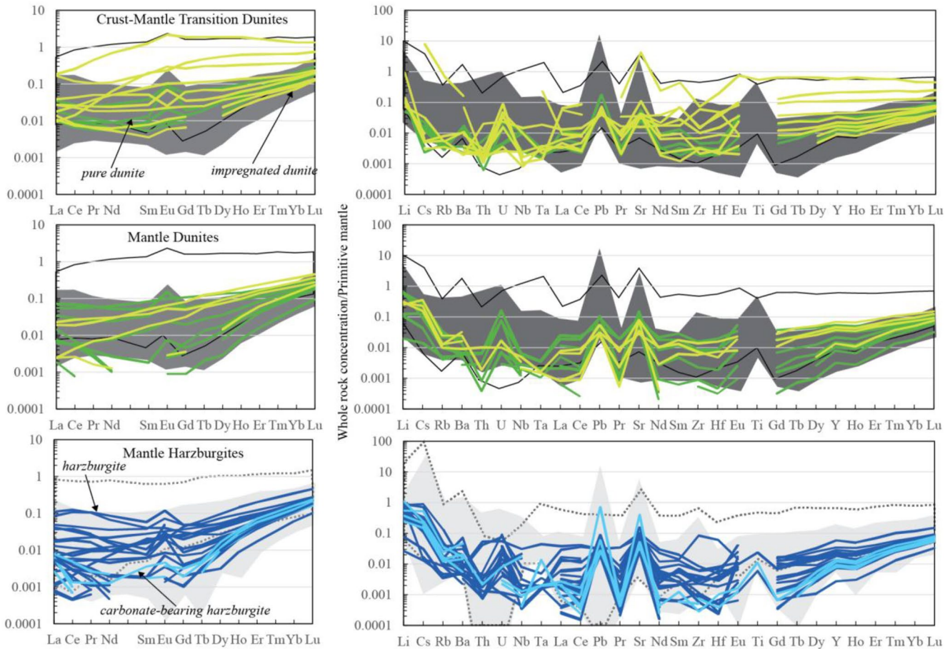
Figure 7b. Chondrite-normalized REE and Primitive Mantle (PM)-normalized multi-element patterns of pure dunites, impregnated dunites, harzburgites and carbonate-bearing harzburgites from the crust-mantle transition zone and mantle sections recovered at Hole CM2B. Other pure dunites (dark gray field formed) and impregnated dunites (field formed by black line) from the crust-mantle transition, and harzburgites (light gray field) and lherzolites (field formed by dashed line) patterns from the mantle section of the whole Oman ophiolite are reported for comparison (Gerbert-Gaillard, 2002; Girardeau et al., 2002; Godard et al., 2000; Hanghøj et al., 2010; Khedr et al., 2014; Lippard et al., 1986; Monnier et al., 2006; Nicolle et al., 2016; Rospabé, Benoit, & Candaup, 2018; Rospabé, Benoit et al., 2019; Takazawa et al., 2003). Normalizing chondrite and PM values are from Barrat et al. (2012) and Sun and McDonough (1989) respectively.
