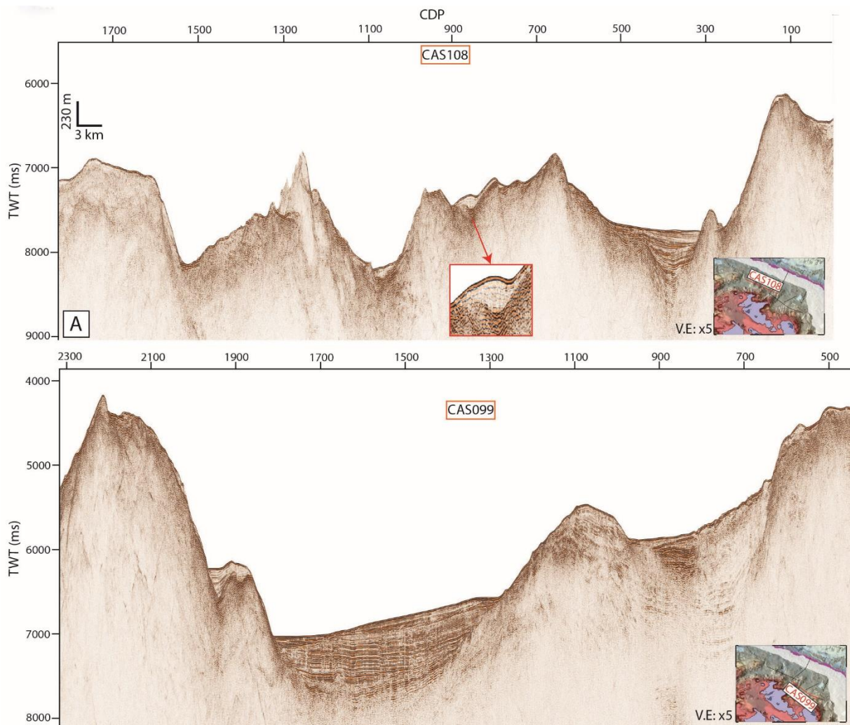
Figure 1S: Uninterpreted seismic profiles: A) CAS108. B) CAS099. The vertical exaggeration (V.E) is x5 for the two seismic profiles.
